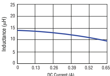
SRN3010TA-150M
