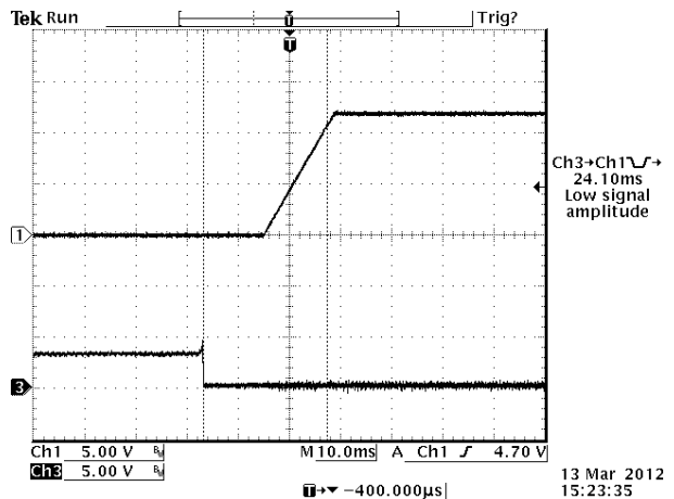
Figure 13. Startup from on/off Ch1: V_o Ch3: on/off V_{out} = 12\text{ V} / 20\text{ A} at V_{in} = 48\text{ V} @ T_a = 25^\circ\text{C} C_{ext} = 6800\text{ }\mu\text{F}
