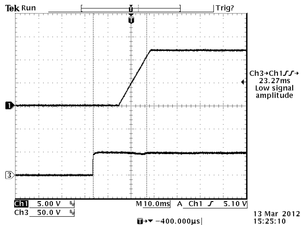
Figure 12. Startup from V_{in} Ch1: V_o Ch3: V_{in} V_{out} = 12\text{ V} / 20\text{ A} at V_{in} = 48\text{ V} @ T_a = 25^\circ\text{C} C_{ext} = 6800\text{ }\mu\text{F}
