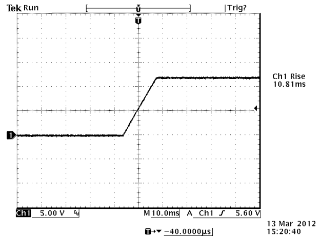
Figure 14. V_{out} = 12\text{ V} / 20\text{ A} at V_{in} = 48\text{ V} @ T_a = 25^\circ\text{C} , C_{ext} = 6800\text{ }\mu\text{F}
