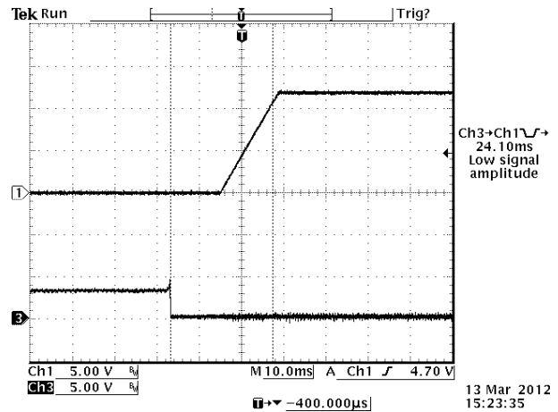
Figure 16. Startup from on/off Ch1: V_o Ch3: on/off V_{out} = 12\text{ V} / 20\text{ A} at V_{in} = 48\text{ V} @ T_a = 25^\circ\text{C} , C_{ext} = 6800\text{ }\mu\text{F}
