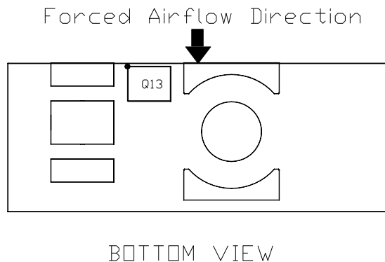
Figure 22. Airflow direction
