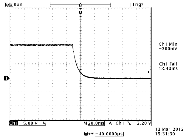
Figure 18. V_{out} = 12\text{ V} / 20\text{ A} at V_{in} = 48\text{ V} @ T_a = 25^\circ\text{C} , C_{ext} = 6800\text{ }\mu\text{F}
