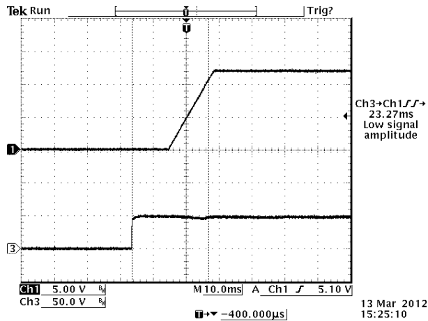
Figure 15. Startup from V_{in} Ch1: V_o Ch3: V_{in} V_{out} = 12\text{ V} / 20\text{ A} at V_{in} = 48\text{ V} @ T_a = 25^\circ\text{C} , C_{ext} = 6800\text{ }\mu\text{F}
