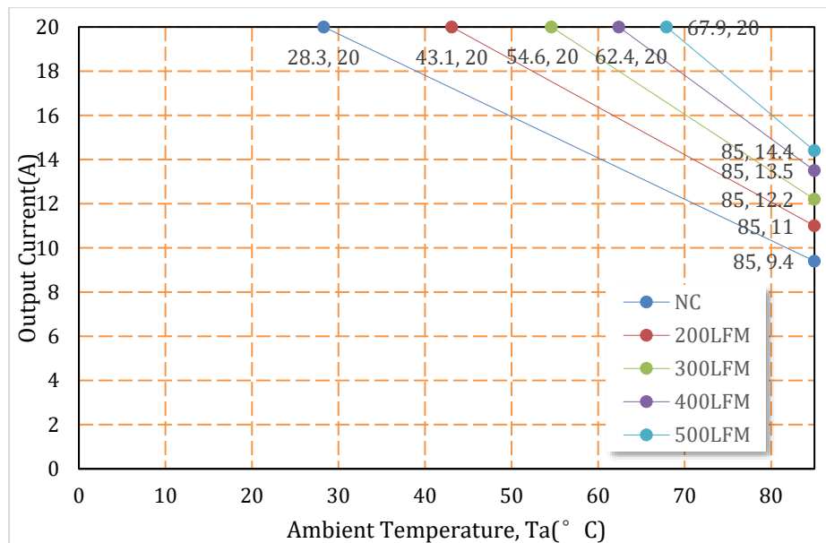
Figure 25. V_{in} = 48\text{ V} with baseplate version (ORCY-D4T12AG/BG)
