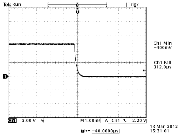
Figure 17. V_{out} = 12\text{ V} / 20\text{ A} at V_{in} = 48\text{ V} @ T_a = 25^\circ\text{C} , C_{ext} = 270\text{ }\mu\text{F}
