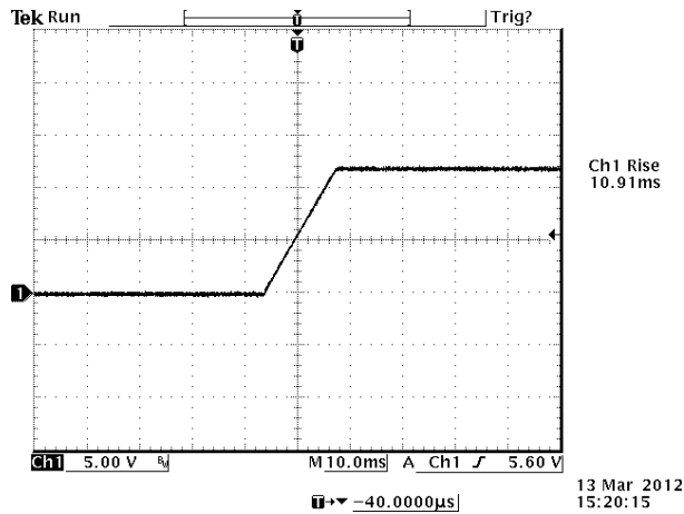
Figure 13. V_{out} = 12\text{ V} / 20\text{ A} at V_{in} = 48\text{ V} @ T_a = 25^\circ\text{C} , C_{ext} = 270\text{ }\mu\text{F}
