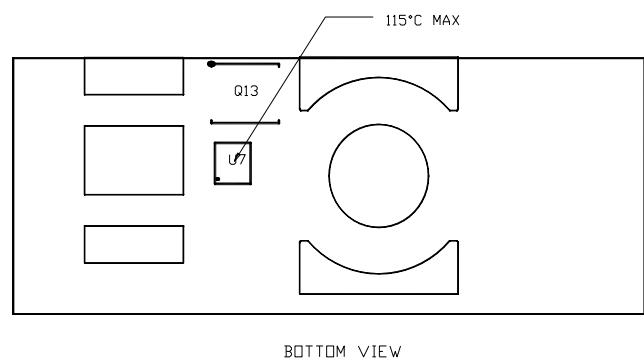
Figure 23. Hot spot
