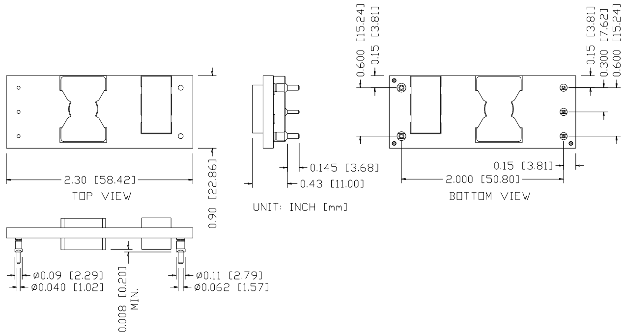
Figure 29. ORCY-D4T120G/LG Outline
