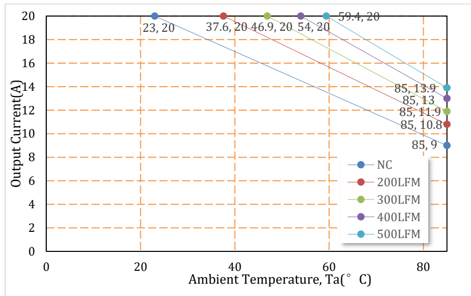
Figure 24. V_{in} = 48\text{ V} Open frame version (ORCY-D4T12LG/0G)
