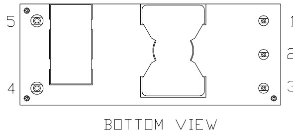
Figure 31. Pins
