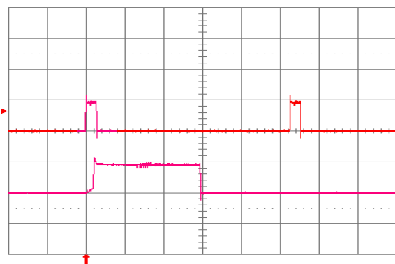
Fig. 1.8V.18: Load current (top trace, 20 A/div., 20 ms/div.) into a 10 \text{ m}\Omega short circuit during restart, at V_{in} = 24 \text{ V} . Bottom trace (20 A/div., 2 ms/div.) is an expansion of the on-time portion of the top trace.
