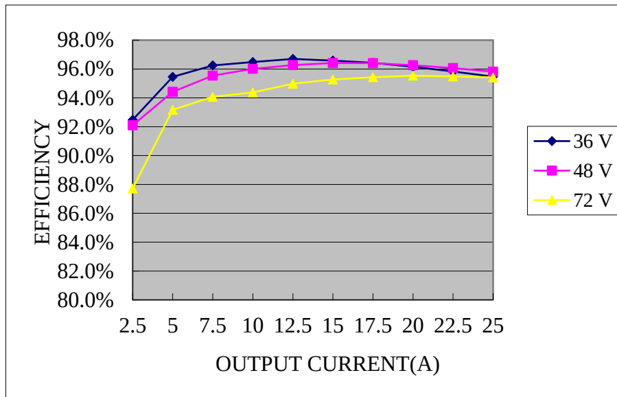
Figure 2. Efficiency data
