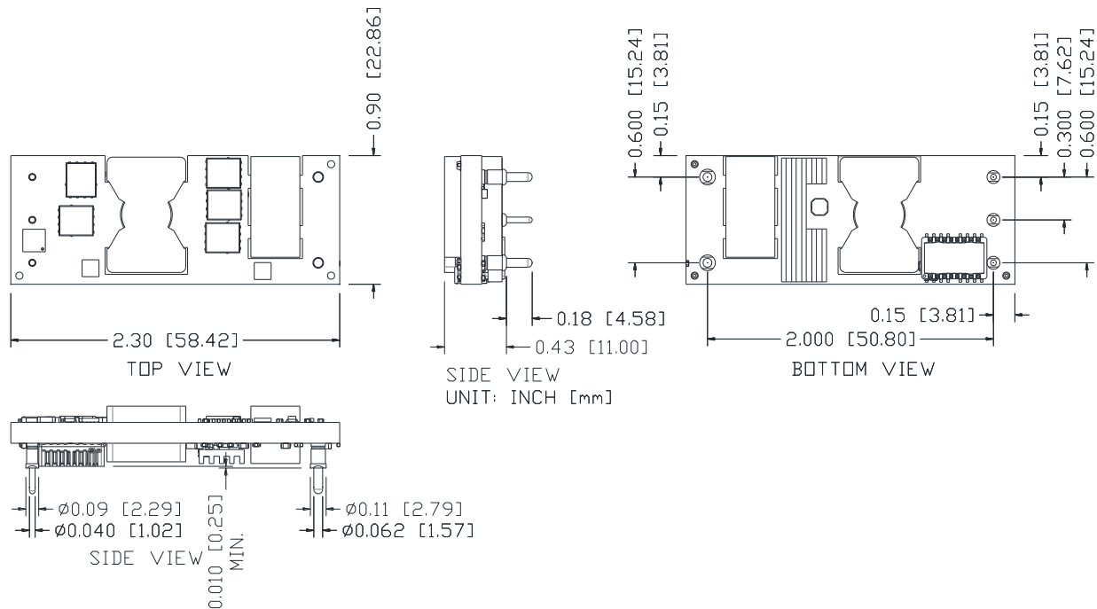
Figure 31. ORCY-T0T120G/LG Outline
