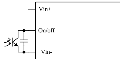
Figure 8. Control with photocoupler circuit
