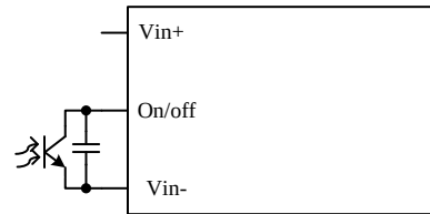
Figure 4. Control with photocoupler circuit
