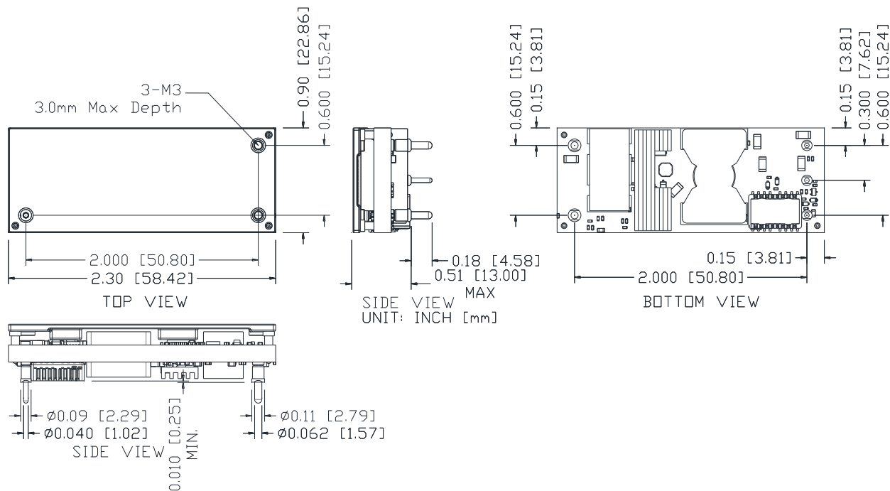
Figure 32. ORCY-T0T12AG/BG Outline
