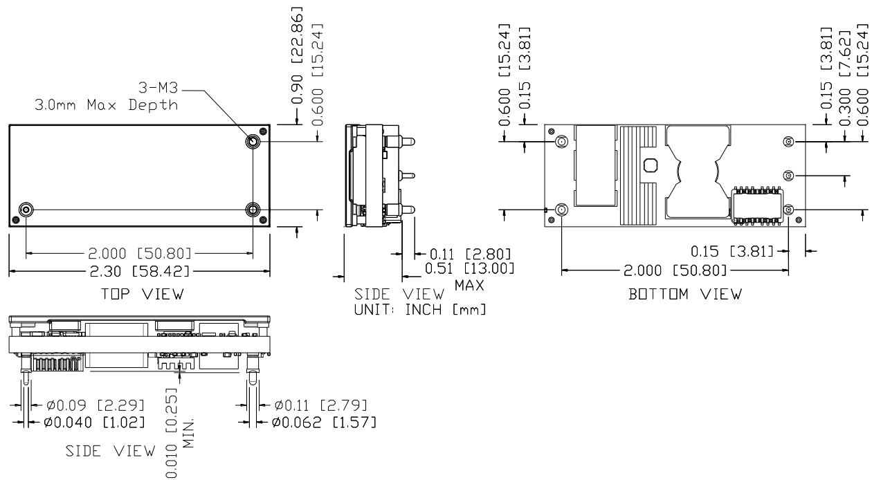
Figure 33. ORCY-T0T12C/N Outline
