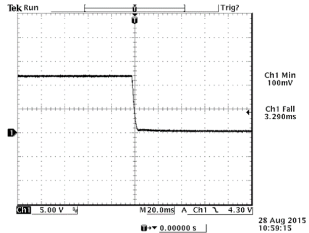
Figure 22. V_{out} = 12\text{ V} / 25\text{ A} at V_{in} = 48\text{ V} @ T_a = 25^\circ\text{C} , C_{ext} = 6800\text{ }\mu\text{F}
