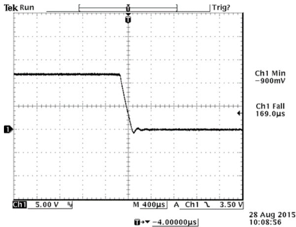
Figure 21. V_{out} = 12\text{ V} / 25\text{ A} at V_{in} = 48\text{ V} @ T_a = 25^\circ\text{C} , C_{ext} = 270\text{ }\mu\text{F}
