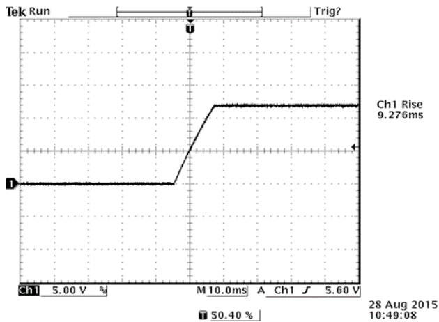
Figure 17. V_{out} = 12\text{ V} / 25\text{ A} at V_{in} = 48\text{ V} @ T_a = 25^\circ\text{C} , C_{ext} = 270\text{ }\mu\text{F}
