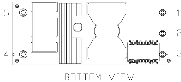
Figure 34. Pins
