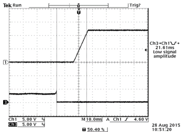
Figure 20. Startup from on/off Ch1: V_o Ch3: \text{on/off} V_{out} = 12\text{ V} / 25\text{ A} at V_{in} = 48\text{ V} @ T_a = 25^\circ\text{C} C_{ext} = 6800\text{ }\mu\text{F}
