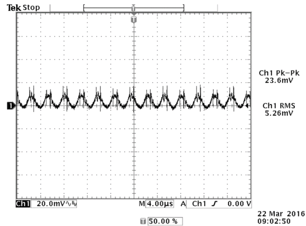
Figure 14. Ripple and noise waveform
