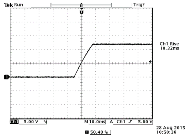
Figure 18. V_{out} = 12\text{ V} / 25\text{ A} at V_{in} = 48\text{ V} @ T_a = 25^\circ\text{C} , C_{ext} = 6800\text{ }\mu\text{F}
