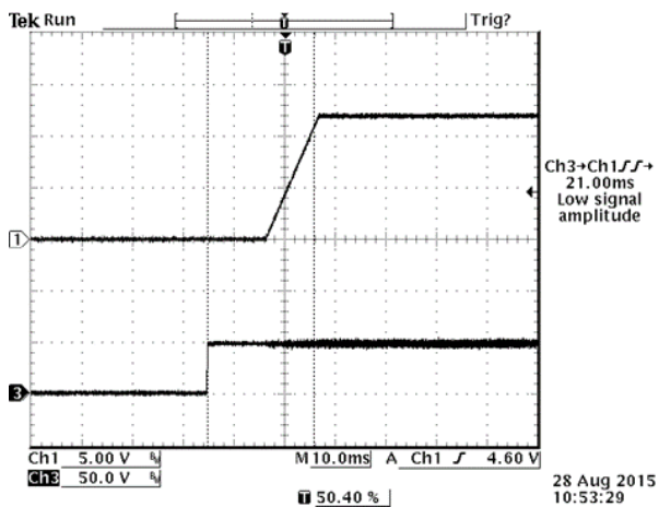
Figure 19. Startup from V_{in} Ch1: V_o Ch3: V_{in} V_{out} = 12\text{ V} / 25\text{ A} at V_{in} = 48\text{ V} @ T_a = 25^\circ\text{C} C_{ext} = 270\text{ }\mu\text{F}
