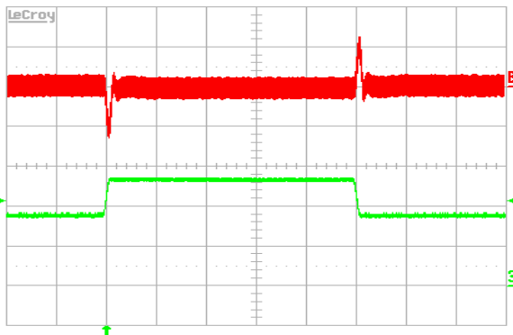
Figure 8. Output voltage response to load current step (3.5 A–5.25 A–3.5 A) at V_{in} = 48\text{ V} . Top trace: output voltage (100 mV/div.). Bottom trace: load current (2 A/div.). Current slew rate: 0.1 A/ \mu\text{s} . C_o = 1\text{ }\mu\text{F} ceramic + 10 \mu\text{F} tantalum. Time scale: 0.2 ms/div.
