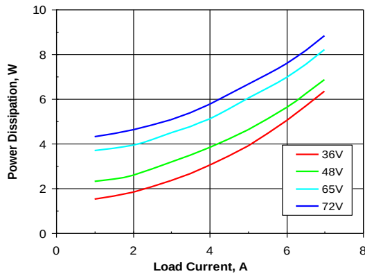
Figure 4. Power dissipation vs. load current and input voltage for SSQE48T07120 converter mounted vertically with air flowing from pin 1 to pin 3 at a rate of 300 LFM (1.5 m/s) and T_a = 25^\circ\text{C} .
