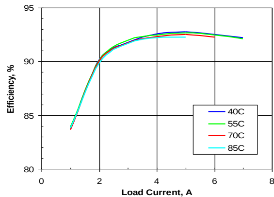
Figure 3. Efficiency vs. load current and ambient temperature for SSQE48T07120 converter mounted vertically with V_{in} = 48\text{ V} and air flowing from pin 1 to pin 3 at a rate of 200 LFM (1.0 m/s).
