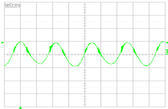
Figure 13. Input reflected-ripple-current, i_c (50 mA/div.), measured at input terminals at full rated load current and V_{in} = 48 \text{ V} . Refer to Figure 11 for test setup. Time scale: 1 \mu\text{s}/\text{div} .
