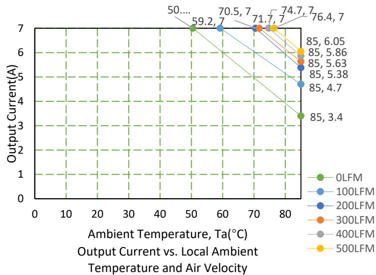
Figure 1. Available load current vs. ambient air temperature and airflow rates for SSQE48T07120 converter mounted vertically with air flowing from pin 1 to pin 3, V_{in} = 48\text{ V} . Note: NC – Natural convection
