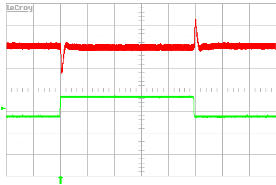
Figure 9. Output voltage response to load current step (3.5 A–5.25 A–3.5 A) at V_{in} = 48\text{ V} . Top trace: output voltage (100 mV/div.). Bottom trace: load current (2 A/div.). Current slew rate: 1 A/ \mu\text{s} . C_o = 100\text{ }\mu\text{F} Tantalum + 1 \mu\text{F} ceramic. Time scale: 0.2 ms/div.
