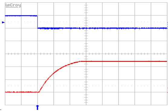
Figure 7. Turn-on transient at full rated load current (resistive) plus 3,300 \mu\text{F} at V_{in} = 48\text{ V} , triggered via ON/OFF pin. Top trace: ON/OFF signal (5 V/div.). Bottom trace: Output voltage (5 V/div.). Time scale: 2 ms/div.
