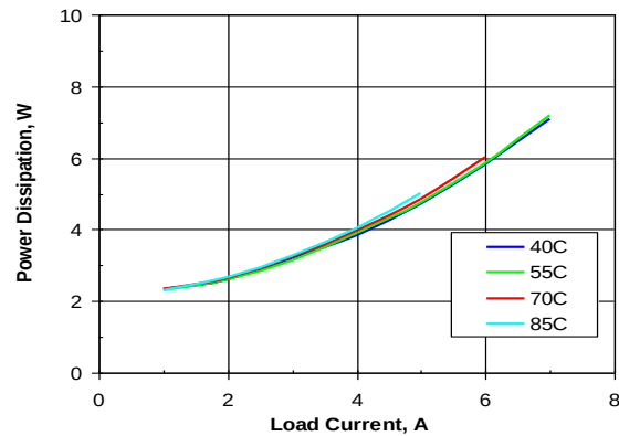
Figure 5. Power dissipation vs. load current and ambient temperature for SSQE48T07120 converter mounted vertically with V_{in} = 48\text{ V} and air flowing from pin 1 to pin 3 at a rate of 200 LFM (1.0 m/s).
