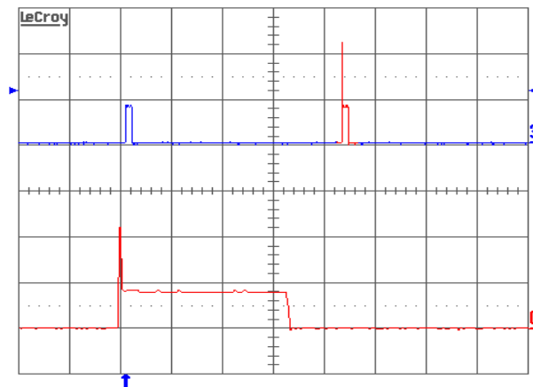
Figure 14. Load current (top trace, 5 \text{ A}/\text{div} ., 50 \text{ ms}/\text{div} .) into a 10 \text{ m}\Omega short circuit during restart, at V_{in} = 48 \text{ V} . Bottom trace ( 5 \text{ A}/\text{div} ., 2 \text{ ms}/\text{div} .) is an expansion of the on-time portion of the top trace.
