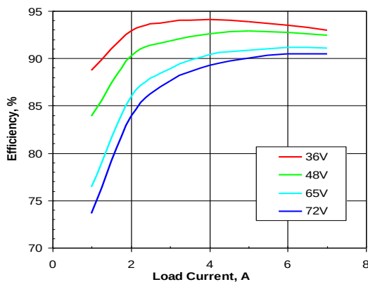
Figure 2. Efficiency vs. load current and input voltage for SSQE48T07120 converter mounted vertically with air flowing from pin 1 to pin 3 at a rate of 300 LFM (1.5 m/s) and T_a = 25^\circ\text{C} .
