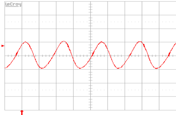
Figure 10. Output voltage ripple (10 mV/div.) at full rated load current into a resistive load with C_o = 10 \mu\text{F} tantalum + 1 \mu\text{F} ceramic and V_{in} = 48 \text{ V} . Time scale: 1 \mu\text{s}/\text{div} .
