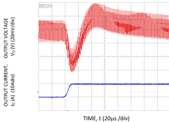
Figure 22. Transient Response to Dynamic Load Change from 50% to 100% at 12 Vin, Cout = 2x 47 \mu F + 2x 330 \mu F, CTune = 3300 pF & RTune = 220 ohms. Vo = 2.5 V
