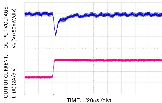
Figure 24. Transient Response to Dynamic Load Change from 50% to 100% at 12V in , C out = 2x47 μF, C Tune = 2200 pF, R Tune = 261 Ω. V o = 5.0 V
