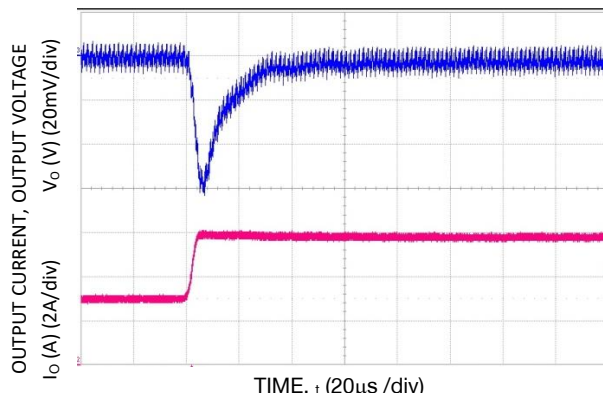
Figure 23. Transient Response to Dynamic Load Change from 50% to 100% at 12V in , C out = 3x47 μF, C Tune = 3300 pF, R Tune = 178 Ω. V o = 3.3 V
