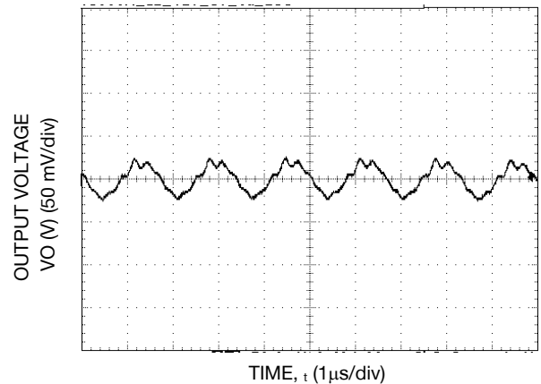
Figure 18. V_o = 5.0\text{ V} , I_o = I_{o, \max}
