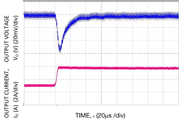
Figure 22. Transient Response to Dynamic Load Change from 50% to 100% at 12V in , C out = 3x47 μF, C Tune = 3300 pF, R Tune = 178 Ω. V o = 2.5 V
