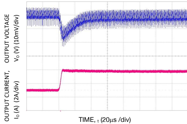
Figure 20. Transient Response to Dynamic Load Change from 50% to 100% at 12V in , C out = 1x47 μF + 2x330 μF, C Tune = 12 nF, R Tune = 178 Ω. V o = 1.2 V
