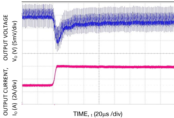
Figure 19. Transient Response to Dynamic Load Change from 50% to 100% at 12V in , C out = 1x47 μF + 4x330 μF, C Tune = 33 nF, R Tune = 178 Ω. V o = 0.6 V
