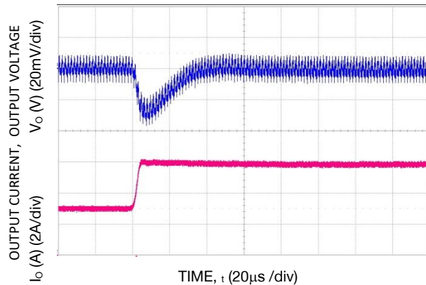
Figure 21. Transient Response to Dynamic Load Change from 50% to 100% at 12V in , C out = 1x47 μF + 1x330 μF, C Tune = 4700 pF, R Tune = 178 Ω. V o = 1.8 V
