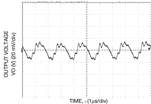
Figure 16. V_o = 2.5\text{ V} , I_o = I_{o, \max}
