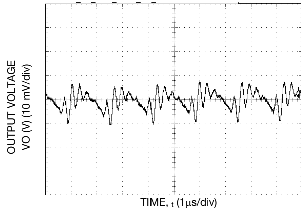
Figure 13. V_o = 0.6\text{ V} , I_o = I_{o, \max}
