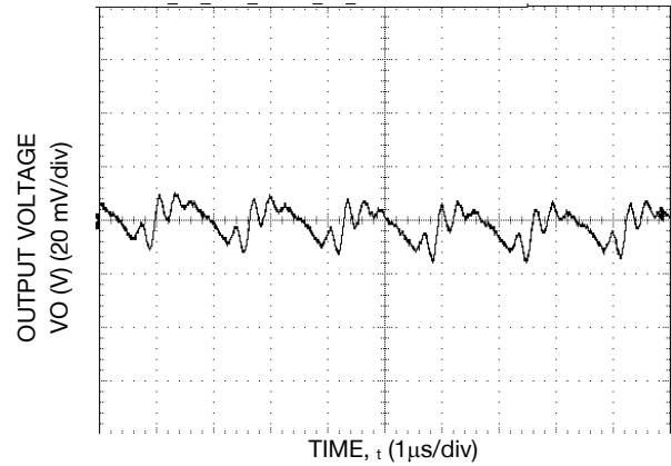
Figure 14. V_o = 1.2\text{ V} , I_o = I_{o, \max}
