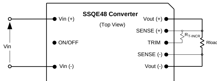
Figure C. Configuration for increasing output voltage.
