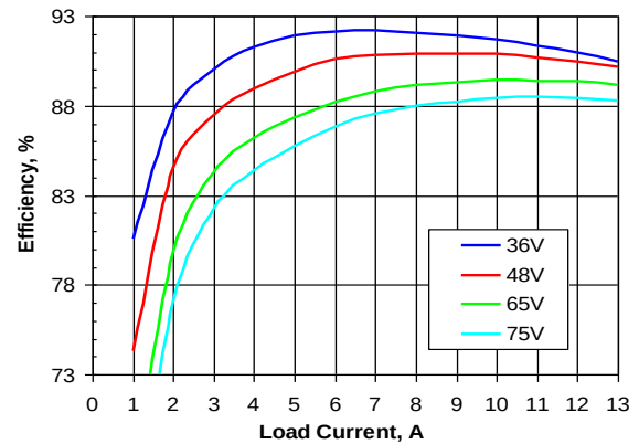
Figure 2. Efficiency vs. load current and input voltage for SSQE48T13050 converter mounted vertically with air flowing from pin 1 to pin 3 at a rate of 300 LFM (1.5 m/s) and T_a = 25^\circ\text{C} .
