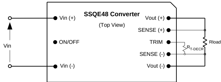
Figure D. Configuration for decreasing output voltage.
