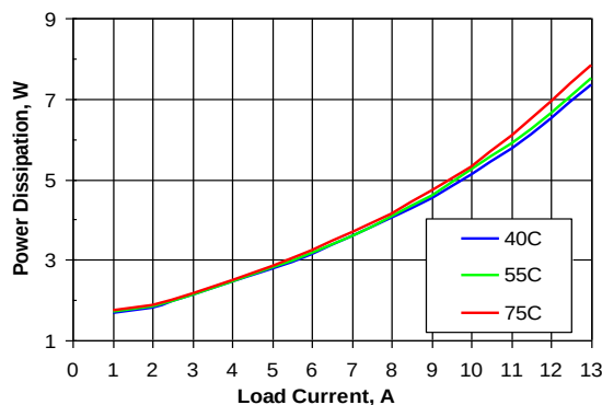
Figure 5. Power dissipation vs. load current and ambient temperature for SSQE48T13050 converter mounted vertically with V_{in} = 48\text{ V} and air flowing from pin 1 to pin 3 at a rate of 200 LFM (1.0 m/s).
