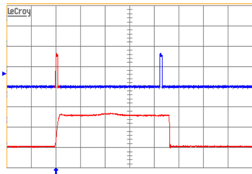
Figure 15. Load current (top trace, 10 A/div., 50 ms/div.) into a 10 m \Omega short circuit during restart, at V_{in} = 48 V. Bottom trace (10 A/div., 1.0 ms/div.) is an expansion of the on-time portion of the top trace.
