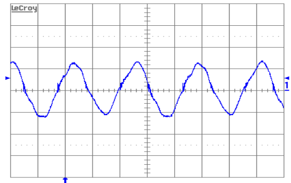
Figure 10. Output voltage ripple (20 mV/div.) at full rated load current into a resistive load with C_o = 10\text{ }\mu\text{F} tantalum + 1 \mu\text{F} ceramic and V_{in} = 48\text{ V} . Time scale: 1 \mu\text{s} /div.
