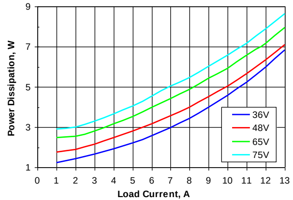
Figure 4. Power dissipation vs. load current and input voltage for SSQE48T13050 converter mounted vertically with air flowing from pin 1 to pin 3 at a rate of 300 LFM (1.5 m/s) and T_a = 25^\circ\text{C} .
