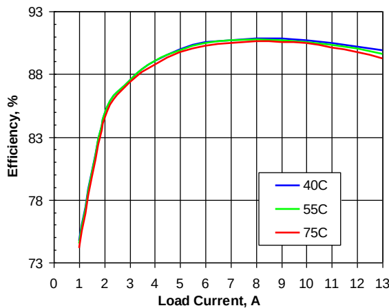
Figure 3. Efficiency vs. load current and ambient temperature for SSQE48T13050 converter mounted vertically with V_{in} = 48\text{ V} and air flowing from pin 1 to pin 3 at a rate of 200 LFM (1.0 m/s).
