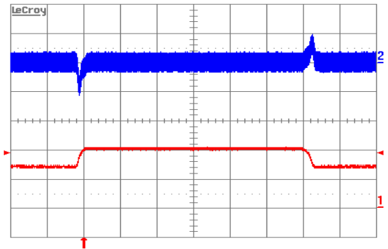
Figure 8. Output voltage response to load current step-change (6.5 A–9.75 A–6.5 A) at V_{in} = 48\text{ V} . Top trace: output voltage (100 mV/div.). Bottom trace: load current (5 A/div.). Current slew rate: 0.1 A/ \mu\text{s} . C_o = 1\text{ }\mu\text{F} ceramic + 10 \mu\text{F} tantalum. Time scale: 0.2 ms/div.
