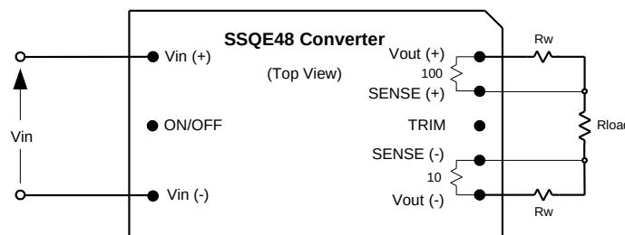
Figure B. Remote sense circuit configuration.
