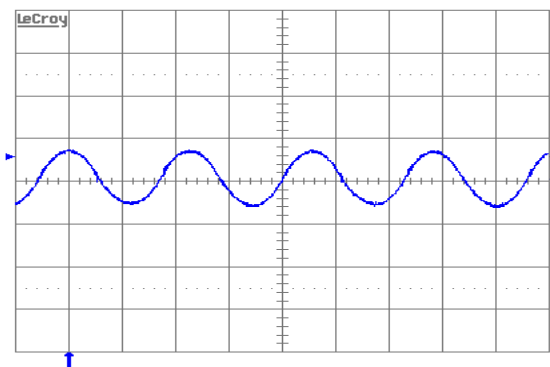
Figure 13. Input reflected ripple-current, i_c (200 mA/div.), measured at input terminals at full rated load current and V_{in} = 48 V. Refer to Figure 11 for test setup. Time scale: 1 \mu s/div.
