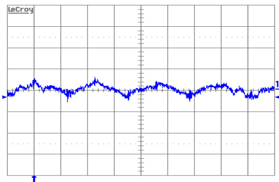
Figure 12. Input reflected-ripple current, i_s (10 mA/div.), measured through 10 \mu H at the source at full rated load current and V_{in} = 48 V. Refer to Figure 11 for test setup. Time scale: 1 \mu s/div.
