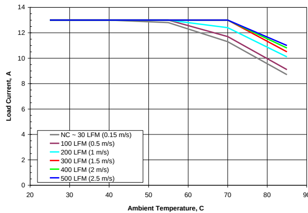
Figure 1. Available load current vs. ambient air temperature and airflow rates for SSQE48T13050 converter mounted vertically with air flowing from pin 1 to pin 3, V_{in} = 48\text{ V} . Note: NC – Natural convection
