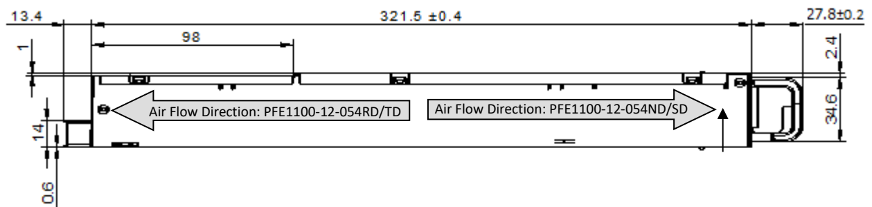
Figure 3. Side View 1
