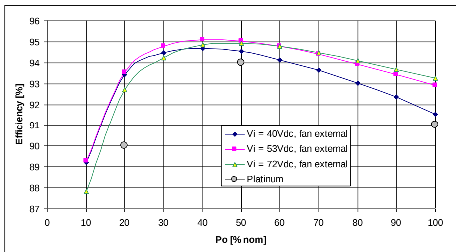
Figure 1. Efficiency
