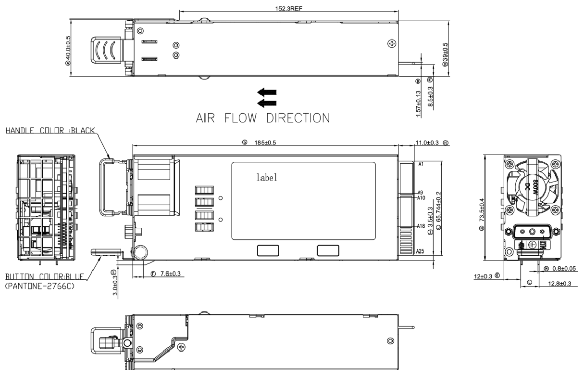
Figure 5. Mechanical Drawing
