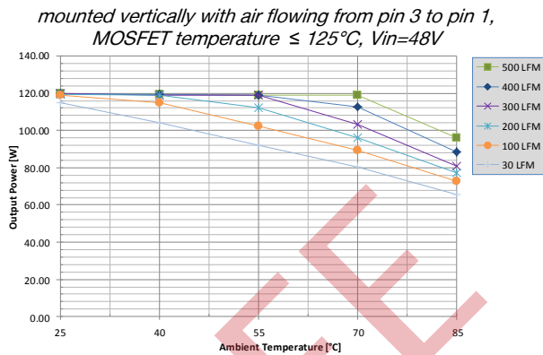
Fig. 4: Power derating vs. ambient air temperature and airflow rates for UIE48T36033 converter w/o baseplate mounted vertically with air flowing from pin 3 to pin 1, MOSFET temperature \leq 125^{\circ}\text{C} , V_{in}=48\text{V}
