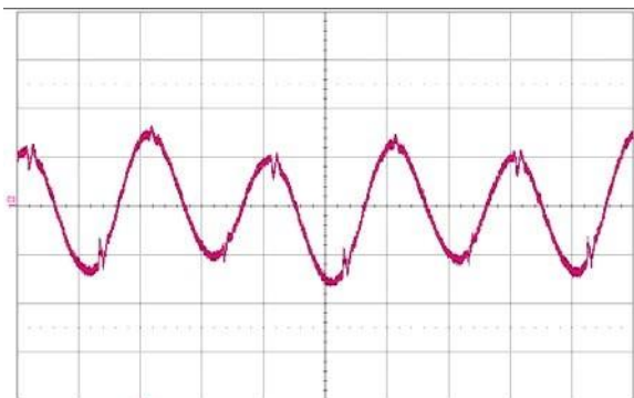
Figure 15. Input reflected ripple-current, i_s (50 mA/div.), measured at input terminals at full rated load current and V_{in} = 48 V. Refer to Fig. J for test setup. Time scale: 1 μs/div.
