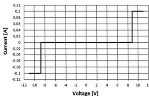
Voltage Sweeping of I/O_1 to I/O_2
