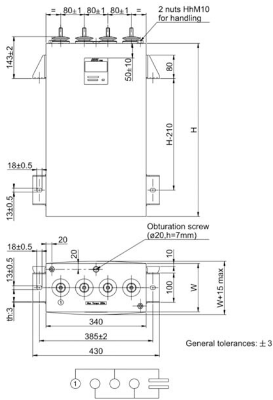
4 TERMINALS Type 2
