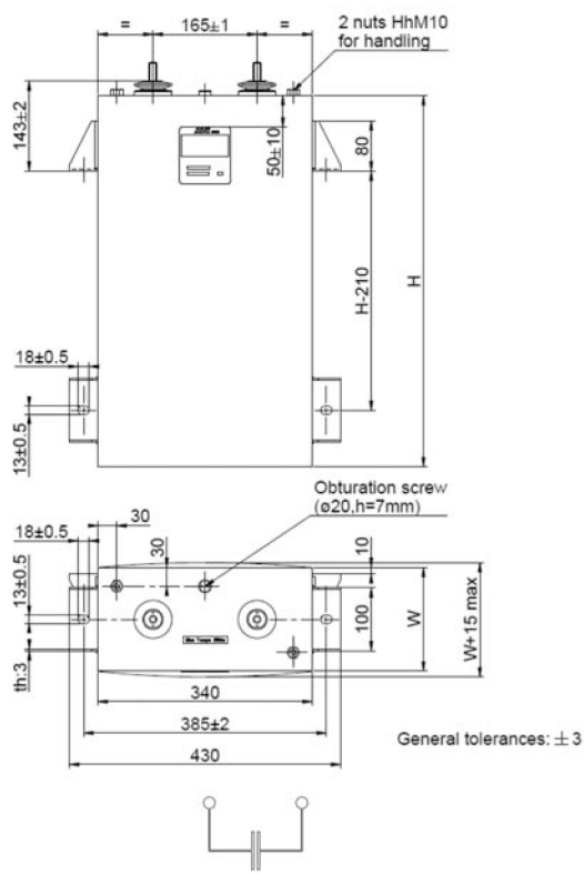
2 TERMINALS Type 2
