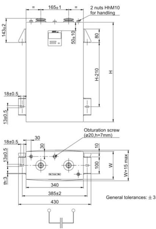
2 TERMINALS Type 2
