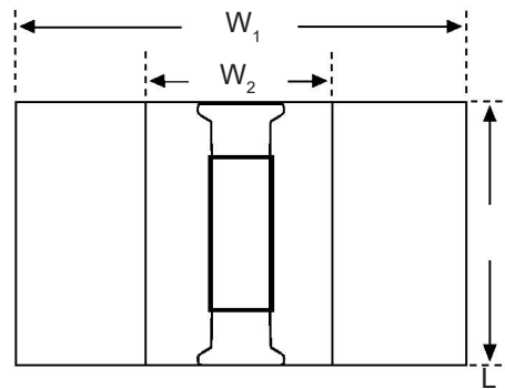
Substrate W_1 or Substrate W_2 Length is determined by transmission line
