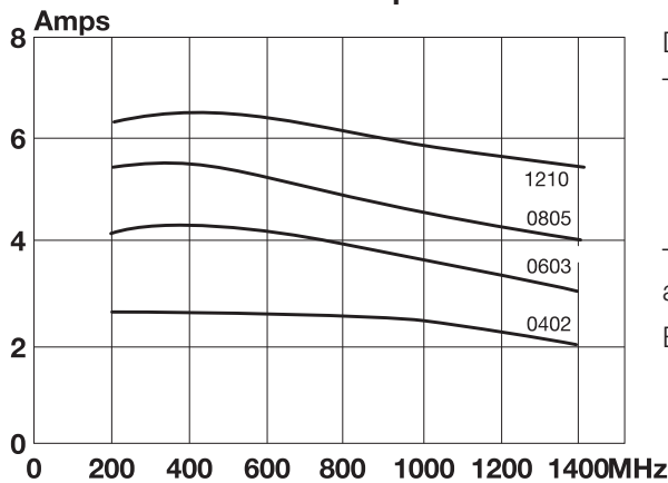
Power Handling Accu-P® 10pF
