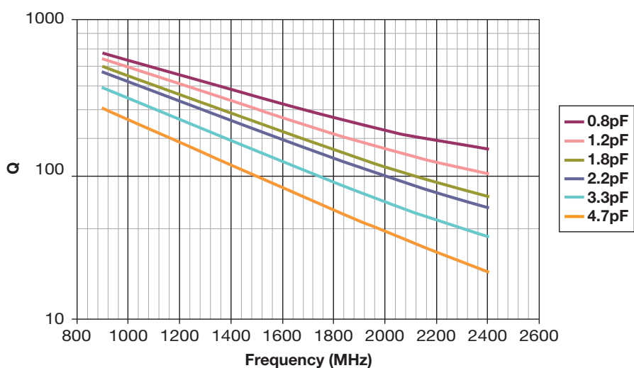
Accu-P ® 0402 Typical Q vs Frequency
