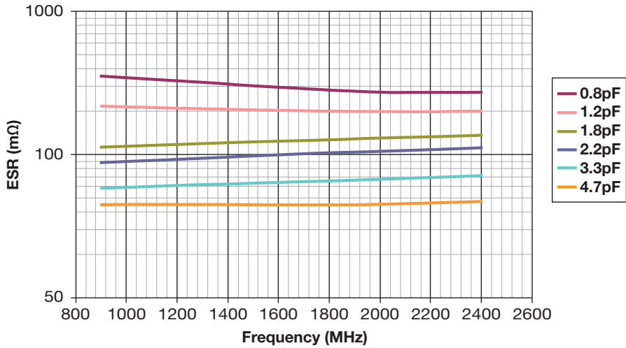
Accu-P ® 0402 Typical ESR vs Frequency
