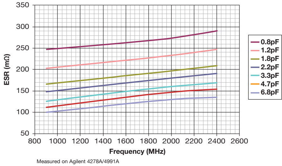
Accu-P ® 0603 Typical ESR vs Frequency
