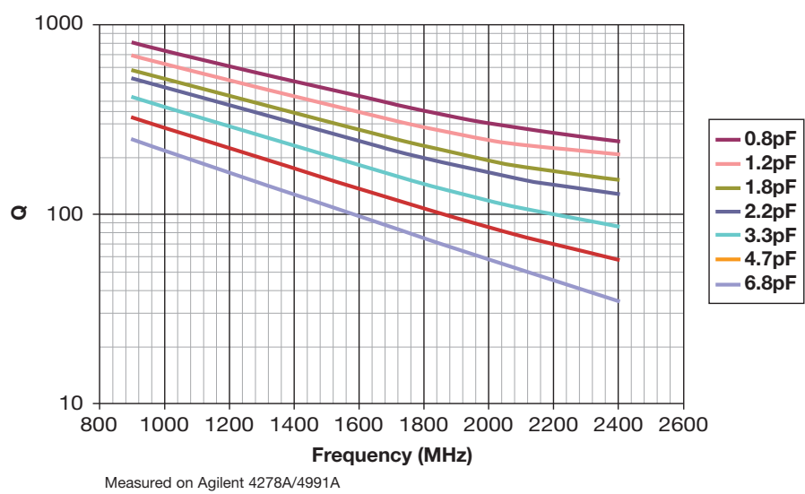
Accu-P ® 0603 Typical Q vs Frequency
