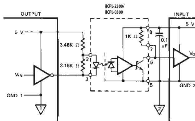
Figure 14. Series drive from open collector TTL/LSTTL units.
