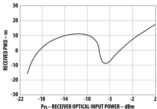
Figure 8. Typical POF receiver pulse width distortion vs. optical power at 10 MBd
