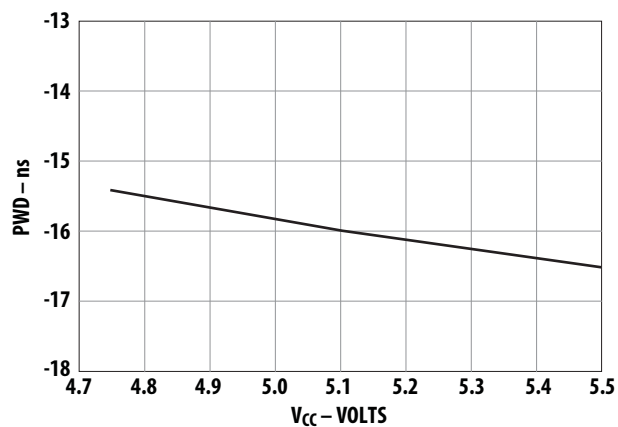
Figure 10. Typical POF receiver pulse width distortion vs. power supply voltage at low optical power (-21 dBm, 10 MBd)
