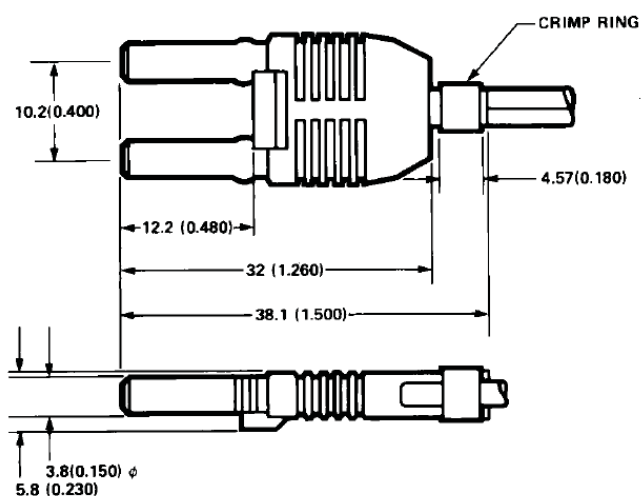
HFBR-4506Z (Parchment) Duplex Connector
