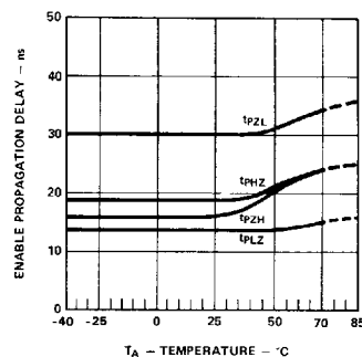
Figure 10. Typical Enable Propagation Delay vs. Ambient Temperature.
