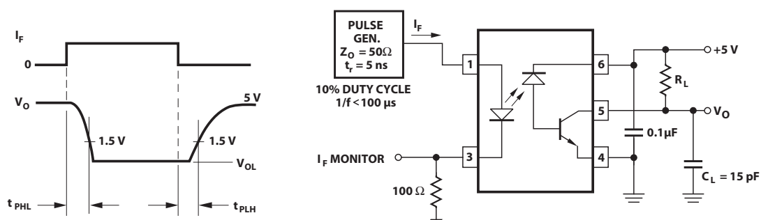
Figure 8. Switching Test Circuit
