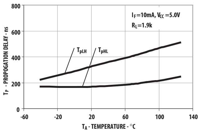
Figure 5. Propagation Delay vs Temperature
