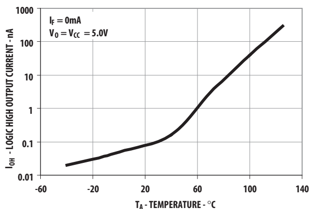
Figure 7. Logic High Output Current vs Temperature.
