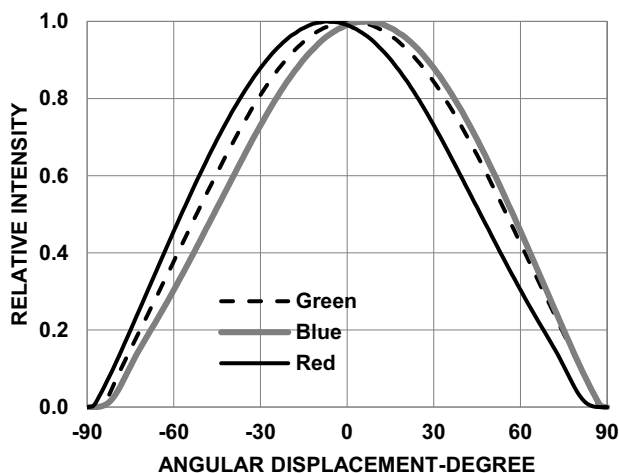
Figure 11: Radiation Pattern for Y-Axis
