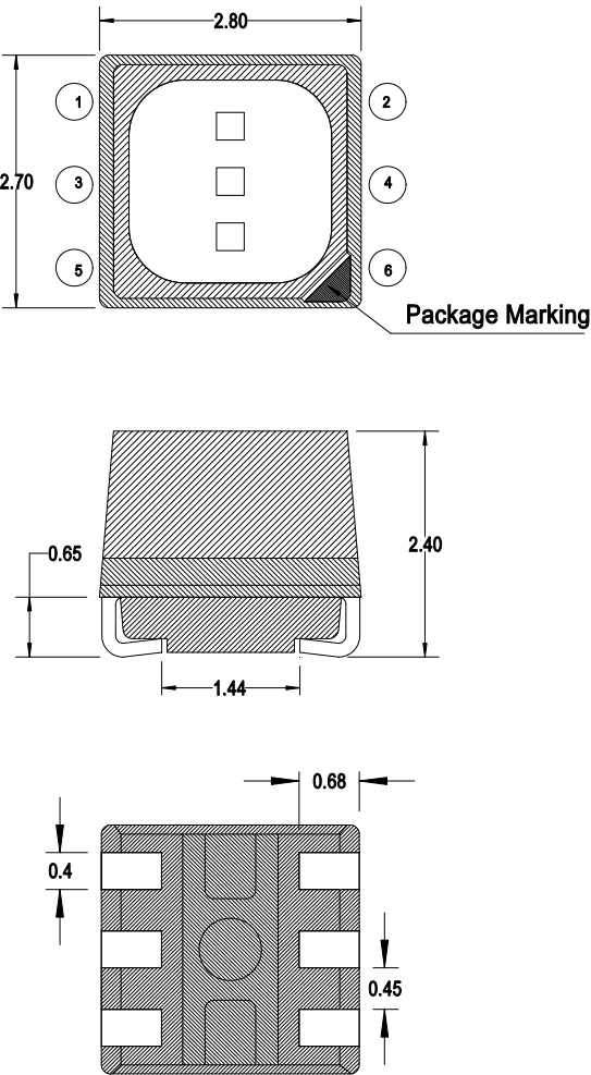
Figure 1: Package Drawing
