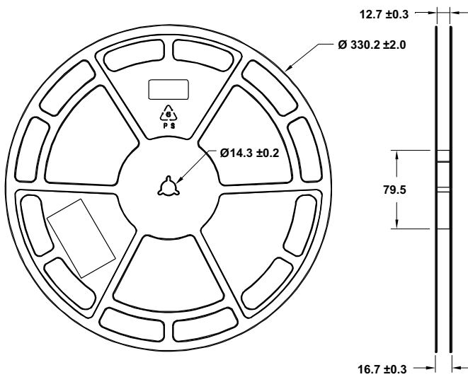
Figure 14: Reel Dimensions
