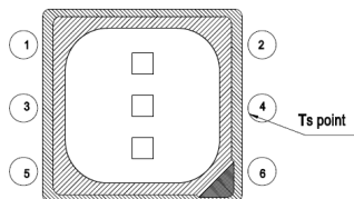
Figure 17: Solder Point Temperature on PCB
