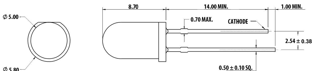
Figure 1: Package Drawing
