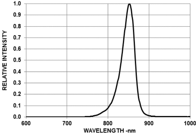
Figure 6: Spectral Distribution
