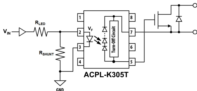
Figure 18: Photovoltaic Driver + Two Back-To-Back MOSFET
