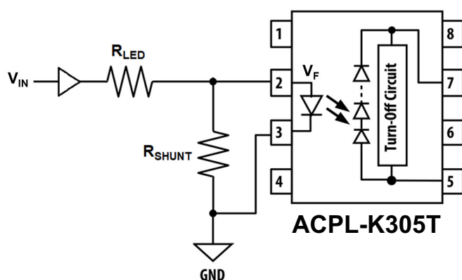
Figure 16: Circuit Diagram
