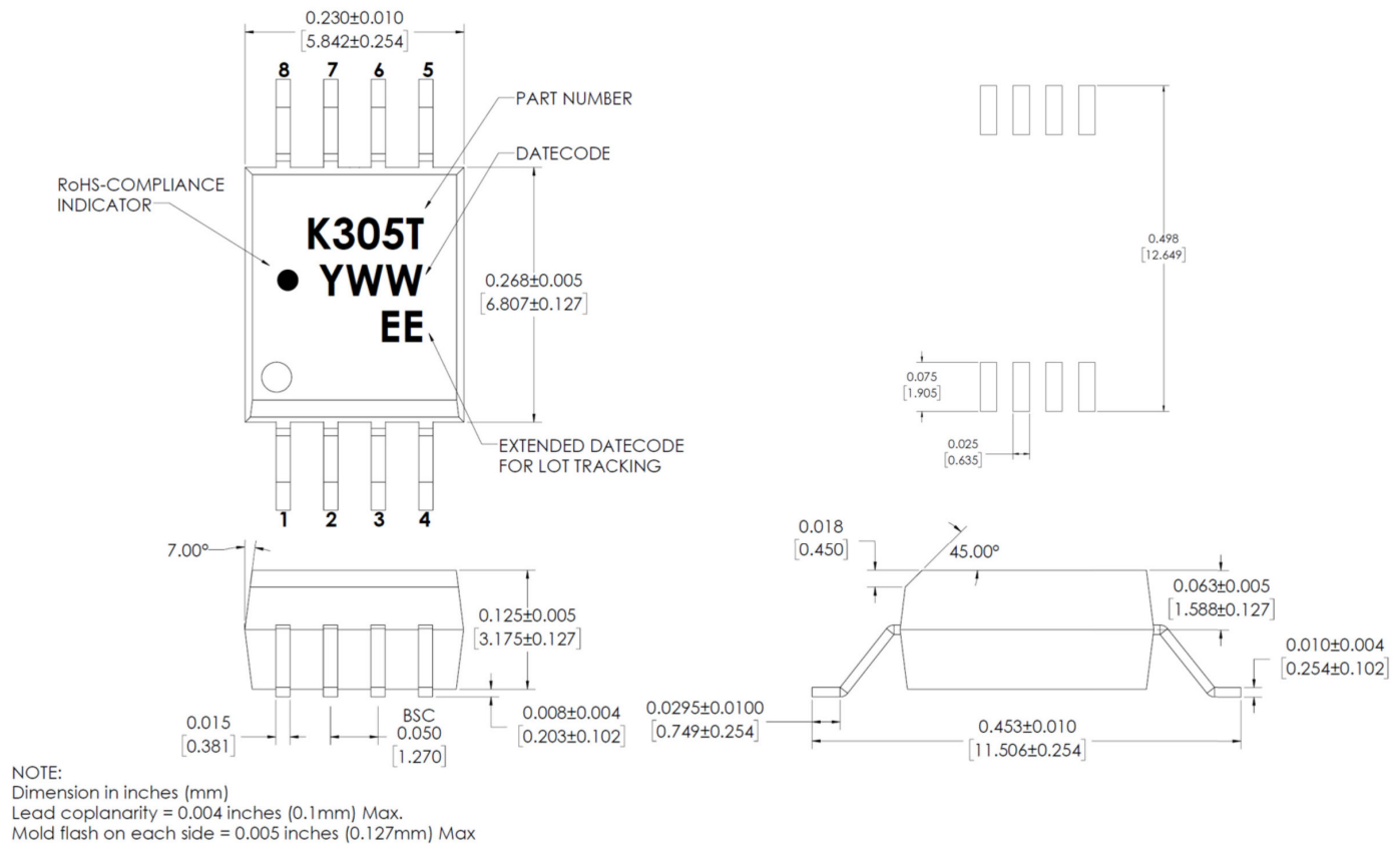
Figure 4: Stretched SO-8 Package
