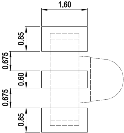
Figure 7: Recommended Soldering Land Pattern
