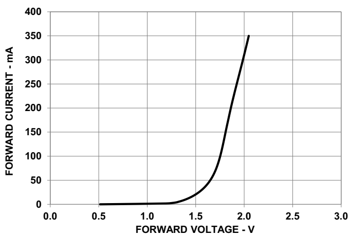
Figure 3: Forward Current vs. Forward Voltage
