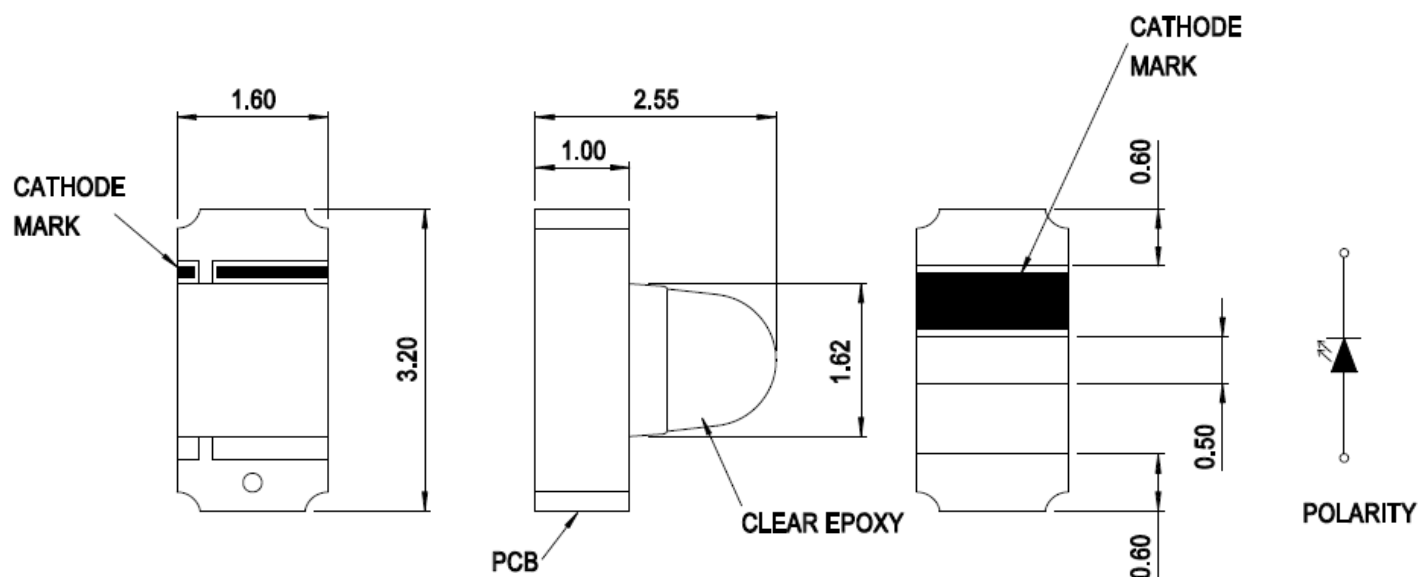
Figure 1: Package Drawing
