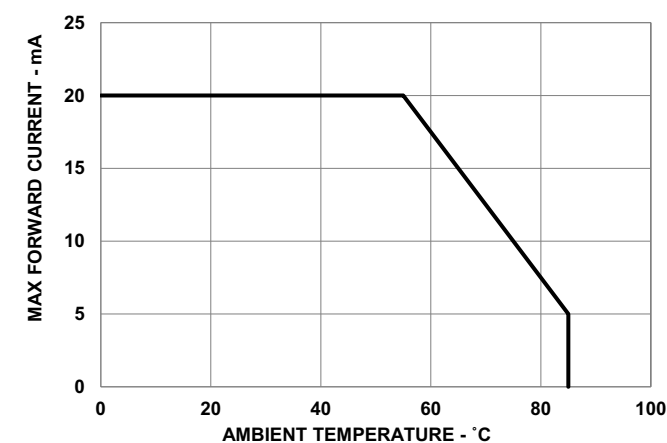
Figure 6: Derating Curve
