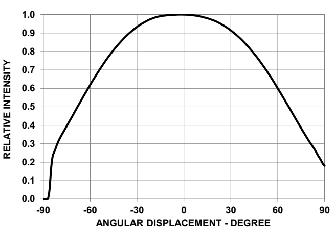
Figure 5: Radiation Pattern
