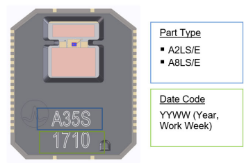
Figure 4: Product Marking Information
