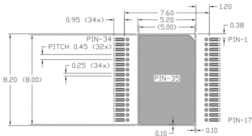
Figure 6: PCB Land Pattern
