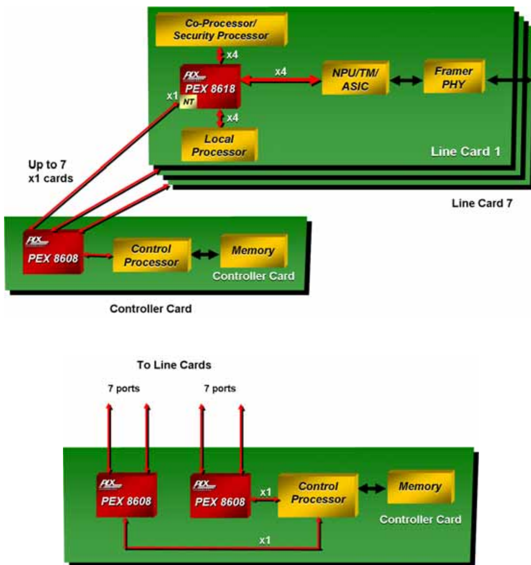
Figure 2-3. Control Plane Application
