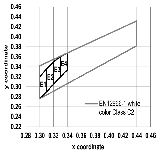
Figure 2: Chromaticity Diagram
