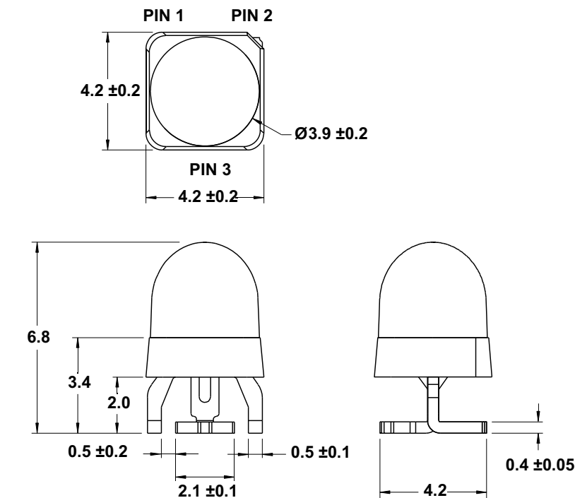
Figure 1: Package Drawing
