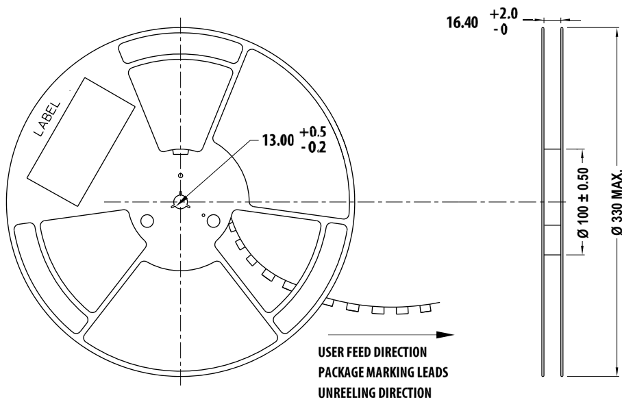
Figure 13: Reel Dimensions
