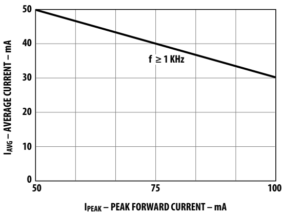
Figure 7: Maximum Average Current vs. Peak Forward Current, HLMA-xxxx
