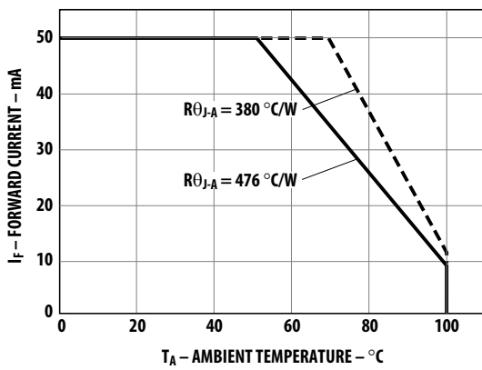
Figure 6: Maximum Forward Current vs. Ambient Temperature
