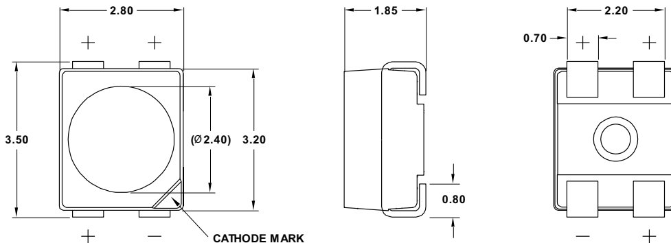
Figure 1: Package Drawing
