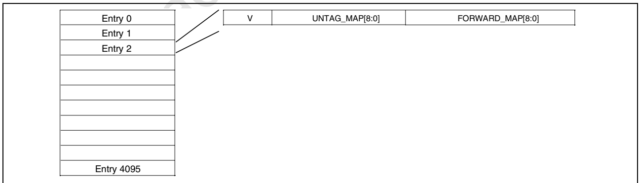
Figure 3: VLAN Table Organization
