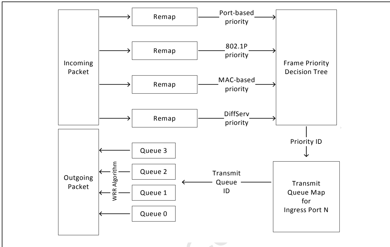
Figure 2: QoS Block Diagram
