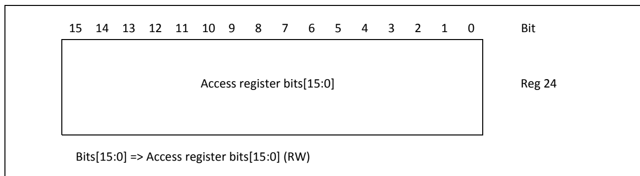
Figure 22: Pseudo-PHY MII Register 24: Access Register Bit Definition
