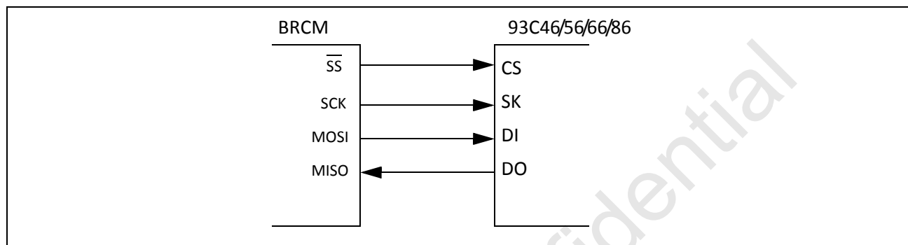
Figure 17: Serial EEPROM Connection
