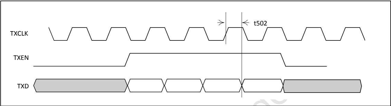
Figure 40: GMII Output Timing
