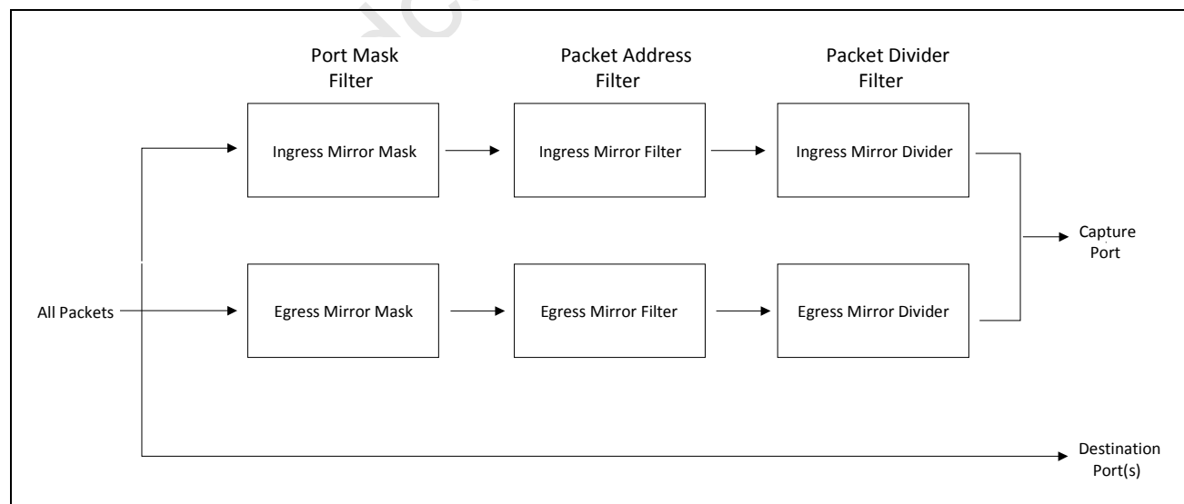
Figure 6: Mirror Filter Flow
