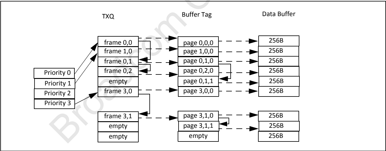
Figure 8: TXQ and Buffer Tag Structure
