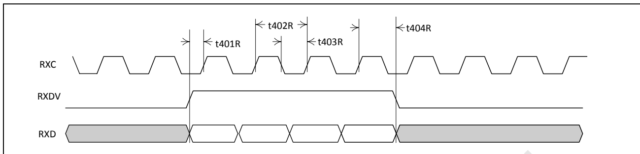
Figure 35: RvMII Mode Input Timing
