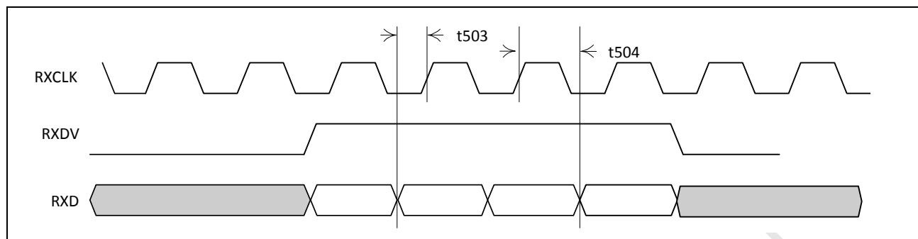
Figure 41: GMII Input Timing
