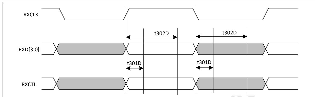
Figure 39: RGMII Input Timing (Delayed Mode)
