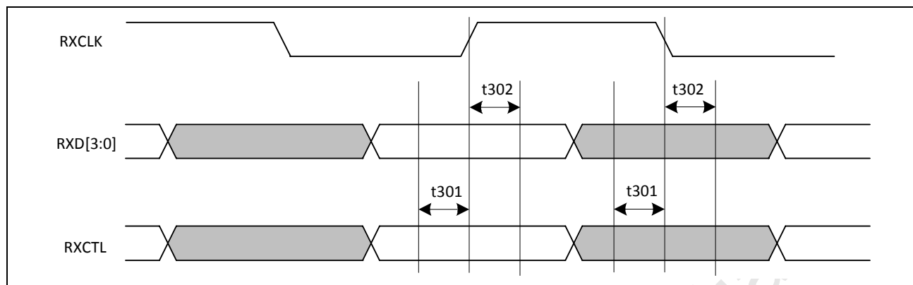
Figure 38: RGMII Input Timing (Normal Mode)
