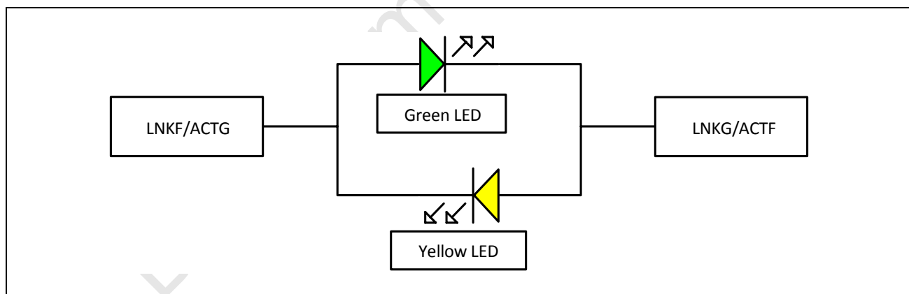
Figure 28: Bicolor Link/Act LED Scheme
