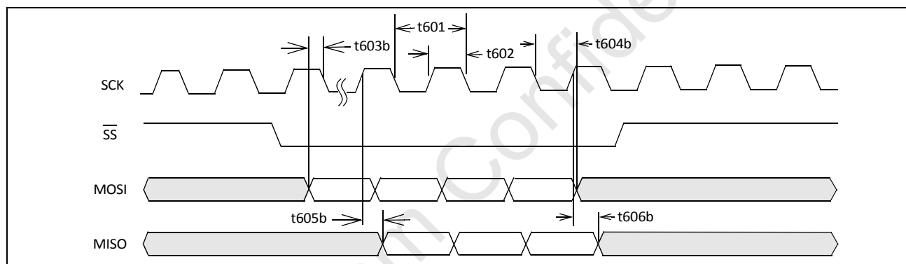
Figure 45: SPI Timing, \overline{SS} Asserted During SCK Low
