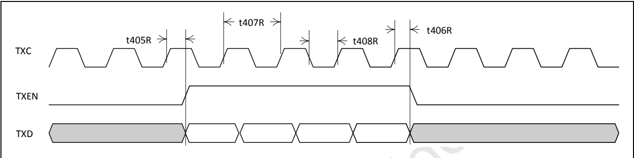
Figure 34: RvMII Mode Output Timing
