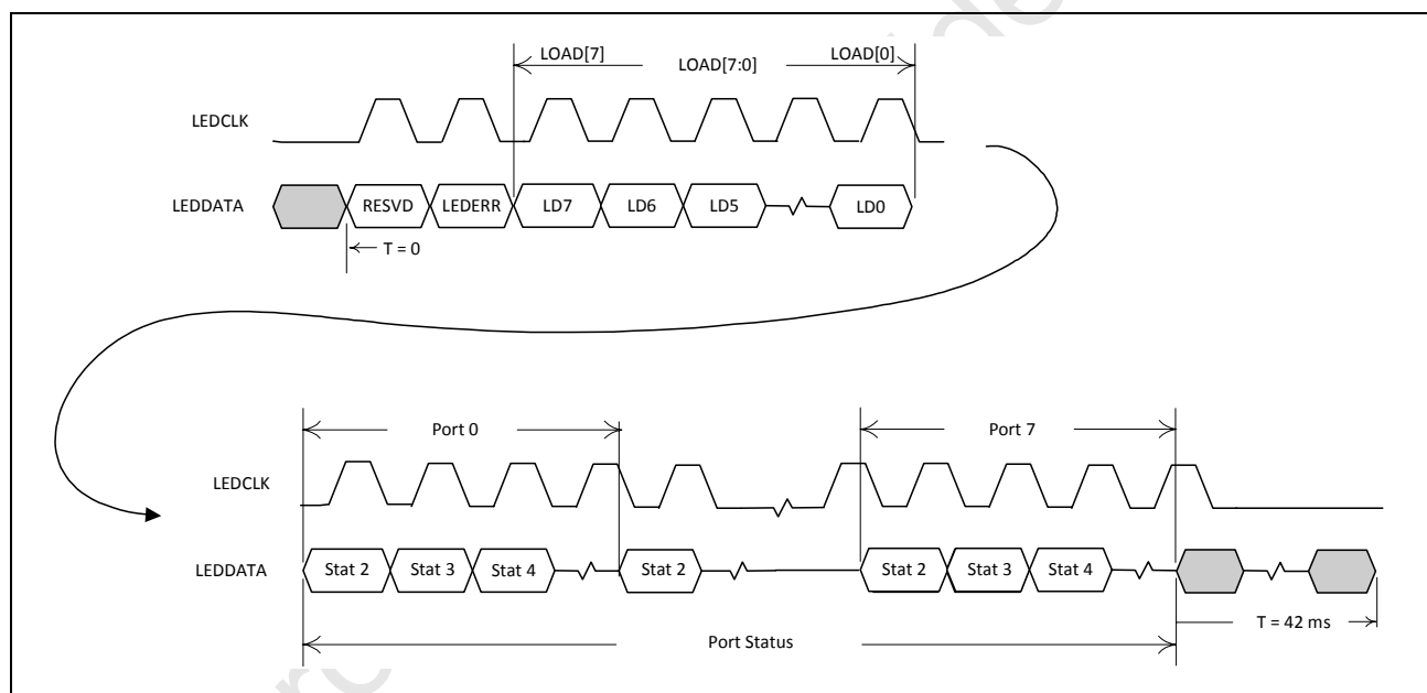
Figure 29: Serial LED Shift Sequence
