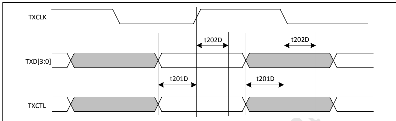
Figure 37: RGMII Output Timing (Delayed Mode)
