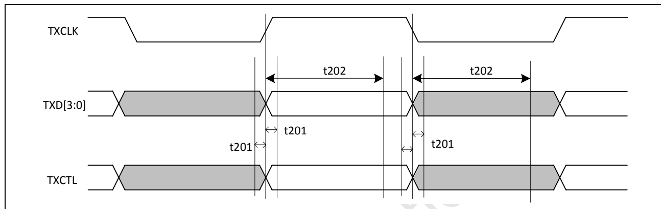
Figure 36: RGMI Output Timing (Normal Mode)
