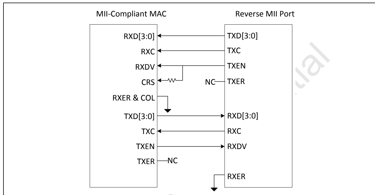
Figure 9: RvMII Port Connection
