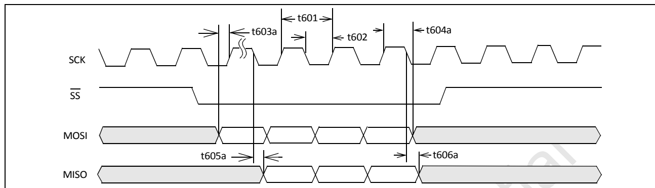
Figure 44: SPI Timing, \overline{SS} Asserted During SCK High
