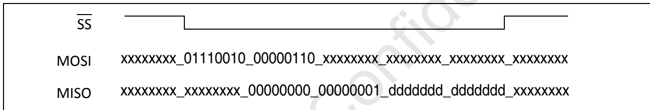
Figure 16: Timing Example
