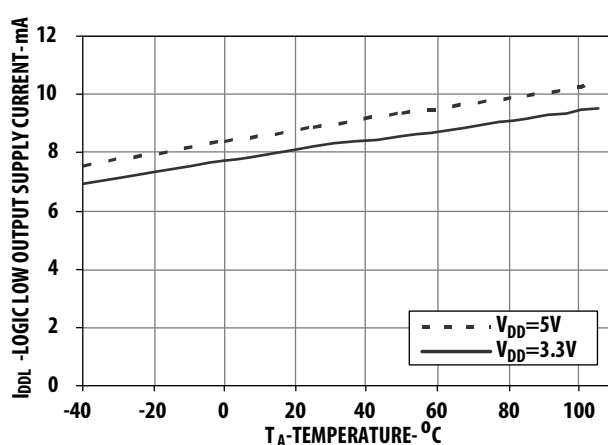
Figure 4 Typical Logic Low Output Supply Current vs. Temperature for Dual Channel (ACPL-K73L)
