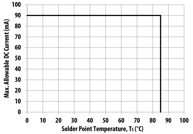
Figure 16: Maximum Forward Current vs. Solder Point Temperature. Derated based on T_{JMAX} = 120^{\circ}C , R_{\theta J-S} = 46^{\circ}C/W .
