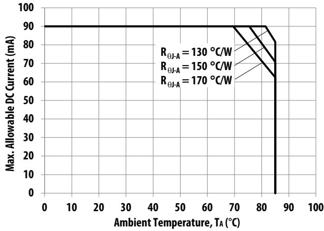
Figure 15: Maximum Forward Current vs. Ambient Temperature. Derated based on T_{JMAX} = 120^{\circ}C , R_{\theta J-A} = 130^{\circ}C/W , 150^{\circ}C/W and 170^{\circ}C/W .
