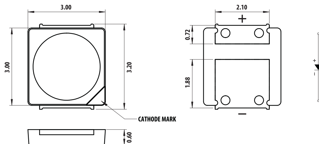
Figure 1 Package Drawing
