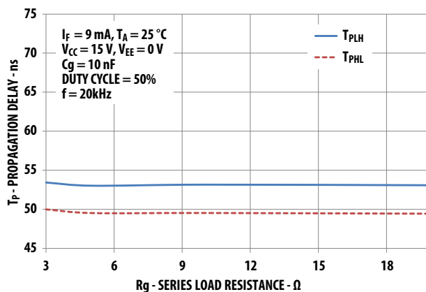
Figure 10: Propagation Delay vs. R_g
