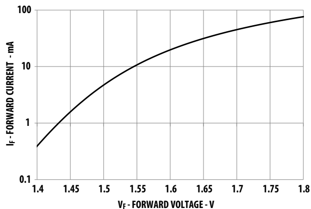
Figure 12: Input Current vs. Forward Voltage
