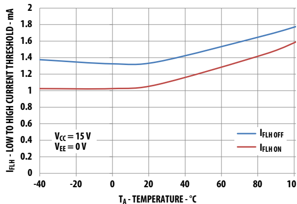
Figure 6: I_{FLH} vs. Temperature
