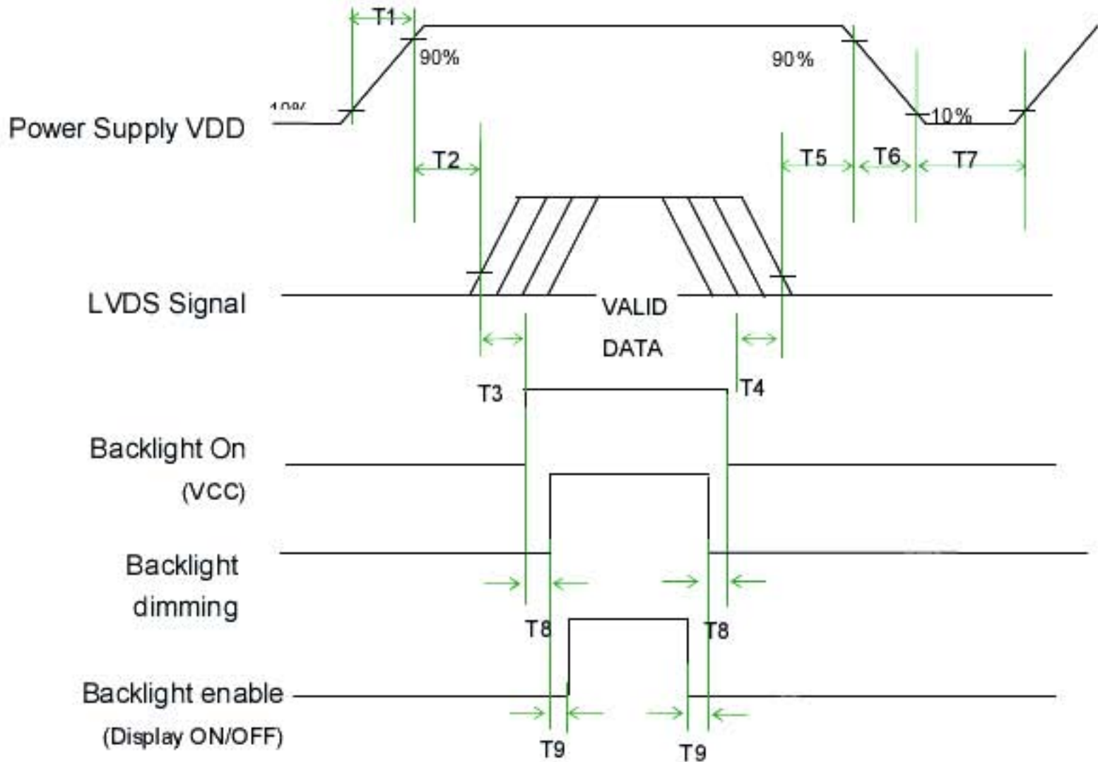
Power ON/OFF sequence timing
