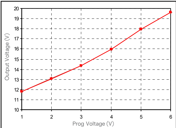
Figure 30: LCM600N Output Voltage Adjustment by Vprom @ 25 degC Loading: Io = 0A (15V), ISB = 0A (5V) ◆ 115 Vac ■ 230 Vac
