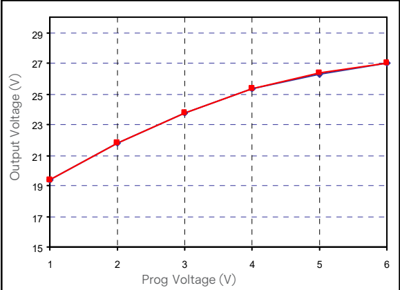
Figure 45: LCM600Q Output Voltage Adjustment by Vprom @ 25 degC Loading: Io = 0A (24V), I SB = 0A (5V) ◆ 115 Vac ■ 230 Vac
