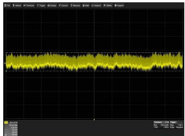
Figure 25: LCM600N Ripple and Noise Measurement V_{in} = 90\text{Vac} Load: I_o = 40\text{A} (15V), I_{sb} = 2\text{A} (5V) Ch 1: V_o
