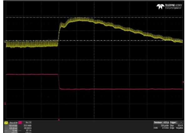
Figure 23: LCM600N Transient Response - V_o Deviation (high to low) 100% to 10% load change 1A/uS slew rate V_{in} = 230\text{Vac} Ch 1: V_o Ch 2: I_o
