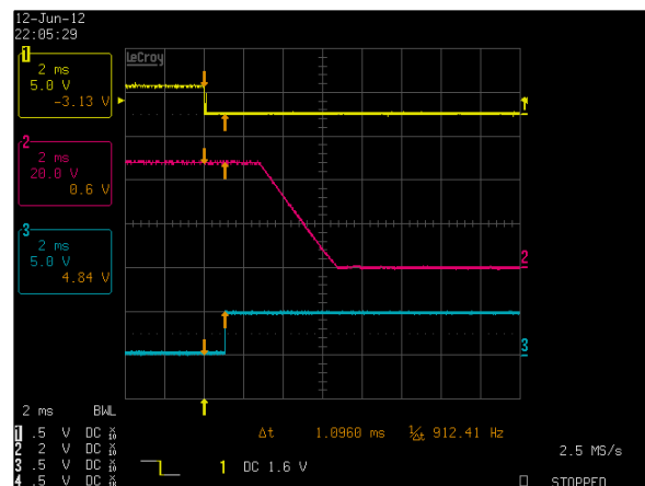
Figure 62: LCM600W Turn Off Characteristic via INH_EN
