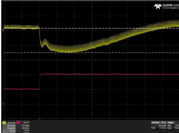
Figure 22: LCM600N Transient Response - V_o Deviation (low to high) 10% to 100% load change 1A/uS slew rate V_{in} = 230\text{Vac} Ch 1: V_o Ch 2: I_o
