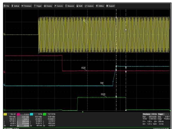
Figure 27: LCM600N ACOK Signal Turn Off Delay - V_{in} = 100\text{Vac} Load: I_o = 2\text{A} (12V), I_{sb} = 0\text{A} (5V) Ch 1: AC Mains Ch 2: ACOK Ch 3: V_o Ch 4: DCOK
