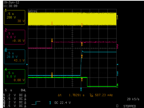
Figure 58: LCM600W Turn-on delay via INH_EN - Vin = 90Vac
