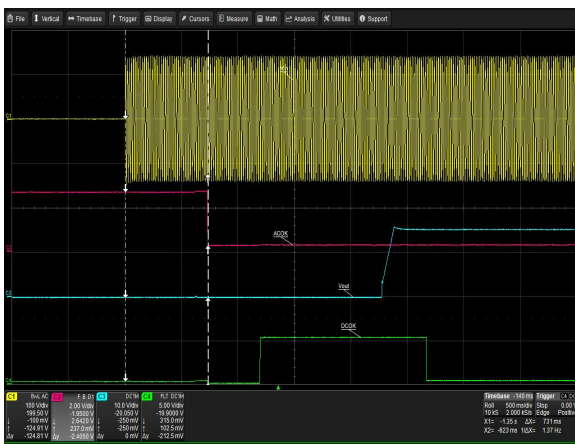
Figure 26: LCM600N ACOK Signal Turn On Delay - V_{in} = 100\text{Vac} Load: I_o = 2\text{A} (12V), I_{sb} = 0\text{A} (5V) Ch 1: AC Mains Ch 2: ACOK Ch 3: V_o Ch 4: DCOK
