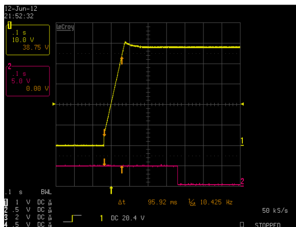
Figure 61: LCM600W Output Voltage Startup Characteristic
