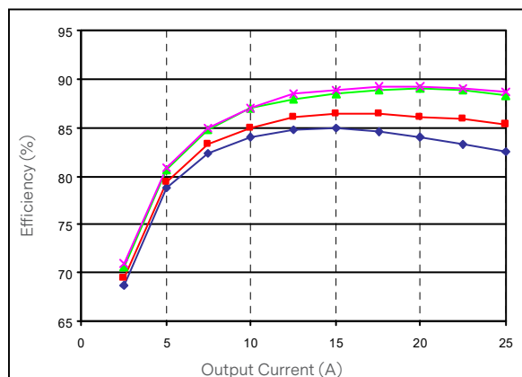
Figure 39: LCM600Q Efficiency Curves @ 25 degC, ◆ 90 Vac ■ 115 Vac ▲ 230 Vac ✕ 264 Vac Loading: V_o = 10\% increment to 25A, I_{SB} = 0A (5V)
