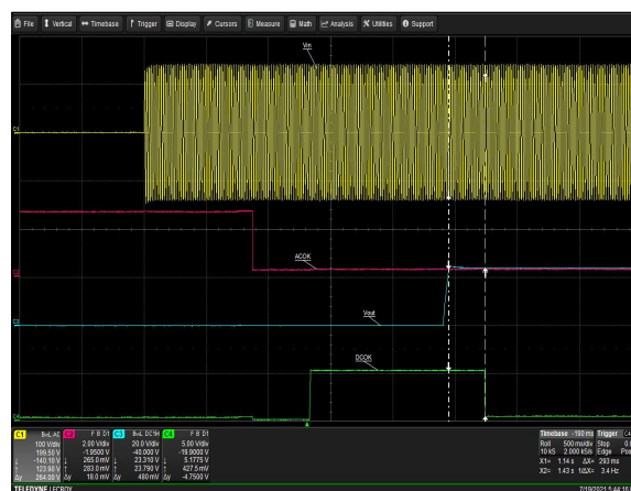
Figure 42: LCM600Q ACOK Signal Turn Off Delay – V_{in} = 100V_{ac} Load: I_o = 2A (12V), I_{SB} = 0A (5V) Ch 1: AC Mains Ch 2: ACOK Ch 3: V_o Ch 4: DCOK
