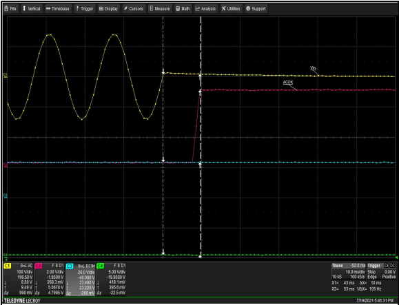
Figure 43: LCM600N DCOK Signal Turn On Delay – Vin = 100Vac Load: Io = 2A (12V), I SB = 0A (5V) Ch 1: AC Mains Ch 2: ACOK Ch 3: Vo Ch 4: DCOK
