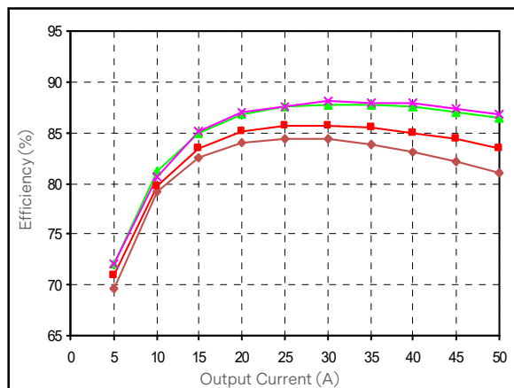
Figure 9: LCM600L Efficiency Curves @ 25 degC, ◆ 90 Vac ■ 115 Vac ▲ 230 Vac ✧ 264 Vac Loading: Vo = 10% increment to 50A, I SR = 0A (5V)
