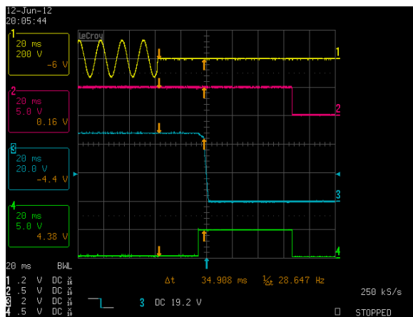
Figure 59: LCM600W Hold-up Time - Vin = 90Vac / 63Hz / 0°
