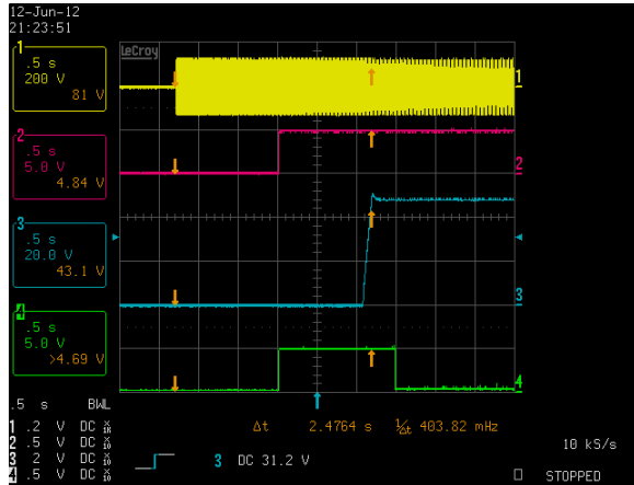
Figure 57: LCM600W Turn-on delay via AC mains - Vin = 90Vac
