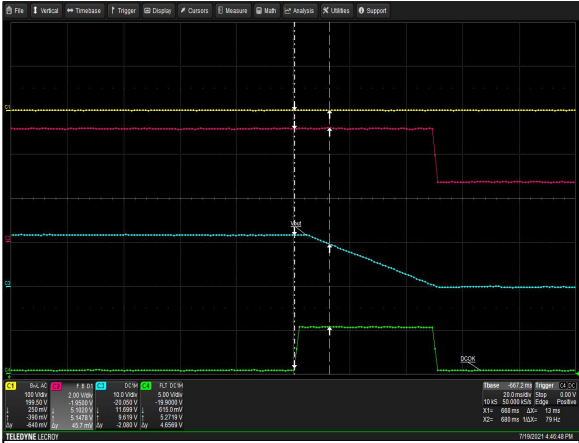
Figure 14: LCM600L DCOK Signal Turn Off Delay – Vin = 100Vac Load: Io = 2A (12V), I SB = 0A (5V) Ch 1: AC Mains Ch 2: ACOK Ch 3: Vo Ch 4: DCOK
