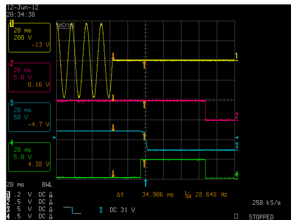
Figure 60: LCM600W Hold-up Time - Vin = 264Vac / 47Hz / 0°
