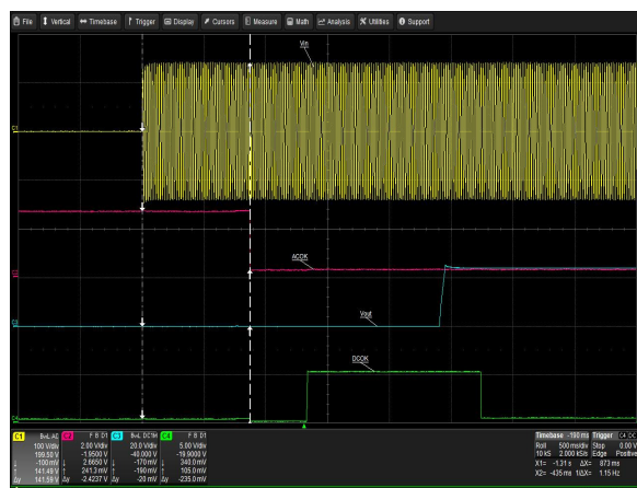
Figure 41: LCM600Q ACOK Signal Turn On Delay – V_{in} = 100V_{ac} Load: I_o = 2A (12V), I_{CP} = 0A (5V)
