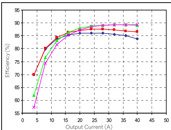
Figure 24: LCM600N Efficiency Curves @ 25 degC, —◆— 90 Vac —■— 115 Vac —▲— 230 Vac Loading: V_o = 10\% increment to 40A, I_{sb} = 0\text{A} (5V)
