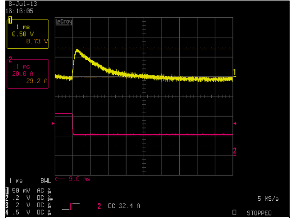
Figure 52: LCM1500U-T-4 Transient Response - V_o Deviation 100% to 50% load change 1A/uS slew rate V_{in} = 230Vac Ch 1: V_o Ch 2: I_o
