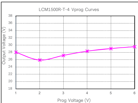
Figure 44: LCM1500R-T-4 Output Voltage Adjustment by Vprog @ 25°C — 115Vac Loading: I_o = 0A (28V), I_{sb} = 0A (5V)
