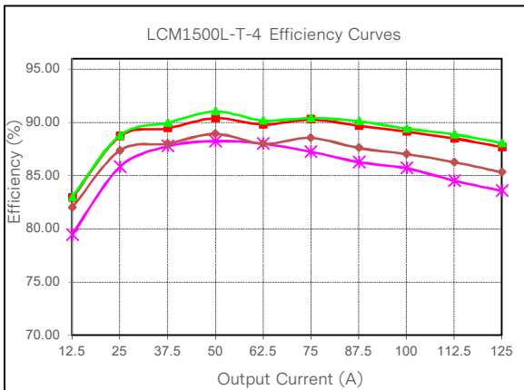
Figure 9: LCM1500L-T-4 Efficiency Curve @ 25°C Loading: I_{o\_main} = 10\%I_{o\_max} increment to 125A, I_{SB} = 0A (5V)
