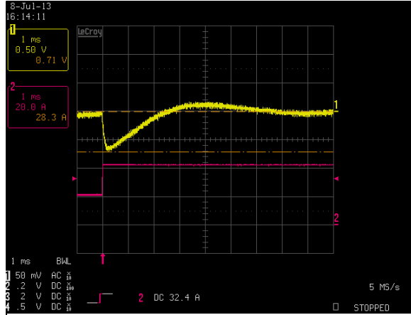
Figure 51: LCM1500U-T-4 Transient Response - V_o Deviation 50% to 100% load change 1A/uS slew rate V_{in} = 230Vac Ch 1: V_o Ch 2: I_o
