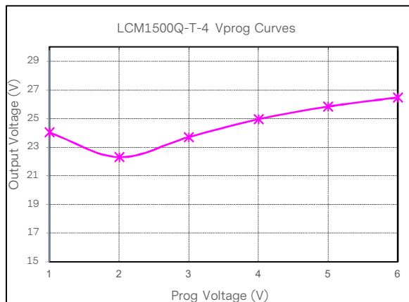
Figure 33: LCM1500Q-T-4 Output Voltage Adjustment by Vprog @ 25°C Loading: I_o = 0A (24V), I_{SB} = 0A (5V)
