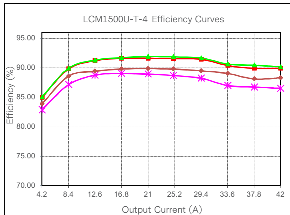
Figure 53: LCM1500U-T-4 Efficiency Curve @ 25°C — 90Vac — 115Vac — 230Vac — 264Vac Loading: I_{o\_main} = 10% I_{o\_max} , increment to 42A, I_{sb} = 0A (5V)
