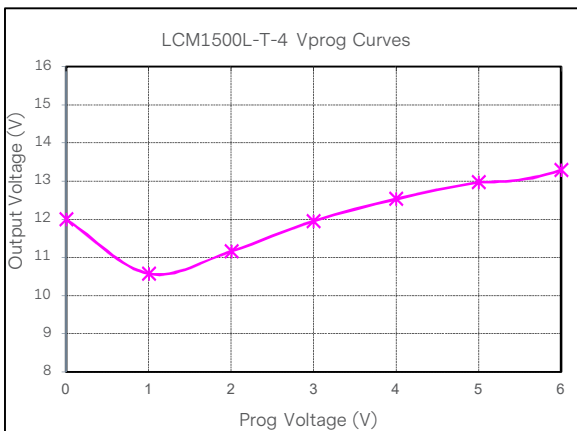
Figure 11: LCM1500L-T-4 Output Voltage Adjustment by Vprog @ 25°C Loading: I_o = 0A (12V), I_{SB} = 0A (5V)
