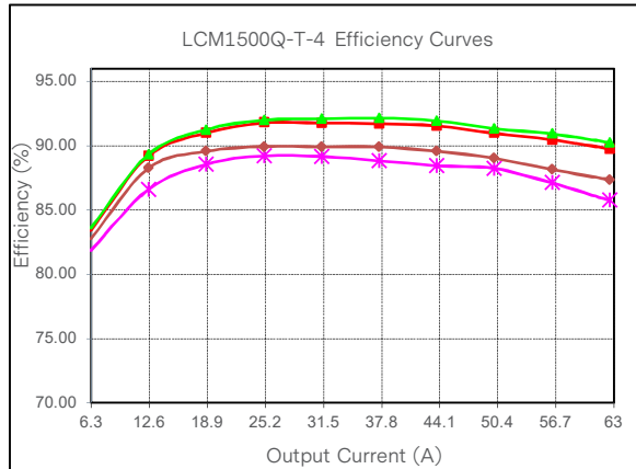
Figure 31: LCM1500Q-T-4 Efficiency Curve @ 25°C Loading: I_{o\_main} = 10\%I_{o\_max} increment to 63A, I_{SB} = 0A (5V)
