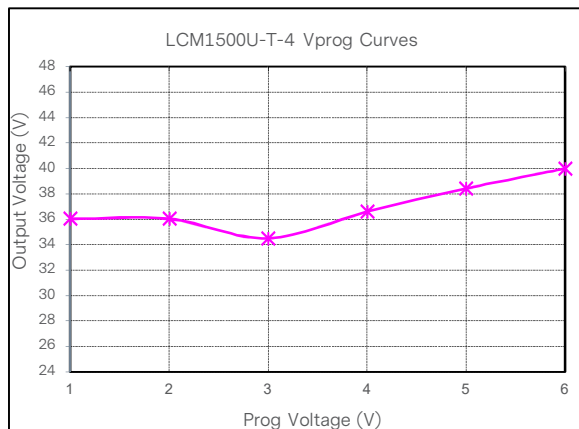
Figure 55: LCM1500U-T-4 Output Voltage Adjustment by V_{prog} @ 25°C — 115Vac Loading: I_o = 0A (36V), I_{sb} = 0A (5V)
