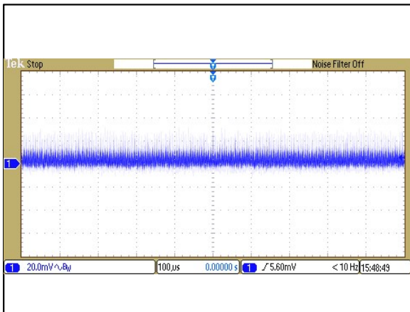
Figure 59: ERM00B36 Ripple and Noise Measurement Vin = 48Vdc Load: Io = 0.83A Ch 1: Vo
