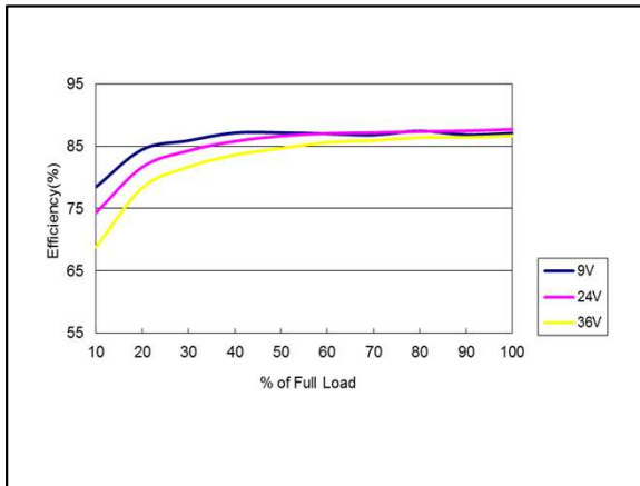
Figure 33: ERM00BB18 Efficiency Versus Output Current Curve Vin = 9 to 36Vdc Load: Io = 0 to ±0.417A
