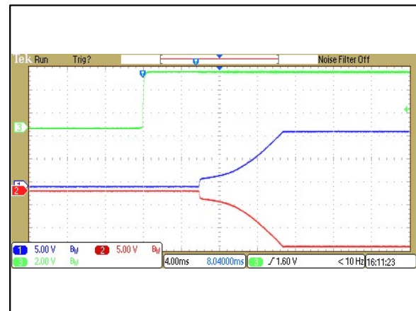
Figure 134: ERM00BB110 Output Voltage Startup Characteristic by V ON/OFF Vin = 110Vdc Load: Io = ±0.417 Ch 1: Vo1 Ch 2: Vo2 Ch 3: V ON/OFF
