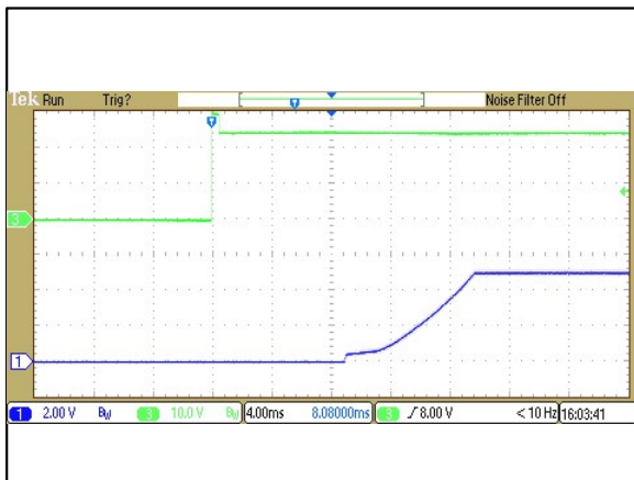
Figure 5: ERM02A18 Output Voltage Startup Characteristic by Vin Vin = 24Vdc Load: Io = 2.0A Ch 1: Vo Ch 3: Vin
