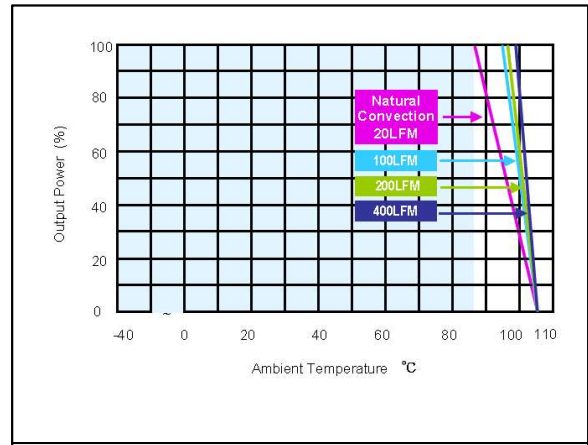
Figure 8: ERM02A18 Derating Output Current vs Ambient Temperature and Airflow (with heatsink) Vin = 24Vdc Load: Io = 0 to 2.0A
