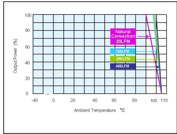
Figure 64: ERM00B36 Derating Output Current vs Ambient Temperature and Airflow (with heatsink) Vin = 48Vdc Load: Io = 0 to 0.83A
