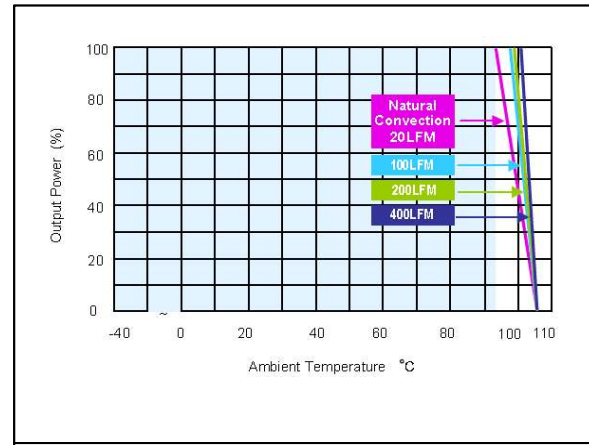
Figure 88: ERM00BB36 Derating Output Current vs Ambient Temperature and Airflow (with heatsink) Vin = 48Vdc Load: Io = 0 to ±0.417A
