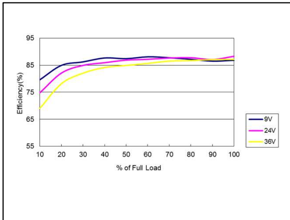
Figure 41: ERM00CC18 Efficiency Versus Output Current Curve Vin = 9 to 36Vdc Load: Io = 0 to ±0.335A
