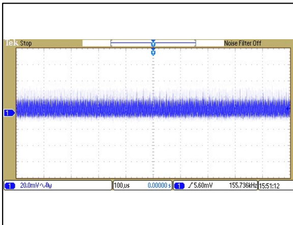
Figure 51: ERM02A36 Ripple and Noise Measurement Vin = 24Vdc Load: Io = 0.835A Ch 1: Vo
