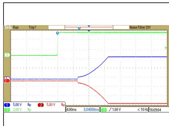
Figure 38: ERM00BB18 Output Voltage Startup Characteristic by VON/OFF Vin = 24Vdc Load: Io = ±0.417A Ch 1: Vo1 Ch 2: Vo2 Ch 3: VON/OFF
