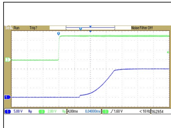
Figure 70: ERM00C36 Output Voltage Startup Characteristic by V_{ON/OFF} Vin = 48Vdc Load: I_o = 0.67A Ch 1: Vo Ch 3: V_{ON/OFF}
