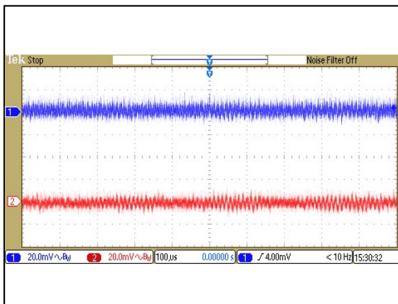
Figure 131: ERM00BB110 Ripple and Noise Measurement Vin = 110Vdc Load: Io = ±0.417A Ch 1: Vo1 Ch 2: Vo2
