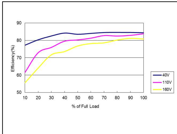
Figure 97: ERM02A110 Efficiency Versus Output Current Curve Vin = 40 to 160Vdc Load: Io = 0 to 0.835A
