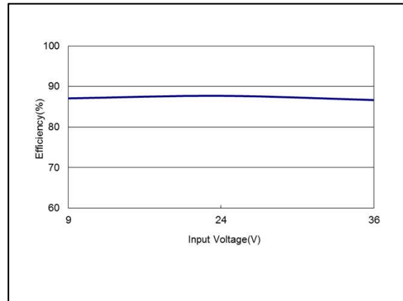
Figure 34: ERM00BB18 Efficiency Versus Input Voltage Curve Vin = 9 to 36Vdc Load: Io = ±0.417A
