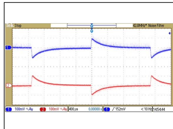
Figure 132: ERM00BB110 Transient Response Vin = 110Vdc Load: Io = 100% to 75% load change Ch 1: Vo1 Ch 2: Vo2
