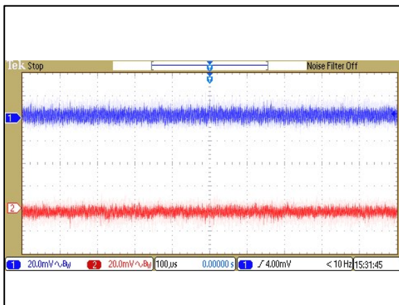
Figure 35: ERM00BB18 Ripple and Noise Measurement Vin = 24Vdc Load: Io = ±0.417A Ch 1: Vo1 Ch 2: Vo2
