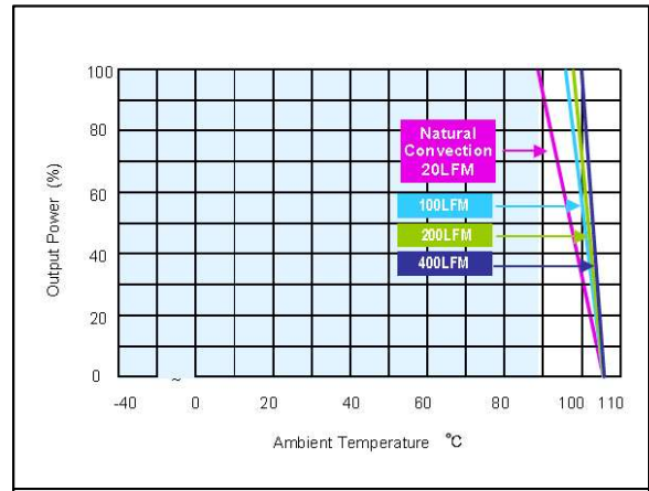
Figure 40: ERM00BB18 Derating Output Current vs Ambient Temperature and Airflow (with heatsink) Vin = 24Vdc Load: Io = 0 to ±0.417A
