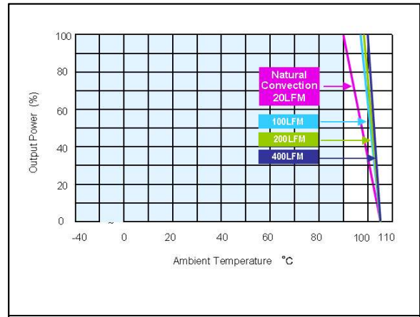
Figure 24: ERM00C18 Derating Output Current vs Ambient Temperature and Airflow (with heatsink) Vin = 24Vdc Load: Io = 0 to 0.67A
