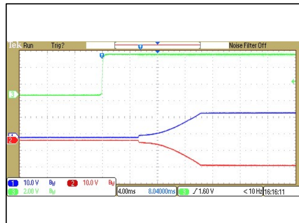
Figure 46: ERM00CC18 Output Voltage Startup Characteristic by VON/OFF Vin = 24Vdc Load: Io = ±0.335A Ch 1: Vo1 Ch 2: Vo2 Ch 3: VON/OFF
