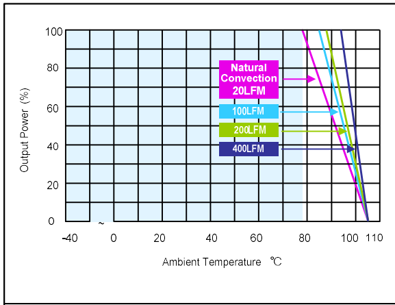
Figure 103: ERM02A110 Derating Output Current vs Ambient Temperature and Airflow (without heatsink) Vin = 110Vdc Load: Io = 0 to 0.835A
