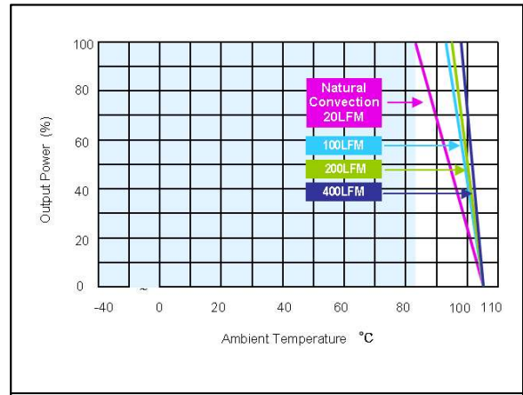
Figure 104: ERM02A110 Derating Output Current vs Ambient Temperature and Airflow (with heatsink) Vin = 110Vdc Load: Io = 0 to 0.835A
