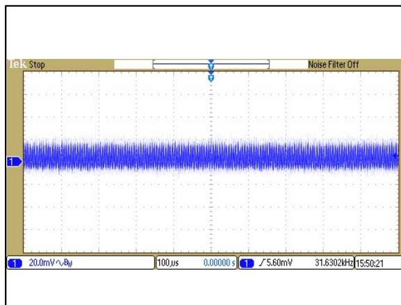
Figure 99: ERM02A110 Ripple and Noise Measurement Vin = 110Vdc Load: Io = 0.835A Ch 1: Vo
