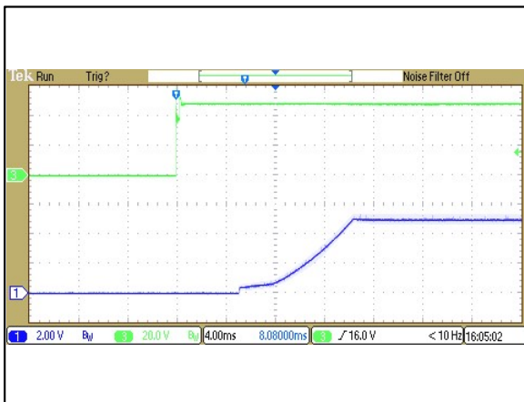
Figure 53: ERM02A36 Output Voltage Startup Characteristic by Vin Vin = 24Vdc Load: Io = 0.835A Ch 1: Vo Ch 3: Vin
