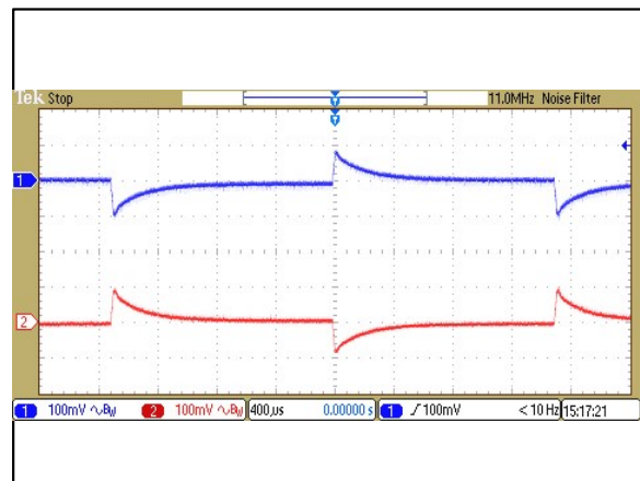
Figure 44: ERM00CC18 Transient Response Vin = 24Vdc Load: Io = 100% to 75% load change Ch 1: Vo1 Ch 2: Vo2
