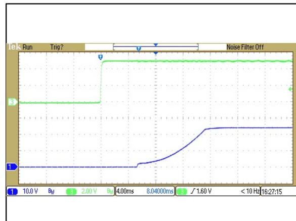
Figure 78: ERM00H36 Output Voltage Startup Characteristic by V_{ON/OFF} Vin = 48Vdc Load: I_o = 0.417A Ch 1: Vo Ch 3: V_{ON/OFF}
