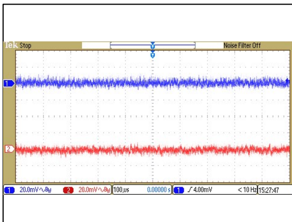
Figure 43: ERM00CC18 Ripple and Noise Measurement Vin = 24Vdc Load: Io = ±0.335A Ch 1: Vo1 Ch 2: Vo2
