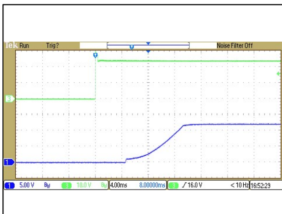
Figure 13: ERM00B18 Output Voltage Startup Characteristic by Vin Vin = 24Vdc Load: I_o = 0.835A Ch 1: Vo Ch 3: Vin
