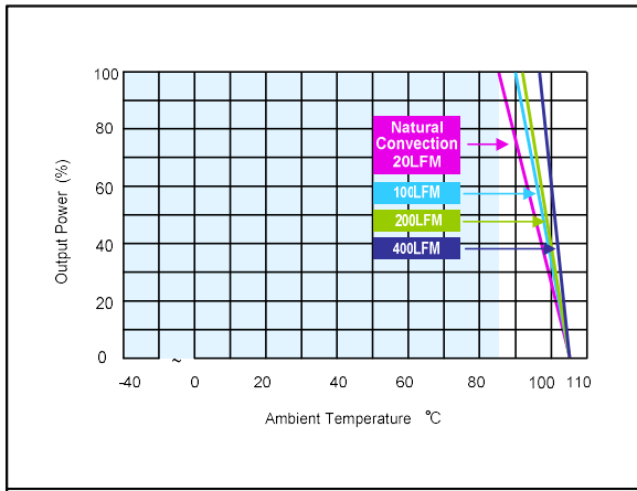
Figure 39: ERM00BB18 Derating Output Current vs Ambient Temperature and Airflow (without heatsink) Vin = 24Vdc Load: Io = 0 to ±0.417A
