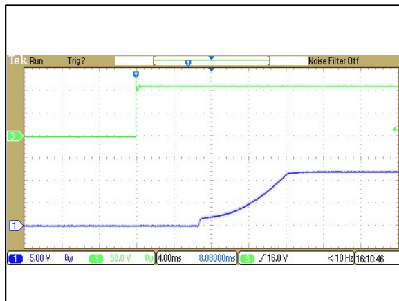
Figure 109: ERM00B110 Output Voltage Startup Characteristic by Vin Vin = 110Vdc Load: Io = 0.83A Ch 1: Vo Ch 3: Vin
