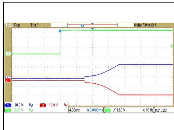
Figure 142: ERM00CC110 Output Voltage Startup Characteristic by VON/OFF Vin = 110Vdc Load: Io = ±0.335A Ch 1: Vo1 Ch 2: Vo2 Ch 3: VON/OFF
