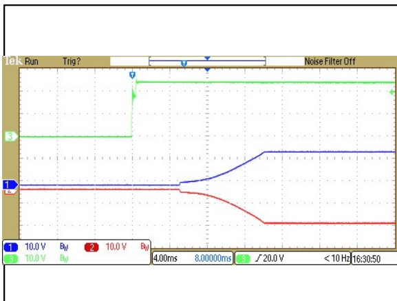
Figure 45: ERM00CC18 Output Voltage Startup Characteristic by Vin Vin = 24Vdc Load: Io = ±0.335A Ch 1: Vo1 Ch 2: Vo2 Ch 3: Vin
