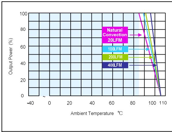
Figure 119: ERM00C110 Derating Output Current vs Ambient Temperature and Airflow (without heatsink) Vin = 110Vdc Load: Io = 0 to 0.417A
