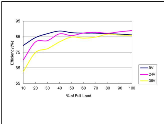
Figure 25: ERM00H18 Efficiency Versus Output Current Curve Vin = 9 to 36Vdc Load: Io = 0 to 0.417A
