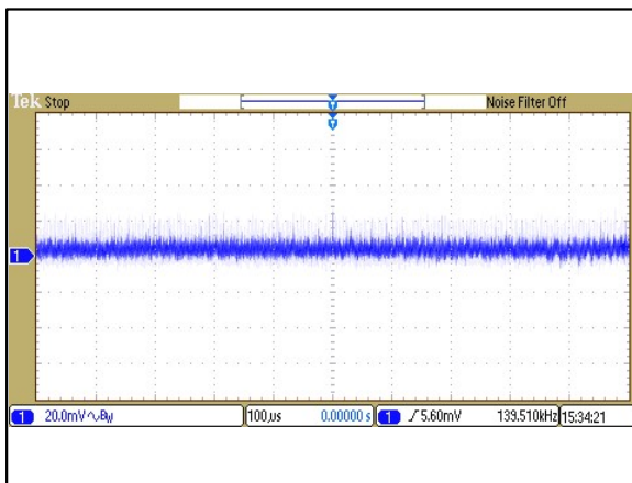
Figure 27: ERM00H18 Ripple and Noise Measurement Vin = 24Vdc Load: Io = 0.417A Ch 1: Vo
