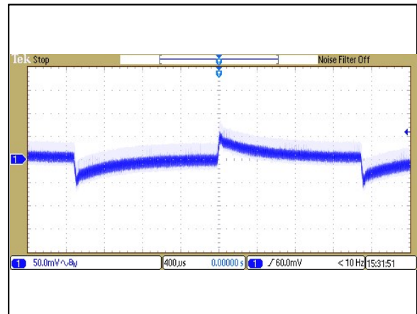
Figure 52: ERM02A36 Transient Response Vin = 24Vdc Load: Io = 100% to 75% load change Ch 1: Vo
