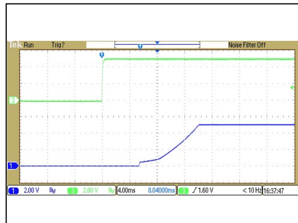
Figure 6: ERM02A18 Output Voltage Startup Characteristic by VON/OFF Vin = 24Vdc Load: Io = 2.0A Ch 1: Vo Ch 3: VON/OFF
