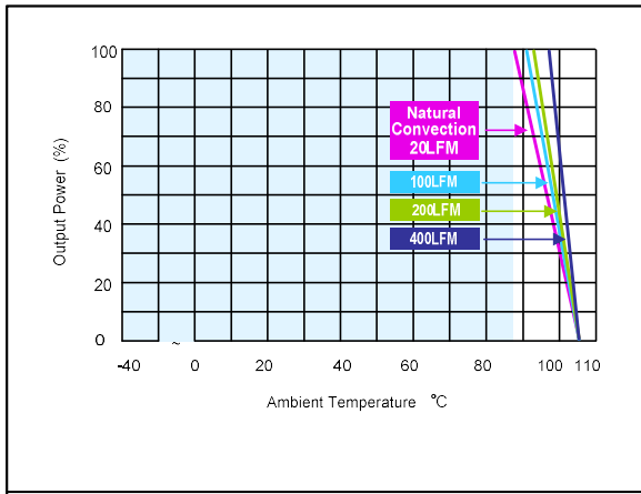
Figure 23: ERM00C18 Derating Output Current vs Ambient Temperature and Airflow (without heatsink) Vin = 24Vdc Load: Io = 0 to 0.67A
