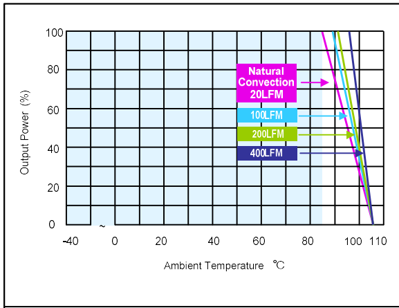
Figure 111: ERM00B110 Derating Output Current vs Ambient Temperature and Airflow (without heatsink) Vin = 110Vdc Load: Io = 0 to 0.83A
