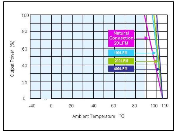
Figure 56: ERM02A36 Derating Output Current vs Ambient Temperature and Airflow (with heatsink) Vin = 24Vdc Load: Io = 0 to 0.835A
