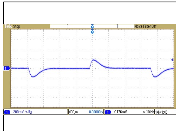
Figure 76: ERM00H36 Transient Response Vin = 48Vdc Load: I_o = 100\% to 75% load change Ch 1: Vo
