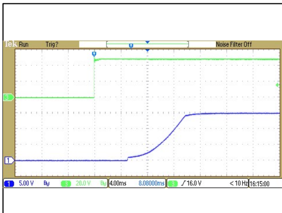
Figure 69: ERM00C36 Output Voltage Startup Characteristic by Vin Vin = 48Vdc Load: I_o = 0.67A Ch 1: Vo Ch 3: Vin
