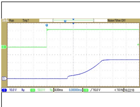
Figure 125: ERM00H110 Output Voltage Startup Characteristic by Vin Vin = 110Vdc Load: Io = 0.417A Ch 1: Vo Ch 3: Vin
