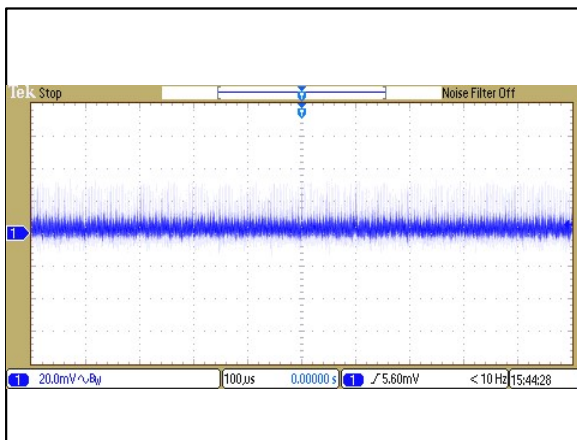
Figure 67: ERM00C36 Ripple and Noise Measurement Vin = 48Vdc Load: I_o = 0.67A Ch 1: Vo
