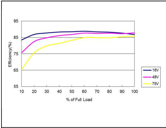
Figure 57: ERM00B36 Efficiency Versus Output Current Curve Vin = 18 to 75Vdc Load: Io = 0 to 0.83A
