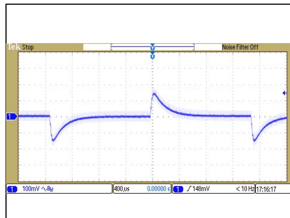
Figure 12: ERM00B18 Transient Response Vin = 24Vdc Load: I_o = 100\% to 75% load change Ch 1: Vo
