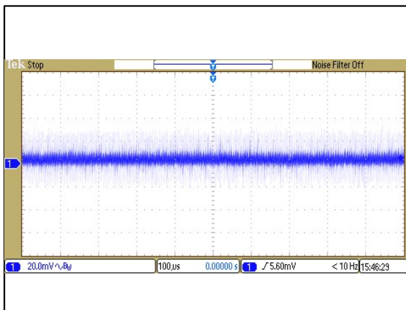
Figure 11: ERM00B18 Ripple and Noise Measurement Vin = 24Vdc Load: I_o = 0.835A Ch 1: Vo
