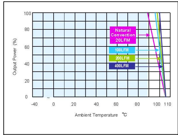
Figure 80: ERM00H36 Derating Output Current vs Ambient Temperature and Airflow (with heatsink) Vin = 48Vdc Load: Io = 0 to 0.417A
