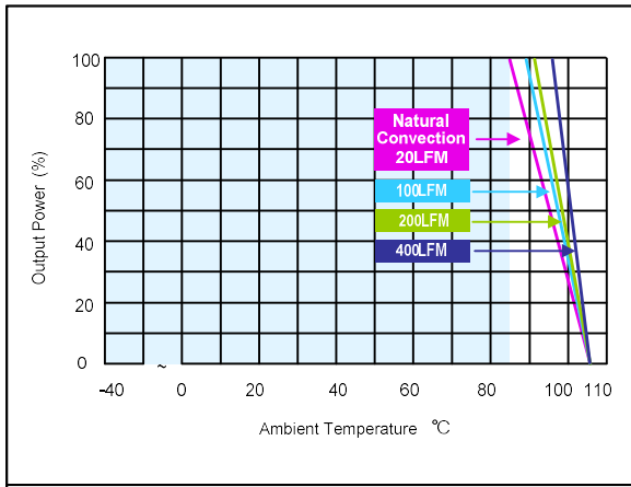
Figure 55: ERM02A36 Derating Output Current vs Ambient Temperature and Airflow (without heatsink) Vin = 24Vdc Load: Io = 0 to 0.835A
