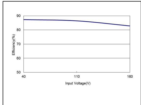
Figure 114: ERM00C110 Efficiency Versus Input Voltage Curve Vin = 40 to 160Vdc Load: Io = 0.417A
