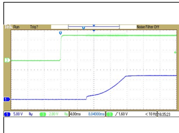
Figure 110: ERM00B110 Output Voltage Startup Characteristic by V ON/OFF Vin = 110Vdc Load: Io = 0.83A Ch 1: Vo Ch 3: V ON/OFF
