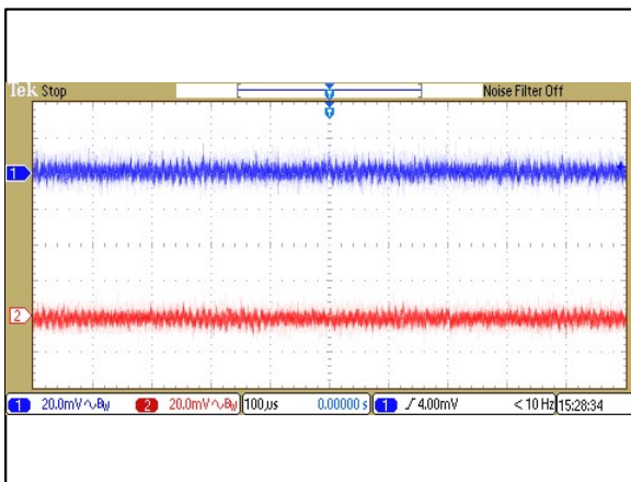
Figure 91: ERM00CC36 Ripple and Noise Measurement Vin = 48Vdc Load: Io = ±0.335A Ch 1: Vo1 Ch 2: Vo2
