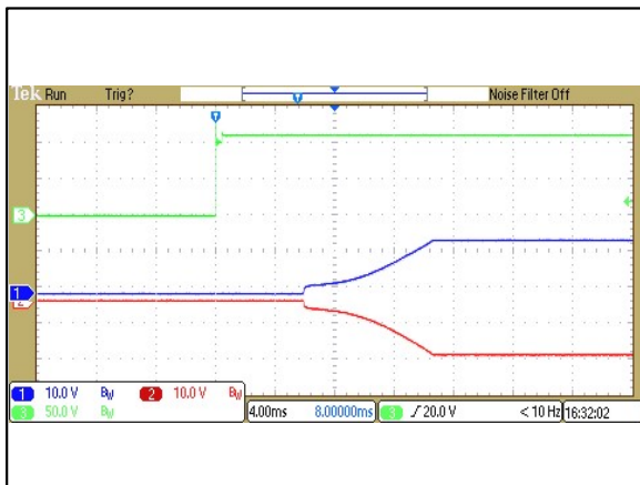
Figure 141: ERM00CC110 Output Voltage Startup Characteristic by Vin Vin = 110Vdc Load: Io = ±0.335A Ch 1: Vo1 Ch 2: Vo2 Ch 3: Vin
