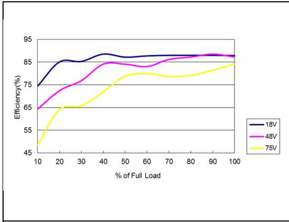
Figure 73: ERM00H36 Efficiency Versus Output Current Curve Vin = 18 to 75Vdc Load: I_o = 0 to 0.417A
