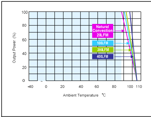
Figure 63: ERM00B36 Derating Output Current vs Ambient Temperature and Airflow (without heatsink) Vin = 48Vdc Load: Io = 0 to 0.83A
