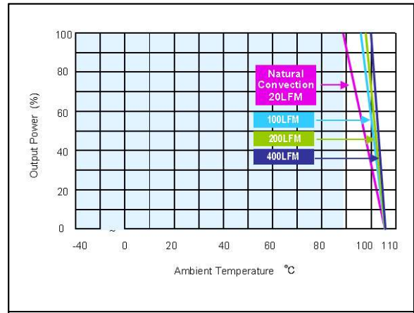
Figure 144: ERM00CC110 Derating Output Current vs Ambient Temperature and Airflow (with heatsink) Vin = 110Vdc Load: Io = 0 to ±0.335A
