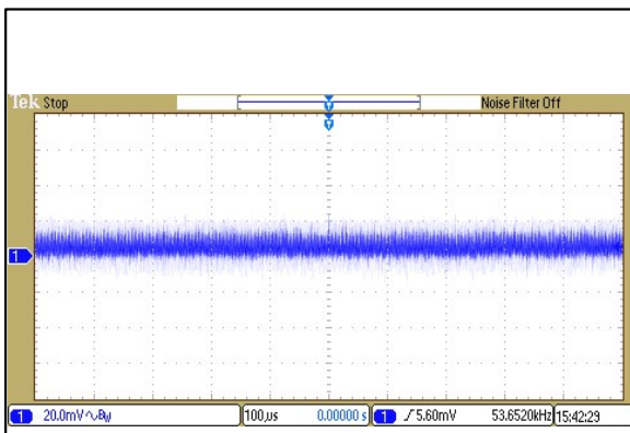
Figure 115: ERM00C110 Ripple and Noise Measurement Vin = 110Vdc Load: Io = 0.417A Ch 1: Vo
