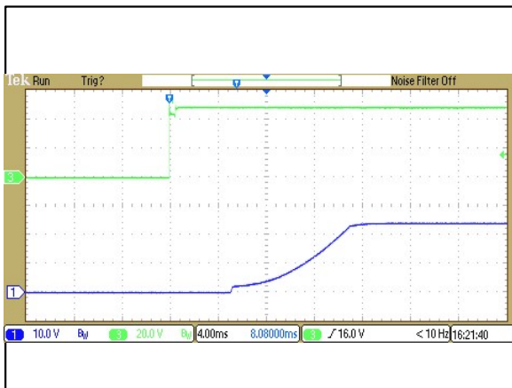
Figure 77: ERM00H36 Output Voltage Startup Characteristic by Vin Vin = 48Vdc Load: I_o = 0.417A Ch 1: Vo Ch 3: Vin
