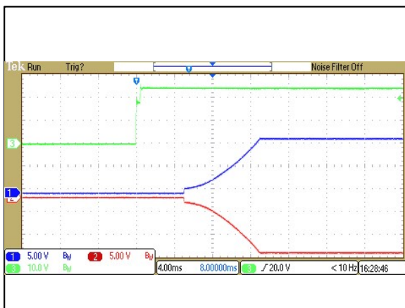
Figure 37: ERM00BB18 Output Voltage Startup Characteristic by Vin Vin = 24Vdc Load: Io = ±0.417A Ch 1: Vo1 Ch 2: Vo2 Ch 3: Vin
