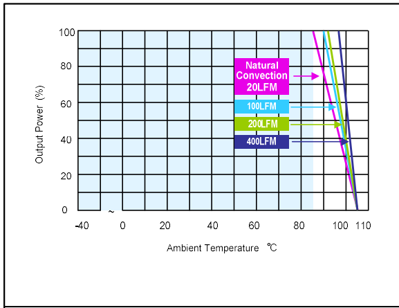
Figure 143: ERM00CC110 Derating Output Current vs Ambient Temperature and Airflow (without heatsink) Vin = 110Vdc Load: Io = 0 to ±0.335A
