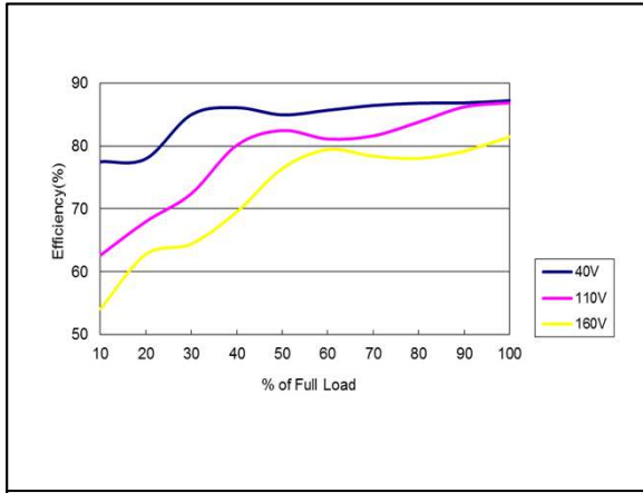
Figure 137: ERM00CC110 Efficiency Versus Output Current Curve Vin = 40 to 160Vdc Load: Io = 0 to ±0.335A
