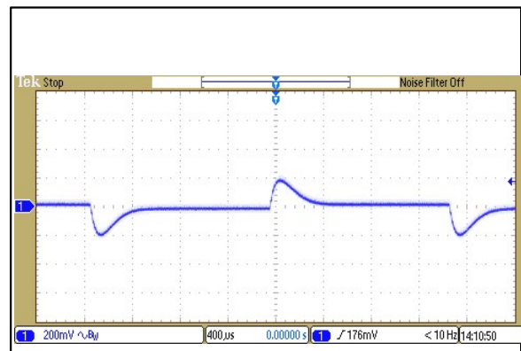
Figure 116: ERM00C110 Transient Response Vin = 110Vdc Load: Io = 100% to 75% load change Ch 1: Vo
