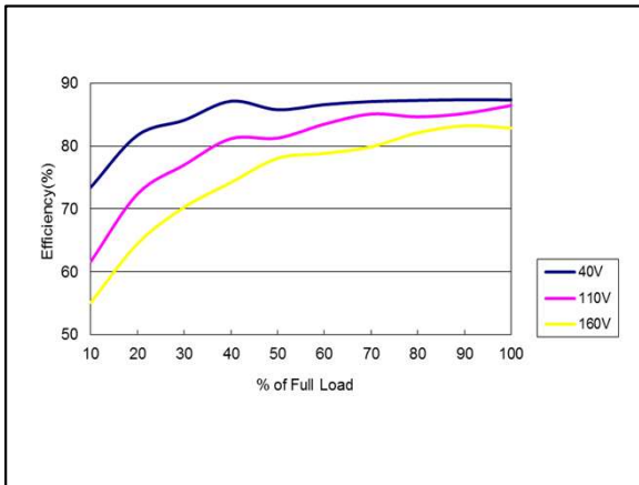
Figure 113: ERM00C110 Efficiency Versus Output Current Curve Vin = 40 to 160Vdc Load: Io = 0 to 0.417A
