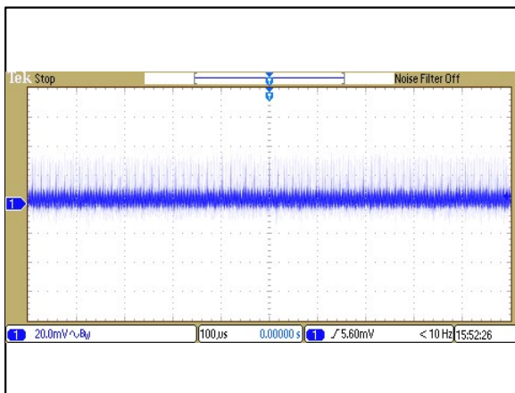
Figure 3: ERM02A18 Ripple and Noise Measurement Vin = 24Vdc Load: Io = 2.0A Ch 1: Vo
