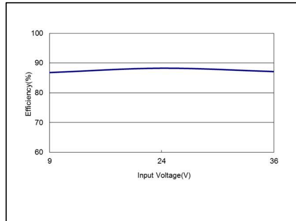
Figure 42: ERM00CC18 Efficiency Versus Input Voltage Curve Vin = 9 to 36Vdc Load: Io = ±0.335A
