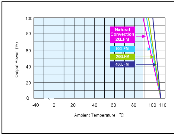
Figure 31: ERM00H18 Derating Output Current vs Ambient Temperature and Airflow (without heatsink) Vin = 24Vdc Load: Io = 0 to 0.417A
