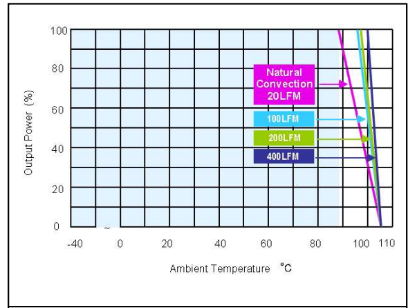
Figure 128: ERM00H110 Derating Output Current vs Ambient Temperature and Airflow (with heatsink) Vin = 110Vdc Load: Io = 0 to 0.417A
