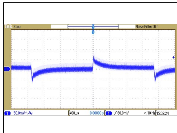
Figure 4: ERM02A18 Transient Response Vin = 24Vdc Load: Io = 100% to 75% load change Ch 1: Vo
