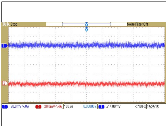
Figure 139: ERM00CC110 Ripple and Noise Measurement Vin = 110Vdc Load: Io = ±0.335A Ch 1: Vo1 Ch 2: Vo2
