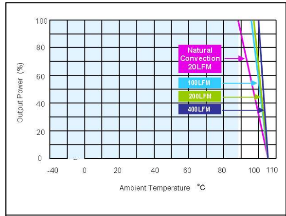
Figure 112: ERM00B110 Derating Output Current vs Ambient Temperature and Airflow (with heatsink) Vin = 110Vdc Load: Io = 0 to 0.83A
