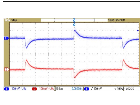
Figure 140: ERM00CC110 Transient Response Vin = 110Vdc Load: Io = 100% to 75% load change Ch 1: Vo1 Ch 2: Vo2
