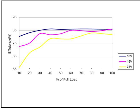
Figure 49: ERM02A36 Efficiency Versus Output Current Curve Vin = 9 to 36Vdc Load: Io = 0 to 0.835A
