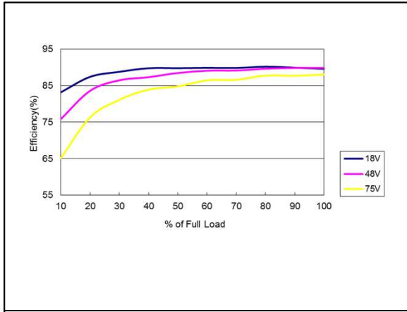
Figure 81: ERM00BB36 Efficiency Versus Output Current Curve Vin = 18 to 75Vdc Load: Io = 0 to ±0.417A
