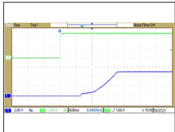
Figure 54: ERM02A36 Output Voltage Startup Characteristic by VON/OFF Vin = 24Vdc Load: Io = 0.835A Ch 1: Vo Ch 3: VON/OFF
