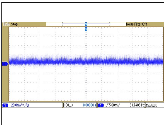
Figure 123: ERM00H110 Ripple and Noise Measurement Vin = 110Vdc Load: Io = 0.417A Ch 1: Vo
