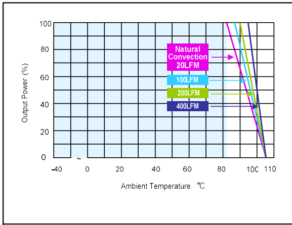
Figure 7: ERM02A18 Derating Output Current vs Ambient Temperature and Airflow (without heatsink) Vin = 24Vdc Load: Io = 0 to 2.0A
