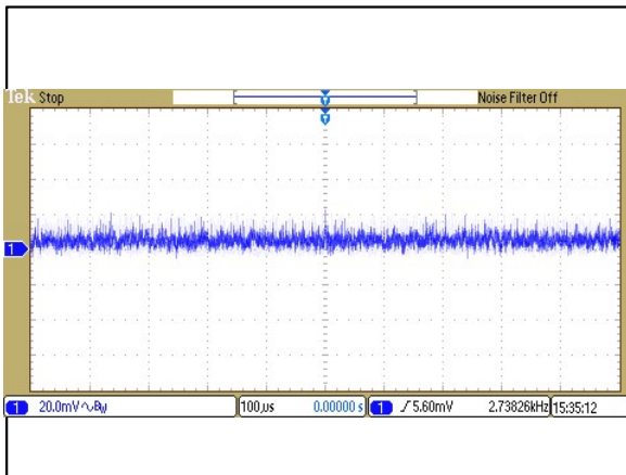
Figure 75: ERM00H36 Ripple and Noise Measurement Vin = 48Vdc Load: I_o = 0.417A Ch 1: Vo
