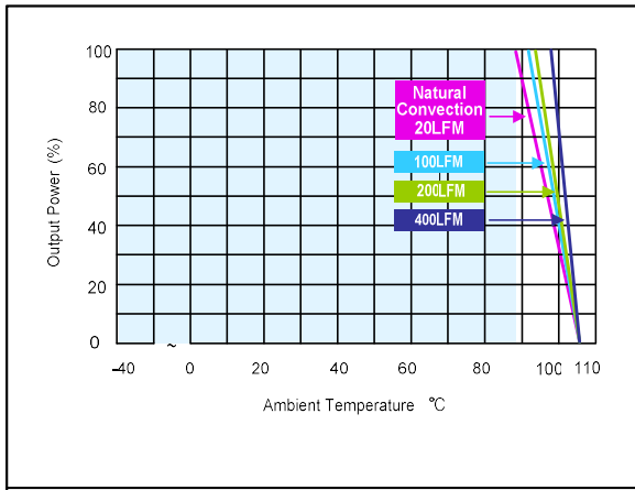
Figure 95: ERM00CC36 Derating Output Current vs Ambient Temperature and Airflow (without heatsink) Vin = 48Vdc Load: Io = 0 to ±0.335A
