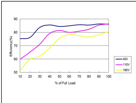
Figure 121: ERM00H110 Efficiency Versus Output Current Curve Vin = 40 to 160Vdc Load: Io = 0 to 0.417A
