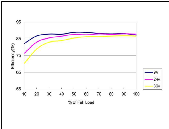
Figure 9: ERM00B18 Efficiency Versus Output Current Curve Vin = 9 to 36Vdc Load: I_o = 0 to 0.835A
