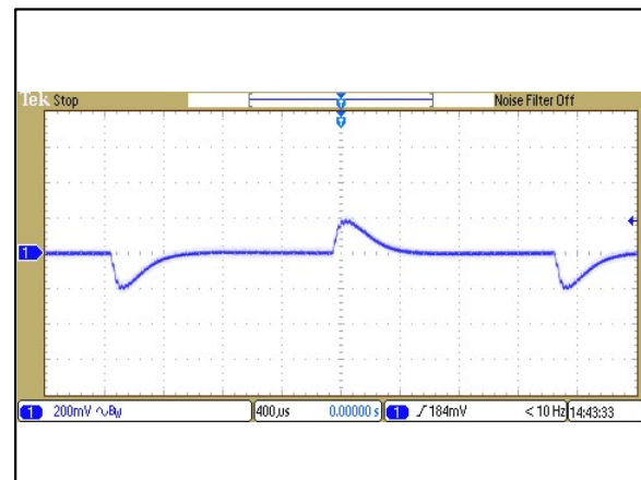
Figure 28: ERM00H18 Transient Response Vin = 24Vdc Load: Io = 100% to 75% load change Ch 1: Vo
