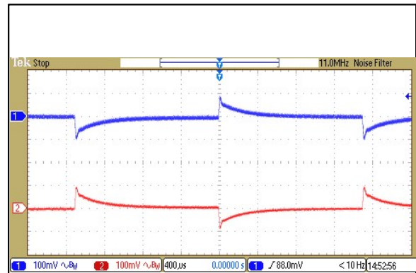
Figure 84: ERM00BB36 Transient Response Vin = 48Vdc Load: Io = 100% to 75% load change Ch 1: Vo1 Ch 2: Vo2
