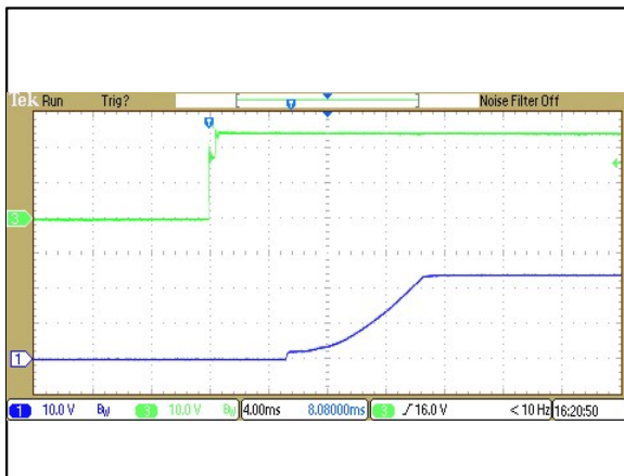
Figure 29: ERM00H18 Output Voltage Startup Characteristic by Vin Vin = 24Vdc Load: Io = 0.417A Ch 1: Vo Ch 3: Vin
