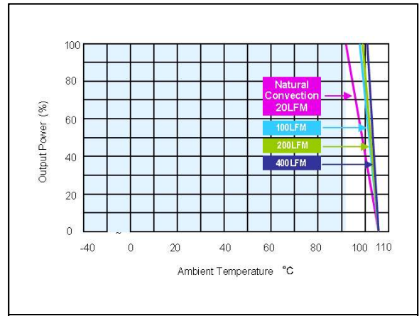
Figure 32: ERM00H18 Derating Output Current vs Ambient Temperature and Airflow (with heatsink) Vin = 24Vdc Load: Io = 0 to 0.417A
