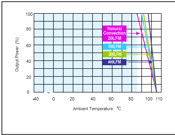
Figure 135: ERM00BB110 Derating Output Current vs Ambient Temperature and Airflow (without heatsink) Vin = 110Vdc Load: Io = 0 to ±0.417A
