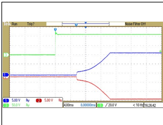
Figure 133: ERM00BB110 Output Voltage Startup Characteristic by Vin Vin = 110Vdc Load: Io = ±0.417A Ch 1: Vo1 Ch 2: Vo2 Ch 3: Vin
