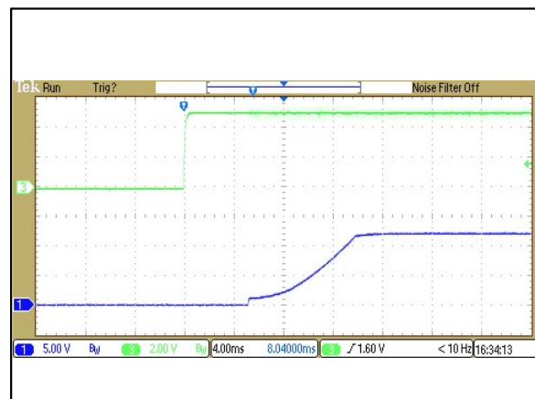
Figure 14: ERM00B18 Output Voltage Startup Characteristic by V_{ON/OFF} Vin = 24Vdc Load: I_o = 0.835A Ch 1: Vo Ch 3: V_{ON/OFF}
