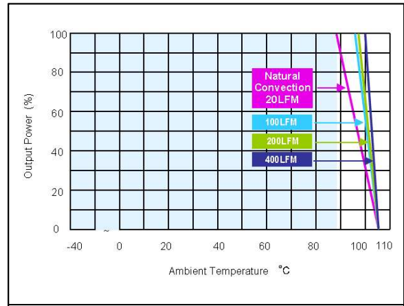
Figure 120: ERM00C110 Derating Output Current vs Ambient Temperature and Airflow (with heatsink) Vin = 110Vdc Load: Io = 0 to 0.417A
