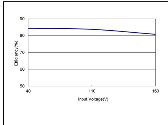
Figure 98: ERM02A110 Efficiency Versus Input Voltage Curve Vin = 40 to 160Vdc Load: Io = 0.835A
