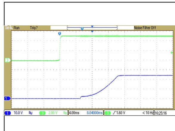
Figure 30: ERM00H18 Output Voltage Startup Characteristic by V ON/OFF Vin = 24Vdc Load: Io = 0.417A Ch 1: Vo Ch 3: V ON/OFF
