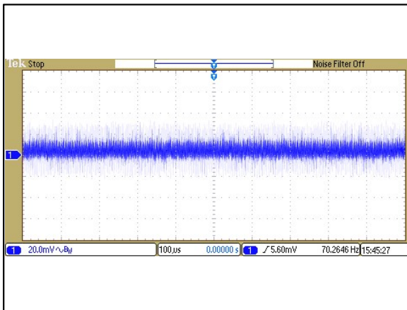
Figure 19: ERM00C18 Ripple and Noise Measurement Vin = 24Vdc Load: Io = 0.67A Ch 1: Vo
