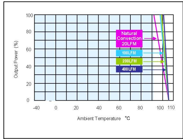
Figure 96: ERM00CC36 Derating Output Current vs Ambient Temperature and Airflow (with heatsink) Vin = 48Vdc Load: Io = 0 to ±0.335A
