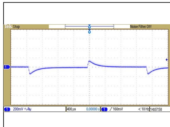
Figure 68: ERM00C36 Transient Response Vin = 48Vdc Load: I_o = 100\% to 75% load change Ch 1: Vo
