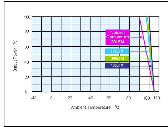
Figure 72: ERM00C36 Derating Output Current vs Ambient Temperature and Airflow (with heatsink) Vin = 48Vdc Load: Io = 0 to 0.67A
