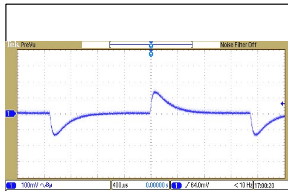
Figure 108: ERM00B110 Transient Response Vin = 110Vdc Load: Io = 100% to 75% load change Ch 1: Vo
