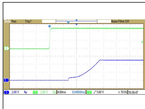
Figure 102: ERM02A110 Output Voltage Startup Characteristic by V ON/OFF Vin = 110Vdc Load: Io = 0.835A Ch 1: Vo Ch 3: V ON/OFF
