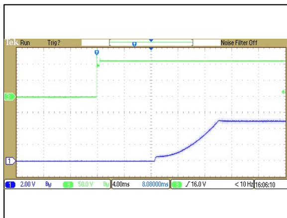
Figure 101: ERM02A110 Output Voltage Startup Characteristic by Vin Vin = 110Vdc Load: Io = 0.835A Ch 1: Vo Ch 3: Vin
