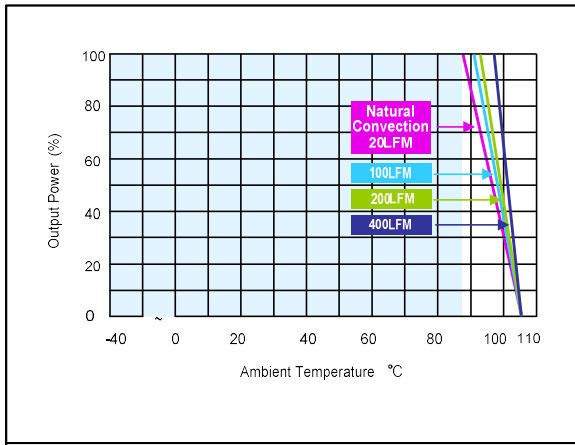
Figure 71: ERM00C36 Derating Output Current vs Ambient Temperature and Airflow (without heatsink) Vin = 48Vdc Load: Io = 0 to 0.67A
