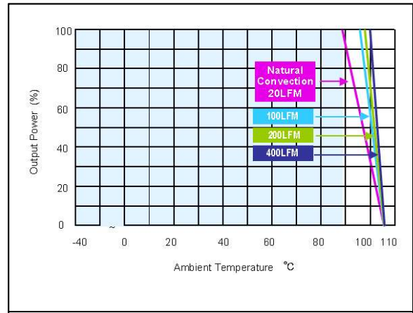
Figure 136: ERM00BB110 Derating Output Current vs Ambient Temperature and Airflow (with heatsink) Vin = 110Vdc Load: Io = 0 to ±0.417A
