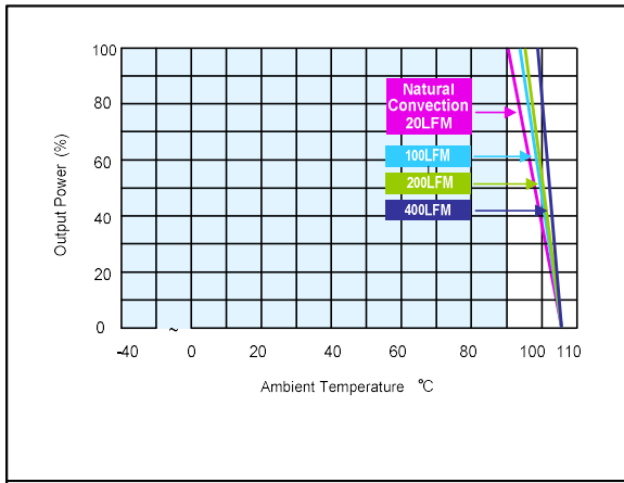
Figure 87: ERM00BB36 Derating Output Current vs Ambient Temperature and Airflow (without heatsink) Vin = 48Vdc Load: Io = 0 to ±0.417A
