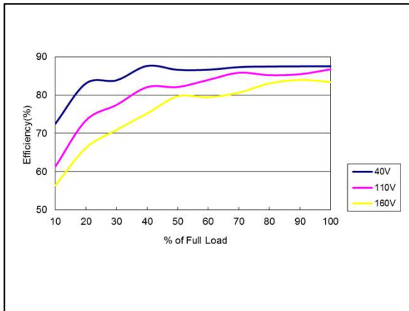
Figure 129: ERM00BB110 Efficiency Versus Output Current Curve Vin = 40 to 160Vdc Load: Io = 0 to ±0.417A
