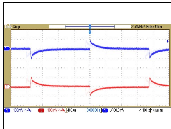
Figure 36: ERM00BB18 Transient Response Vin = 24Vdc Load: Io = 100% to 75% load change Ch 1: Vo1 Ch 2: Vo2
