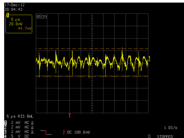
Figure 6: LPT101-M Ripple and Noise Measurement
