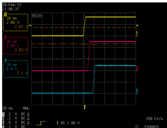
Figure 5: LPT101-M Output Voltage Startup Characteristic
