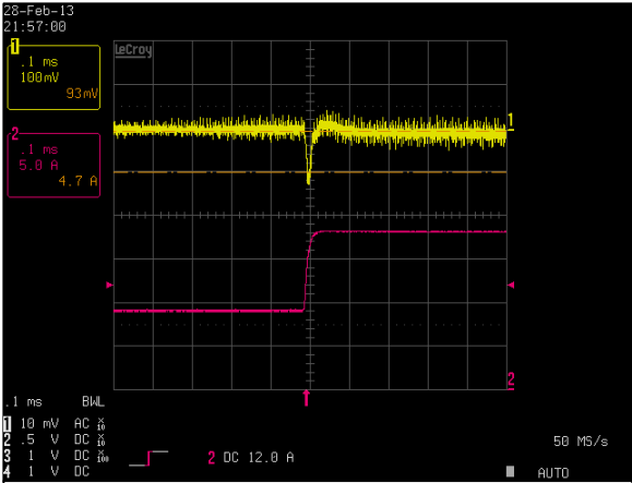
Figure 18: LPT102-M Transient Response – Vo Deviation Vin = 90Vac Load: Io = 50% to 100%, 1A/us slew rate Ch 1: 5.0V Ch 2: Io
