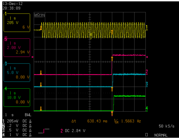
Figure 1: LPT101-M Turn-on delay
