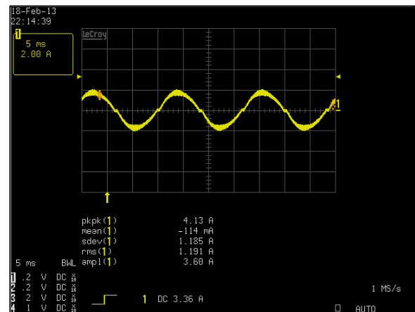
Figure 4: LPT101-M Input Current Waveform
