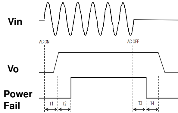
Power Fail signal timing diagram
