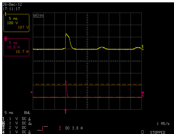
Figure 3: LPT101-M Inrush Current
