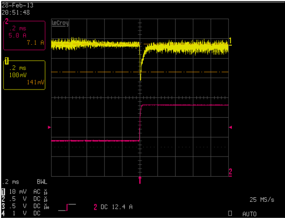
Figure 8: LPT101-M Transient Response – Vo Deviation Vin = 90Vac Load: Io = 50% to 100%, 1A/us slew rate Ch 1: 3.3V Ch 2: Io
