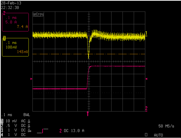
Figure 28: LPT103-M Transient Response – Vo Deviation Vin = 90Vac Load: Io = 50% to 100%, 1A/us slew rate Ch 1: 5.0V Ch 2: Io
