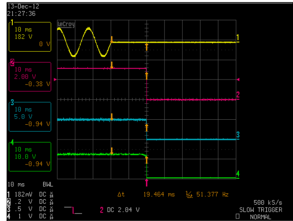
Figure 2: LPT101-M Hold-up Time (time to decay)
