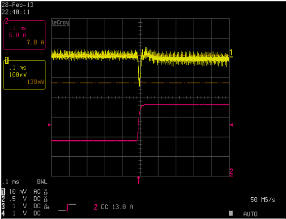
Figure 38: LPT104-M Transient Response – Vo Deviation Vin = 90Vac Load: Io = 50% to 100%, 1A/us slew rate Ch 1: 5.0V Ch 2: Io
