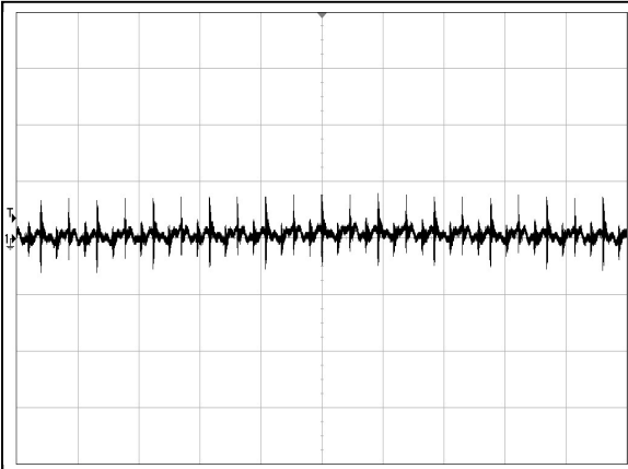
Figure 1: AVD75-48S1V2 Input Reflected Ripple Current Waveform Ch 1: Iin (5 \mu S/div, 10mA/div)
