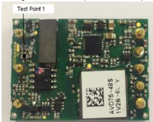
Figure 15 Temperature test point(Bottom)
