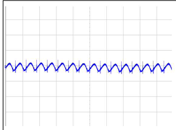
Figure 2: AVO100-48S05 Ripple and Noise Measurement Ch 1: V o (5uS/div, 50mV/div)
