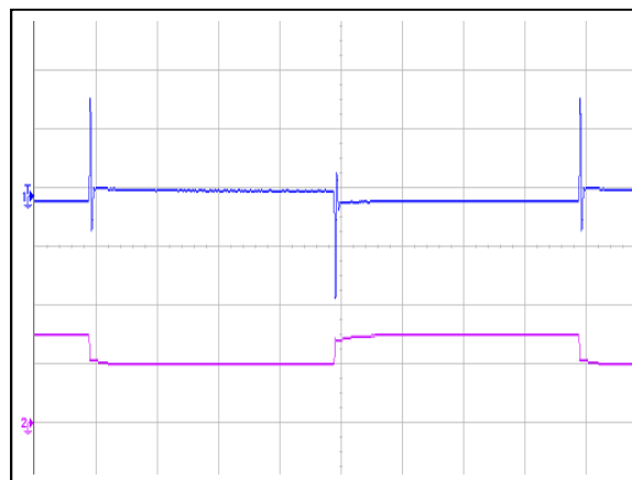
Figure 8: AVO100-48S05 Transient Response (1mS/div) 50%~75%~50% load change, 1A/uS slew rate, Vin = 48Vdc Ch 1: Vo (100mV/div) Ch 3: Io (10A/div)
