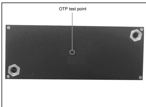
Figure 11: AVO100-48S05B OTP Test Point
