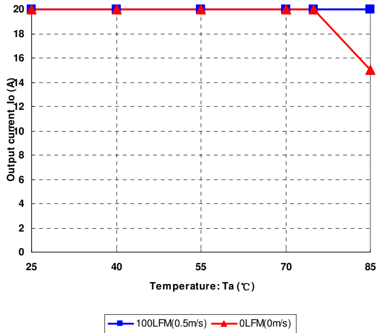
Figure 16 Derating curve
