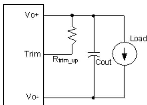
Figure 20 Trim up
