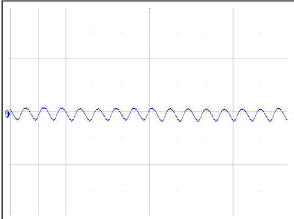
Figure 1: AVO100-48S05 Input Reflected Ripple Current Waveform Ch 1: I in (5uS/div, 10mA/div)
