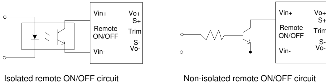
Figure 19 External Remote ON/OFF circuit
