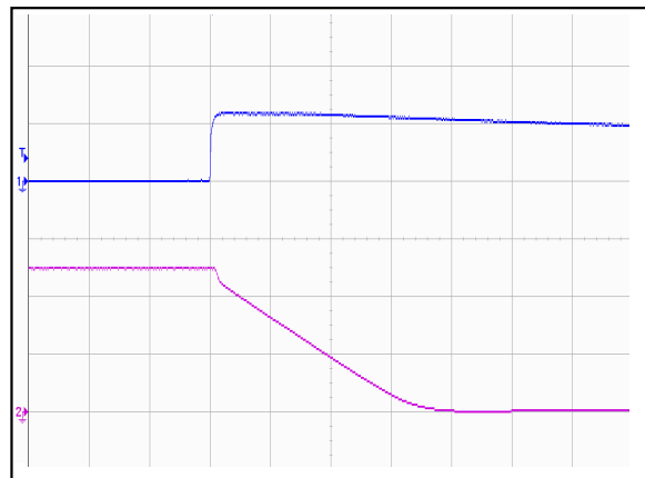
Figure 6: AVO100-48S05 Remote OFF Waveform (100uS/div) Ch 1: Remote OFF (5V/div) CH3: V o (2V/div)
