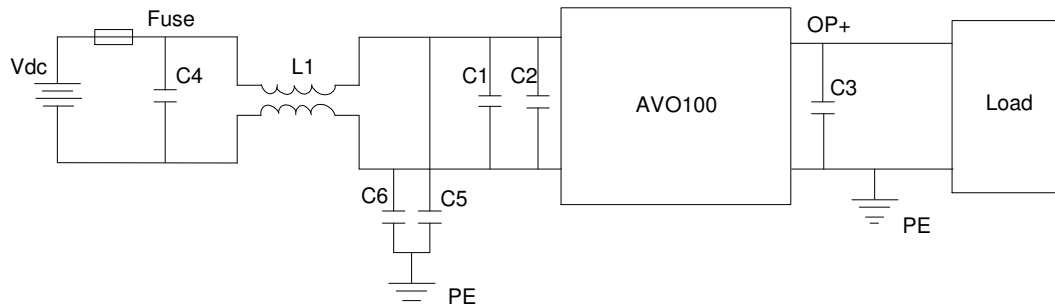
Figure 18 Typical application
