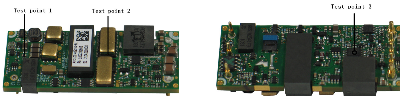
Figure 10 Temperature test point
