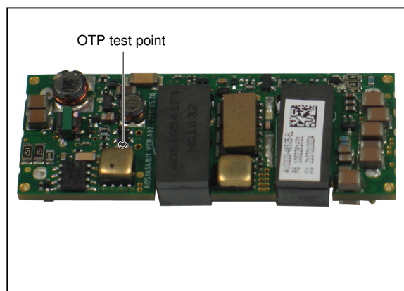
Figure 10: AVO100-48S05 OTP Test Point
