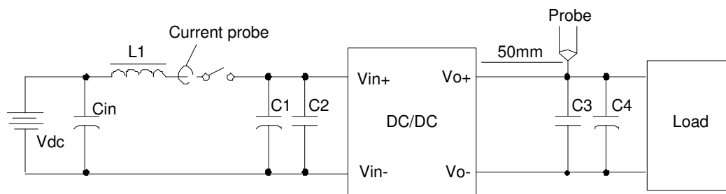
Figure 22 Input ripple & inrush current output ripple & noise test configuration
