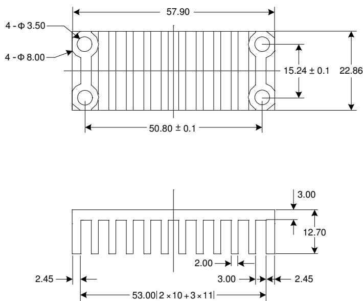
Figure 15 Heatsink (Unit:mm)
