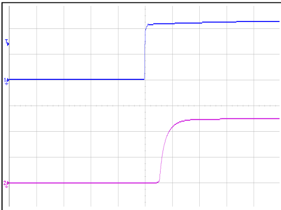
Figure 3: AVO100-48S05 Output Voltage Startup Characteristic (5mS/div) Ch 1: V in (20V/div) Ch 2: V o (2V/div)
