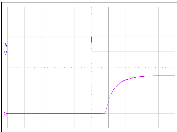
Figure 5: AVO100-48S05 Remote ON Waveform (2mS/div) Ch 1: Remote ON (5V/div) Ch 3: V o (2V/div)
