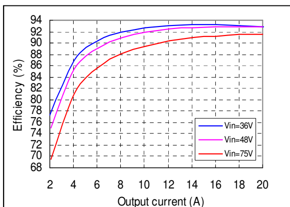
Figure 9: AVO100-48S05 Efficiency Curves @ 25 °C
