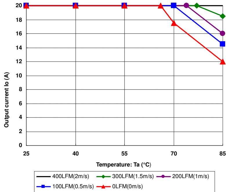
Figure 12 Derating curve
