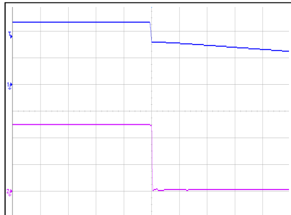
Figure 4: AVO100-48S05 Turn Off Characteristic (10mS/div) Ch 1: V in (20V/div) Ch 2: V o (2V/div)
