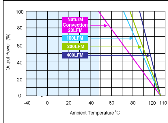
Figure 71: ERM03H110 Derating Curves (with heatsink) Vin = 110Vdc Load: Io = 0 to 3.125A
