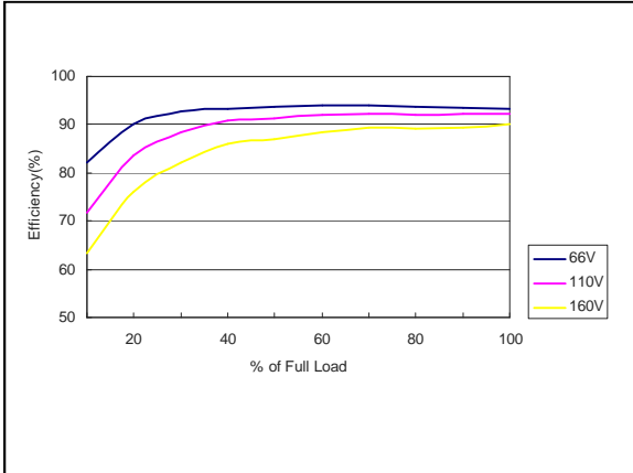
Figure 55: ERM05C110 Efficiency Versus Output Current Curve Vin = 66 to 160Vdc Load: Io = 0 to 5.0A
