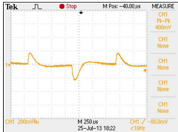
Figure 13: ERM06B72 Transient Response Vin = 72Vdc Load: Io = 100% to 75% load change Ch 1: Vo
