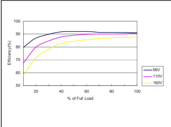
Figure 64: ERM03H110 Efficiency Versus Output Current Curve Vin = 66 to 160Vdc Load: Io = 0 to 3.125A
