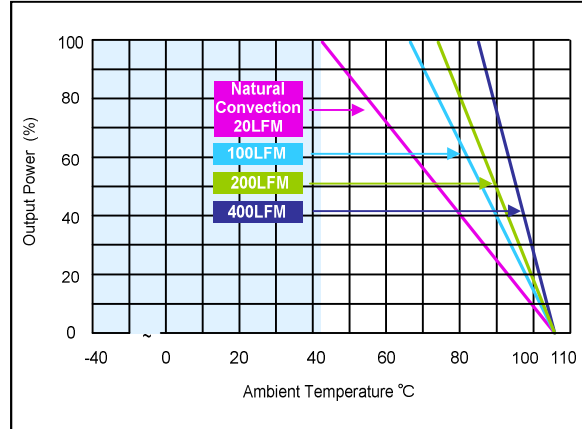
Figure 44: ERM15A110 Derating Curves (with heatsink) Vin = 110Vdc Load: Io = 0 to 15.0A
