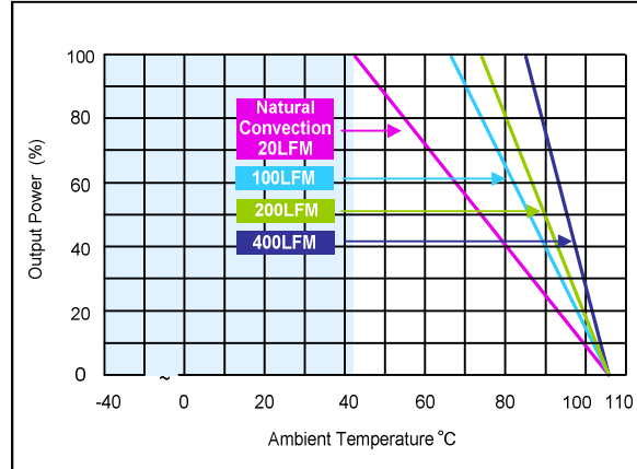
Figure 8: ERM15A72 Derating Curves (with heatsink) Vin = 72Vdc Load: Io = 0 to 15.0A
