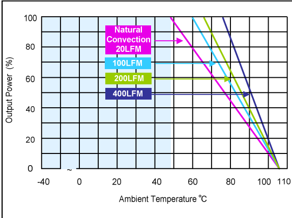
Figure 34: ERM03H72 Derating Curves (without heatsink) Vin = 72Vdc Load: Io = 0 to 3.125A
