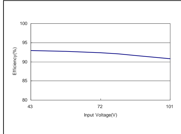
Figure 20: ERM05C72 Efficiency Versus Input Voltage Curve Vin = 43 to 101Vdc Load: Io = 5.0A
