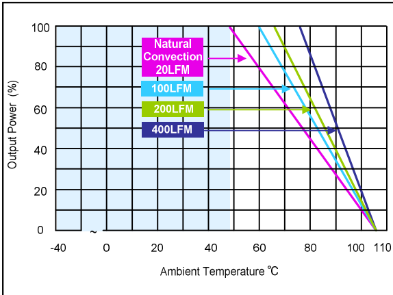
Figure 61: ERM05C110 Derating Curves (without heatsink) Vin = 110Vdc Load: Io = 0 to 5.0A
