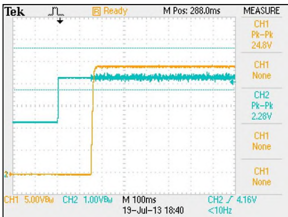
Figure 32: ERM03H72 Output Voltage Startup Characteristic by ON/OFF Vin = 72Vdc Load: Io = 3.125A Ch1: Vo Ch2: Remote On/Off
