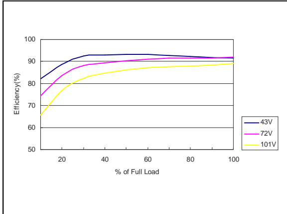
Figure 28: ERM03H72 Efficiency Versus Output Current Curve Vin = 43 to 101Vdc Load: Io = 0 to 3.125A
