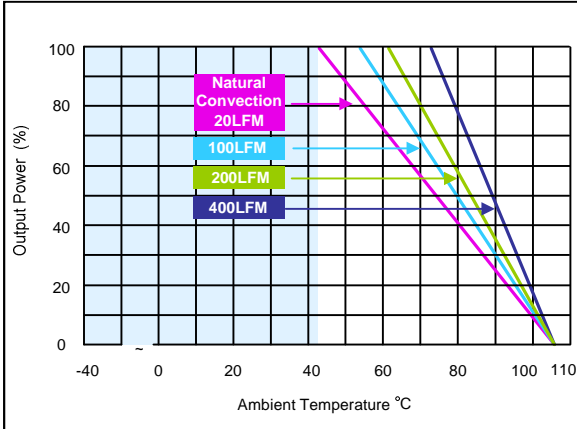
Figure 70: ERM03H110 Derating Curves (without heatsink) Vin = 110Vdc Load: Io = 0 to 3.125A
