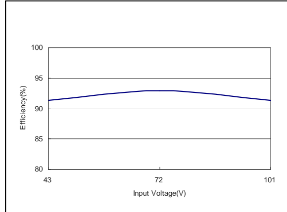
Figure 11: ERM06B72 Efficiency Versus Input Voltage Curve Vin = 43 to 101Vdc Load: Io = 6.25A
