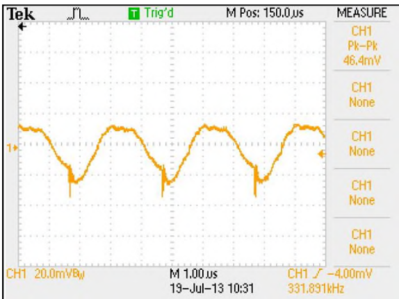
Figure 39: ERM15A110 Ripple and Noise Measurement Vin = 110Vdc Load: Io = 15.0A Ch 1: Vo
