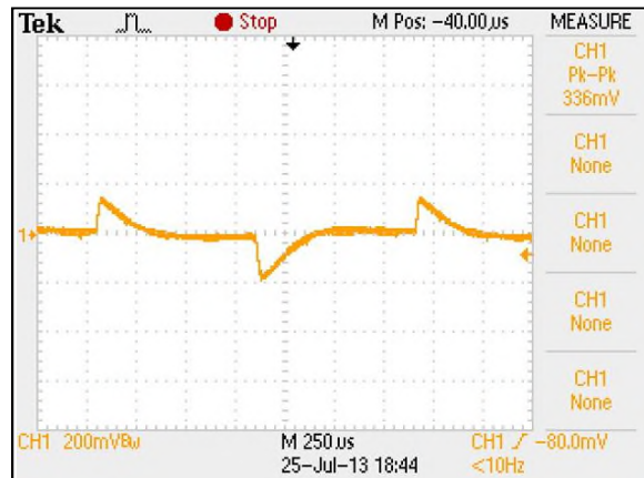
Figure 40: ERM15A110 Transient Response Vin = 110Vdc Load: Io = 100% to 75% load change Ch 1: Vo
