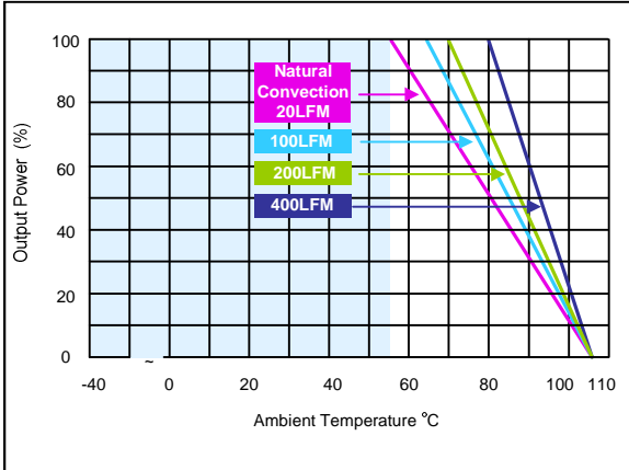
Figure 25: ERM05C72 Derating Curves (without heatsink) Vin = 72Vdc Load: Io = 0 to 5.0A
