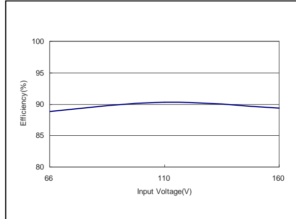
Figure 38: ERM15A110 Efficiency Versus Input Voltage Curve Vin = 66 to 160Vdc Load: Io = 15.0A
