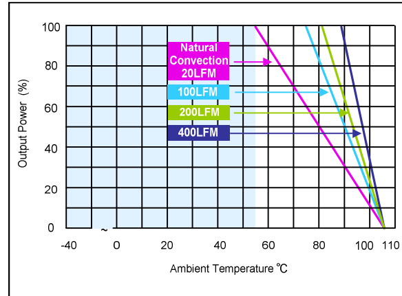
Figure 62: ERM05C110 Derating Curves (with heatsink) Vin = 110Vdc Load: Io = 0 to 5.0A
