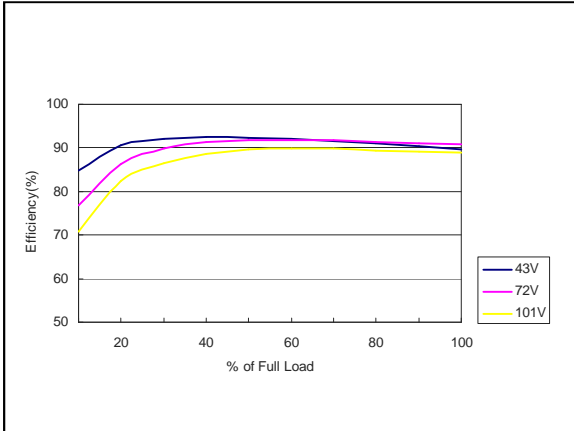
Figure 1: ERM15A72 Efficiency Versus Output Current Curve Vin = 43 to 101Vdc Load: Io = 0 to 15.0A
