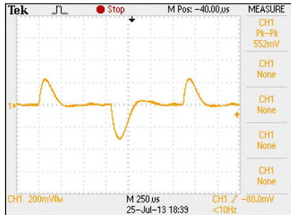
Figure 58: ERM05C110 Transient Response Vin = 110Vdc Load: Io = 100% to 75% load change Ch 1: Vo
