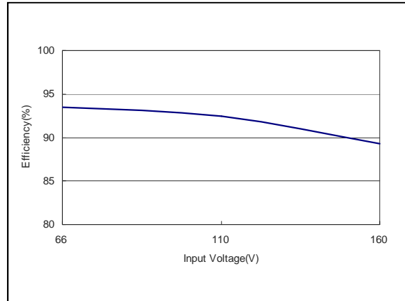
Figure 47: ERM06B110 Efficiency Versus Input Voltage Curve Vin = 66 to 160Vdc Load: Io = 6.25A
