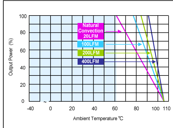
Figure 17: ERM06B72 Derating Curves (with heatsink) Vin = 72Vdc Load: Io = 0 to 6.25A
