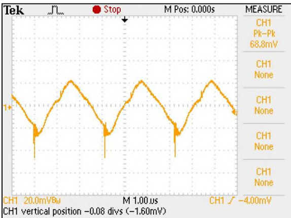
Figure 3: ERM15A72 Ripple and Noise Measurement Vin = 72Vdc Load: Io = 15.0A Ch 1: Vo
