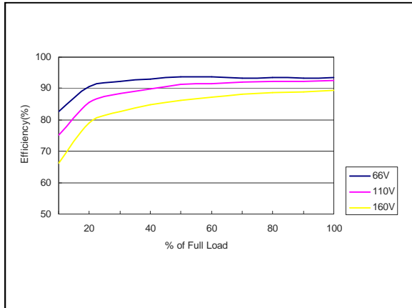
Figure 46: ERM06B110 Efficiency Versus Output Current Curve Vin = 66 to 160Vdc Load: Io = 0 to 6.25A
