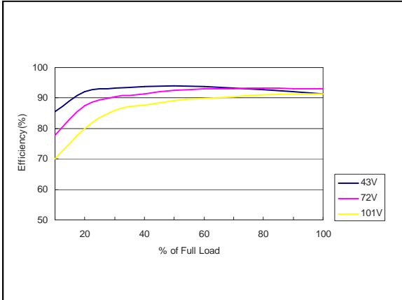
Figure 10: ERM06B72 Efficiency Versus Output Current Curve Vin = 43 to 101Vdc Load: Io = 0 to 6.25A
