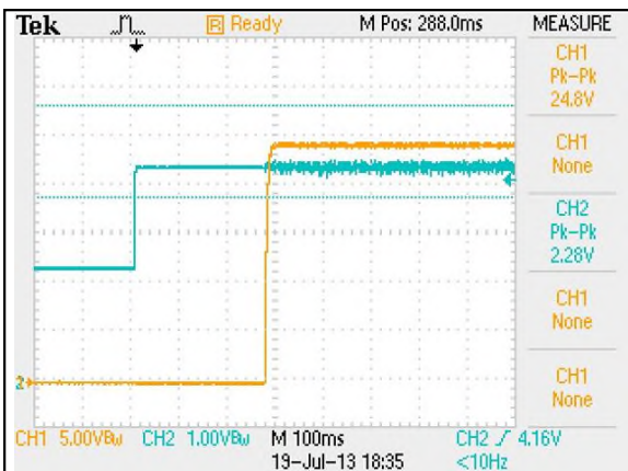
Figure 68: ERM03H110 Output Voltage Startup Characteristic by ON/OFF Vin = 110Vdc Load: Io = 3.125A Ch1: Vo Ch2: Remote On/Off
