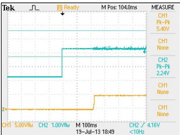
Figure 5: ERM15A72 Output Voltage Startup Characteristic by ON/OFF Vin = 72Vdc Load: Io = 15.0A Ch1: Vo Ch2: Remote On/Off
