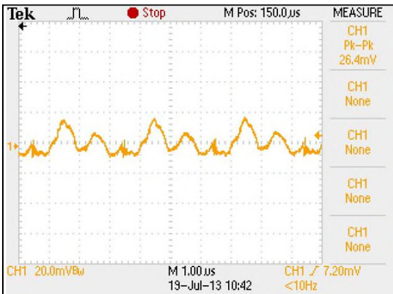
Figure 57: ERM05C110 Ripple and Noise Measurement Vin = 110Vdc Load: Io = 5.0A Ch 1: Vo
