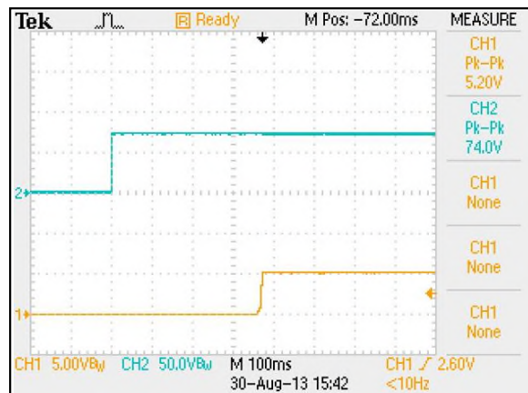
Figure 6: ERM15A72 Output Voltage Startup Characteristic by Vin Vin = 72Vdc Load: Io = 15.0A Ch1: Vo Ch2: Vin
