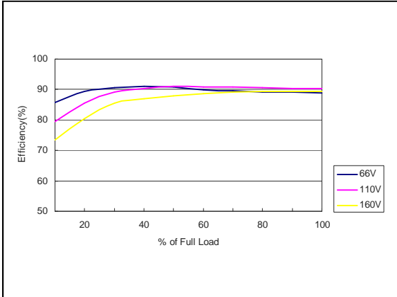
Figure 37: ERM15A110 Efficiency Versus Output Current Curve Vin = 66 to 160Vdc Load: Io = 0 to 15.0A
