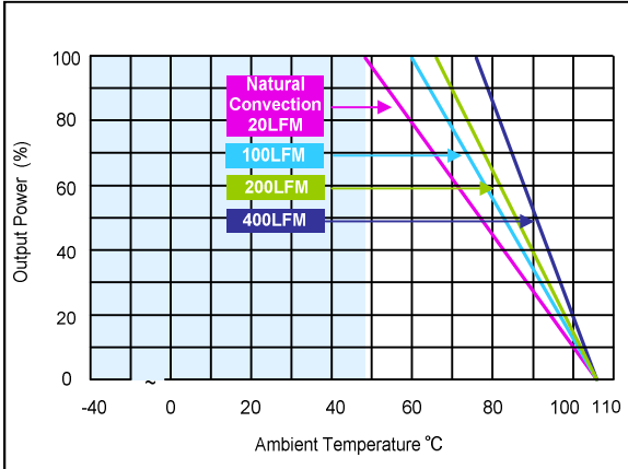
Figure 52: ERM06B110 Derating Curves (without heatsink) Vin = 110Vdc Load: Io = 0 to 6.25A
