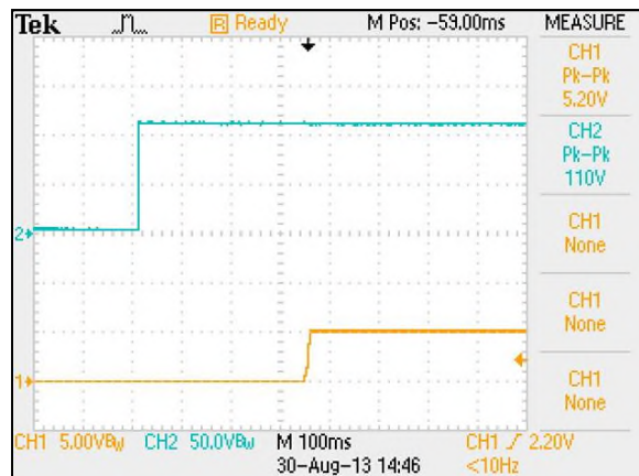
Figure 42: ERM15A110 Output Voltage Startup Characteristic by Vin Vin = 110Vdc Load: Io = 15.0A Ch1: Vo Ch2: Vin
