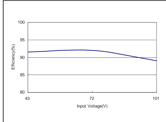
Figure 29: ERM03H72 Efficiency Versus Input Voltage Curve Vin = 43 to 101Vdc Load: Io = 3.125A
