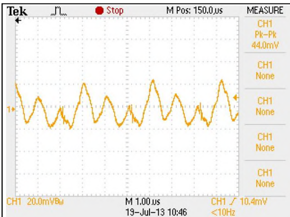
Figure 66: ERM03H110 Ripple and Noise Measurement Vin = 110Vdc Load: Io = 3.125A Ch 1: Vo
