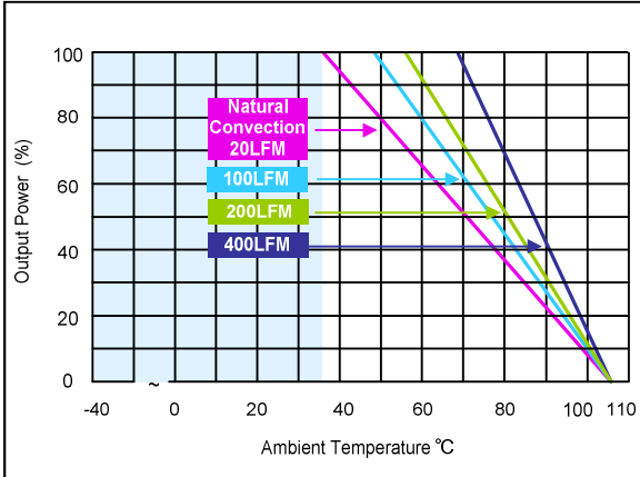
Figure 7: ERM15A72 Derating Curves (without heatsink) Vin = 72Vdc Load: Io = 0 to 15.0A
