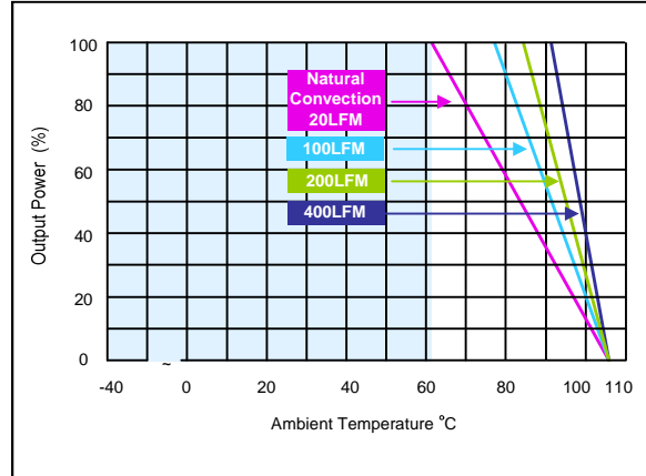
Figure 26: ERM05C72 Derating Curves (with heatsink) Vin = 72Vdc Load: Io = 0 to 5.0A
