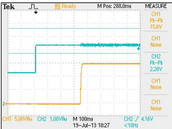
Figure 59: ERM05C110 Output Voltage Startup Characteristic by ON/OFF Vin = 110Vdc Load: Io = 5.0A Ch1: Vo Ch2: Remote On/Off
