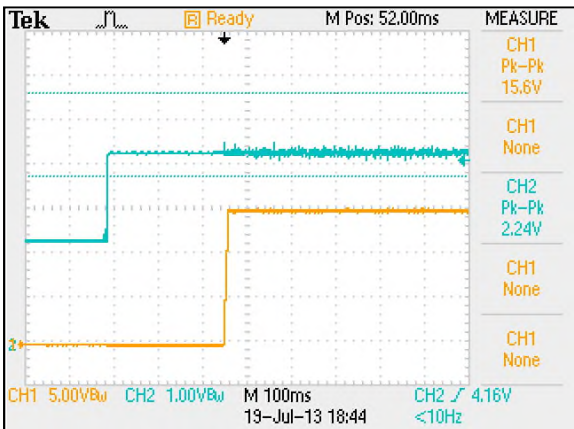
Figure 21: ERM05C72 Ripple and Noise Measurement Vin = 72Vdc Load: Io = 5.0A Ch 1: Vo
