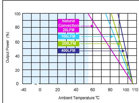
Figure 53: ERM06B110 Derating Curves (with heatsink) Vin = 110Vdc Load: Io = 0 to 6.25A
