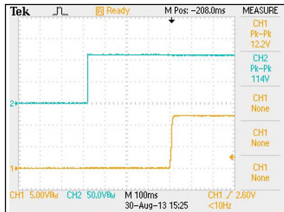
Figure 51: ERM06B110 Output Voltage Startup Characteristic by Vin Vin = 110Vdc Load: Io = 6.25A Ch1: Vo Ch2: Vin
