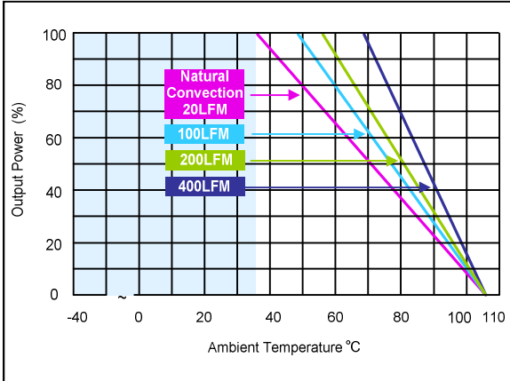
Figure 43: ERM15A110 Derating Curves (without heatsink) Vin = 110Vdc Load: Io = 0 to 15.0A
