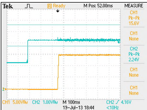
Figure 23: ERM05C72 Output Voltage Startup Characteristic by ON/OFF Vin = 72Vdc Load: Io = 5.0A Ch1: Vo Ch2: Remote On/Off
