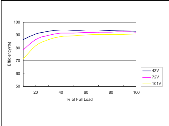
Figure 19: ERM05C72 Efficiency Versus Output Current Curve Vin = 43 to 101Vdc Load: Io = 5.0A
