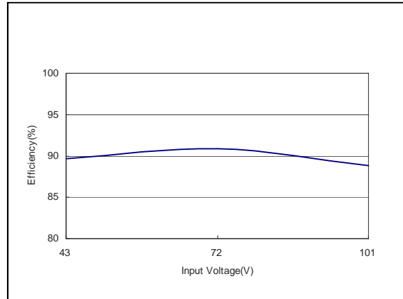
Figure 2: ERM15A72 Efficiency Versus Input Voltage Curve Vin = 43 to 101Vdc Load: Io = 15.0A
