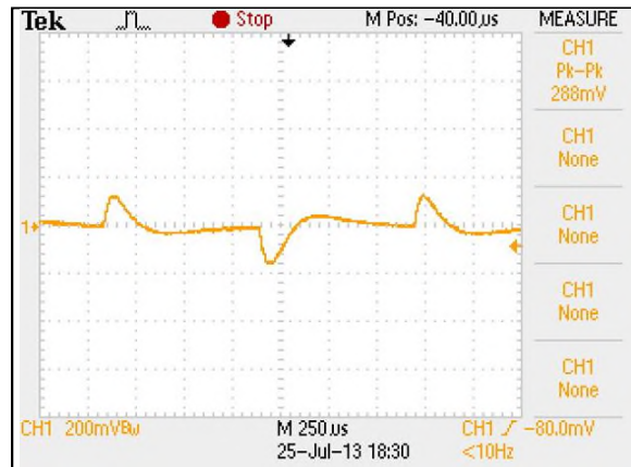
Figure 22: ERM05C72 Transient Response Vin = 72Vdc Load: Io = 100% to 75% load change Ch 1: Vo
