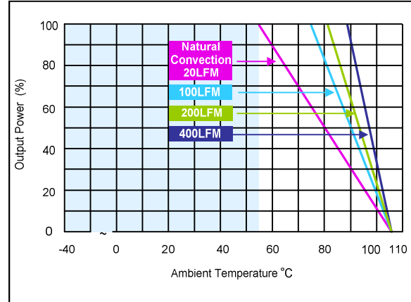
Figure 35: ERM03H72 Derating Curves (with heatsink) Vin = 72Vdc Load: Io = 0 to 3.125A
