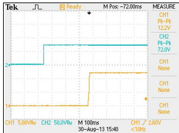
Figure 15: ERM06B72 Output Voltage Startup Characteristic by Vin Vin = 72Vdc Load: Io = 6.25A Ch1: Vo Ch2: Vin
