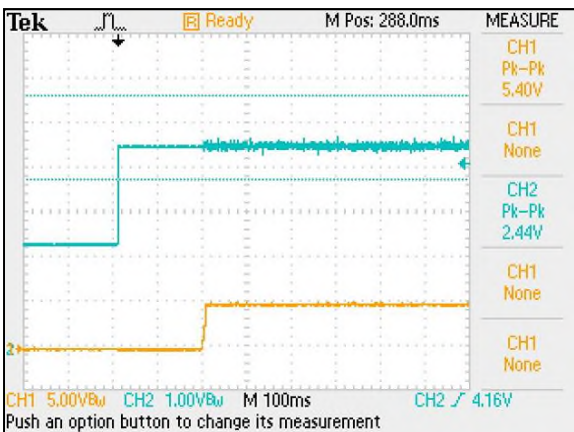
Figure 41: ERM15A110 Output Voltage Startup Characteristic by ON/OFF Vin = 110Vdc Load: Io = 15.0A Ch1: Vo Ch2: Remote On/Off
