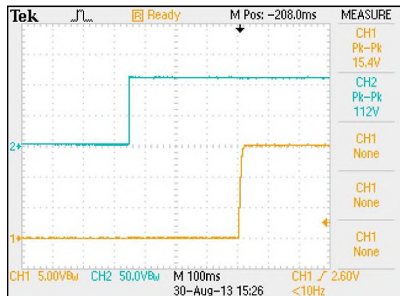
Figure 60: ERM05C110 Output Voltage Startup Characteristic by Vin Vin = 110Vdc Load: Io = 5.0A Ch1: Vo Ch2: Vin
