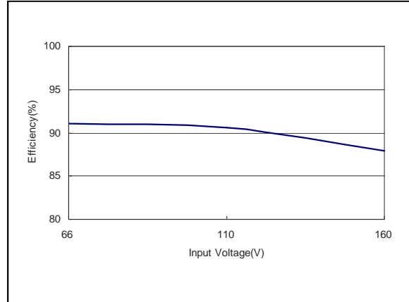
Figure 65: ERM03H110 Efficiency Versus Input Voltage Curve Vin = 66 to 160Vdc Load: Io = 3.125A
