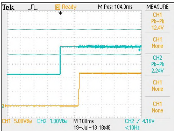
Figure 14: ERM06B72 Output Voltage Startup Characteristic by ON/OFF Vin = 72Vdc Load: Io = 6.25A Ch1: Vo Ch2: Remote On/Off
