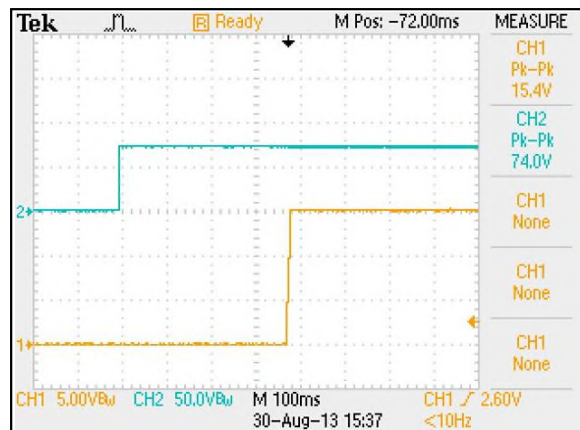
Figure 24: ERM05C72 Output Voltage Startup Characteristic by Vin Vin = 72Vdc Load: Io = 15.0A Ch1: Vo Ch2: Vin
