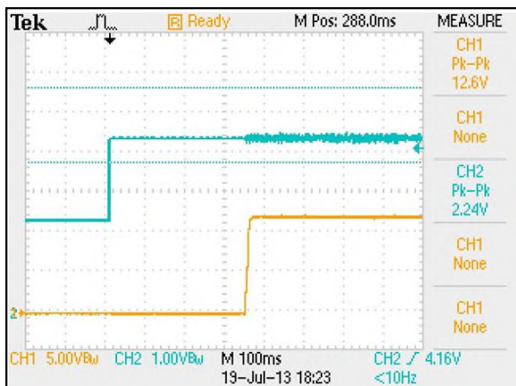
Figure 50: ERM06B110 Output Voltage Startup Characteristic by ON/OFF Vin = 110Vdc Load: Io = 6.25A Ch1: Vo Ch2: Remote On/Off
