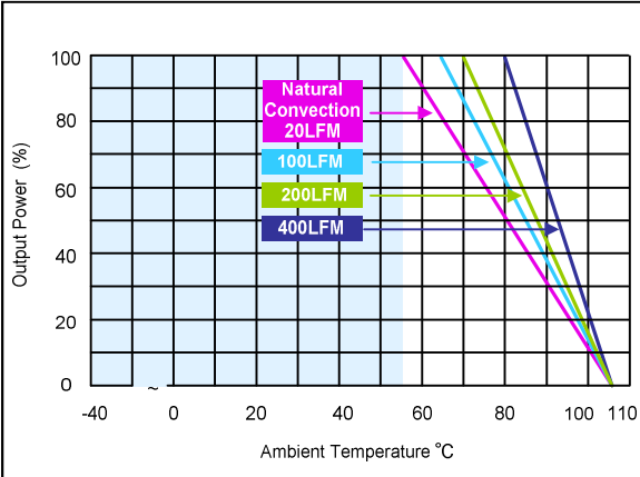
Figure 16: ERM06B72 Derating Curves (without heatsink) Vin = 72Vdc Load: Io = 0 to 6.25A
