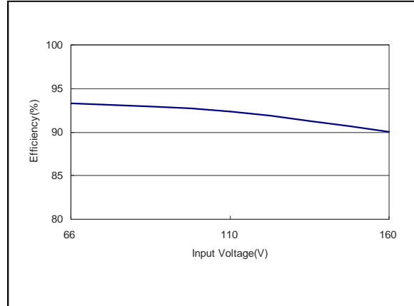
Figure 56: ERM05C110 Efficiency Versus Input Voltage Curve Vin = 66 to 160Vdc Load: Io = 5.0A
