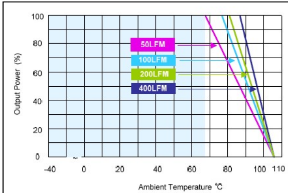
Figure 70: AXA04F36-L Derating Curves (without heatsink) Vin = 48Vdc Load: Io = 0 to 4.5A
