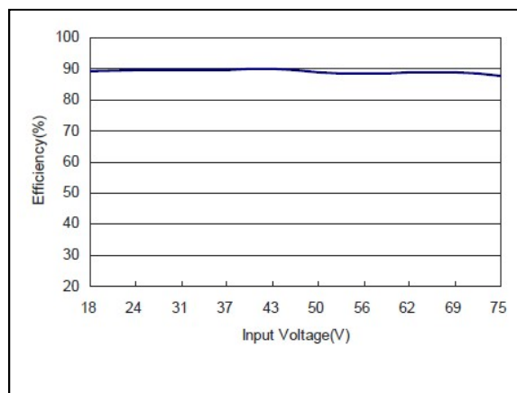
Figure 83: AXA01B36-L Efficiency Versus Input Voltage Curve Vin = 18-75 Vdc Load: Io = 1.67A
