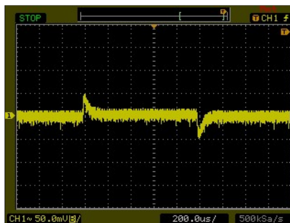
Figure 76: AXA04A36-L Transient Response Vin = 48Vdc Load: Io = 100% to 75% load change Ch 1: Vo
