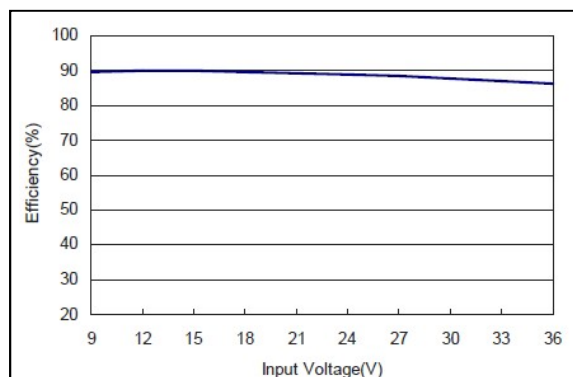
Figure 2: AXA04F18-L Efficiency Versus Input Voltage Curve Vin = 9 to 36Vdc Load: Io = 4.5A
