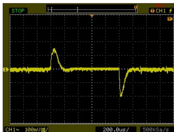
Figure 85: AXA01B36-L Transient Response Vin = 48Vdc Load: Io = 100% to 75% load change Ch 1: Vo
