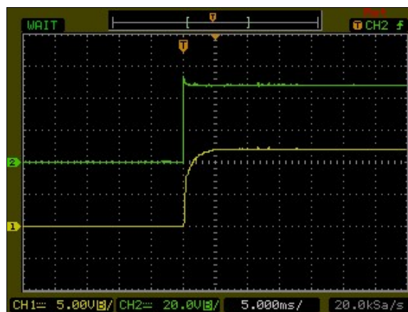
Figure 87: AXA01B36-L Output Voltage Startup Characteristic by Vin Vin = 48Vdc Load: Io = 1.67A Ch1: Vo Ch2: Vin
