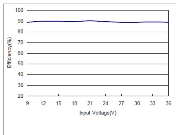
Figure 47: AXA00BB18-L Efficiency Versus Input Voltage Curve Vin = 9 to 36Vdc Load: I_o = \pm 0.835 A
