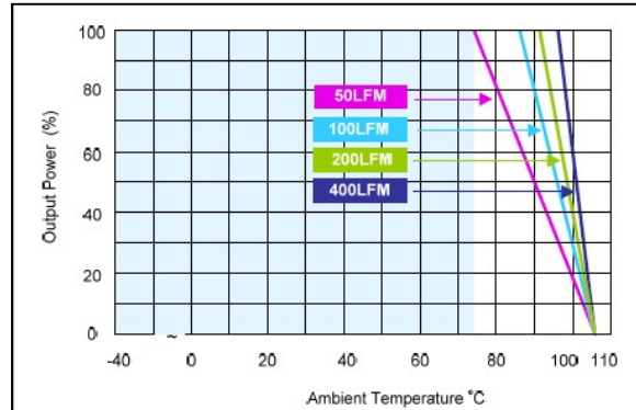
Figure 71: AXA04F36-L Derating Curves (with heatsink) Vin = 48Vdc Load: Io = 4.5A
