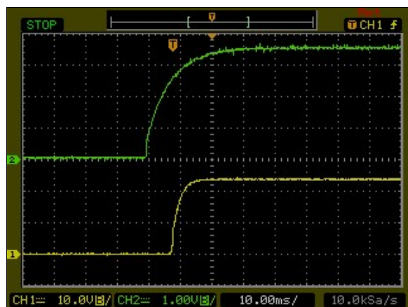
Figure 41: AXA00H18-L Output Voltage Startup Characteristic by ON/OFF Vin = 24Vdc Load: Io = 0.835A Ch1: Vo Ch2: Remote On/Off
