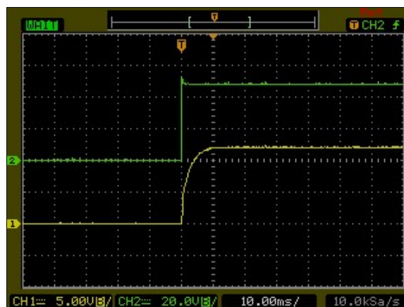
Figure 104: AXA00BB36-L Output Voltage Startup Characteristic by Vin Vin = 48Vdc Load: Io = ±0.835 A Ch1: Vo Ch2: Vin
