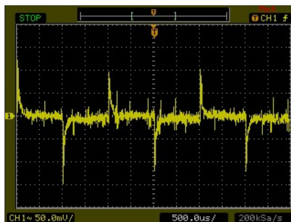
Figure 40: AXA00H18-L Transient Response Vin = 24Vdc Load: Io = 100% to 75% load change Ch 1: Vo
