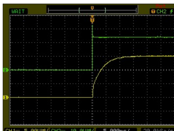
Figure 60: AXA00CC18-L Output Voltage Startup Characteristic by Vin Vin = 24Vdc Load: Io = \pm 0.67 A Ch1: Vo Ch2: Vin
