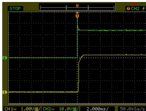
Figure 6: AXA04F18-L Output Voltage Startup Characteristic by Vin Vin = 24Vdc Load: Io = 4.5A Ch1: Vo Ch2: Vin
