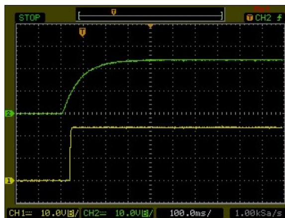
Figure 42: AXA00H18-L Output Voltage Startup Characteristic by Vin Vin = 24Vdc Load: Io = 0.835A Ch1: Vo Ch2: Vin
