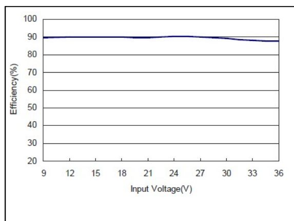
Figure 56: AXA00CC18-L Efficiency Versus Input Voltage Curve Vin = 9 to 36Vdc Load: Io = \pm 0.67 A
