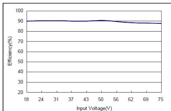
Figure 110: AXA00BB36-L Efficiency Versus Input Voltage Curve Vin = 18-75 Vdc Load: Io = ±0.835 A
