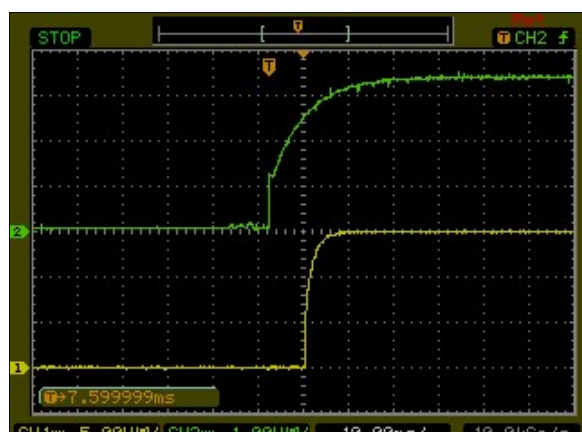
Figure 32: AXA01C18-L Output Voltage Startup Characteristic by ON/OFF Vin = 24Vdc Load: Io = 1.33A Ch1: Vo Ch2: Remote On/Off
