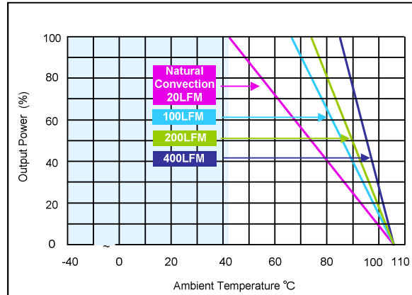
Figure 8: AXA04F18-L Derating Curves (with heatsink) Vin = 24Vdc Load: Io = 0 to 4.5A
