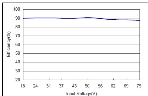
Figure 110: AXA00BB36-L Efficiency Versus Input Voltage Curve Vin = 18-75 Vdc Load: Io = \pm 0.835 A
