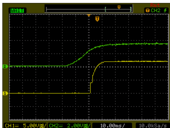
Figure 50: AXA00BB18-L Output Voltage Startup Characteristic by ON/OFF Vin = 24Vdc Load: I_o = \pm 0.835 A Ch1: Vo Ch2: Remote On/Off
