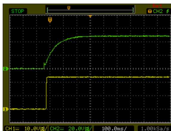
Figure 105: AXA00H36-L Output Voltage Startup Characteristic by Vin Vin = 48Vdc Load: Io = 0.835A Ch1: Vo Ch2: Vin
