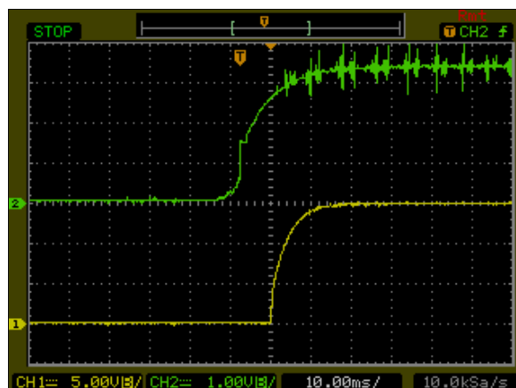
Figure 112: AXA00CC36-L Output Voltage Startup Characteristic by ON/OFF Vin = 48Vdc Load: Io = \pm 0.67 A Ch1: Vo Ch2: Remote On/Off
