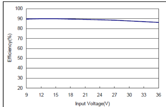
Figure 2: AXA04F18-L Efficiency Versus Input Voltage Curve Vin = 9 to 36Vdc Load: Io = 4.5A
