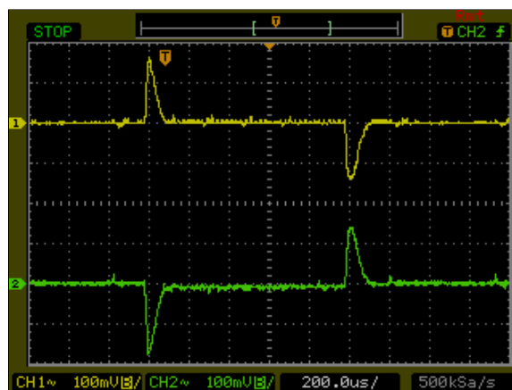
Figure 58: AXA00CC18-L Transient Response Vin = 24Vdc Load: Io = 100% to 75% load change Ch 1: Vo1 Ch 2: Vo2
