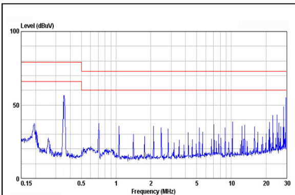
Figure 9: AXA04F18-L Conduction Emission of EN550122 Class A Vin = 24Vdc Load: Io = 4.5A
