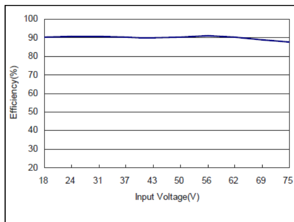
Figure 109: AXA00CC36-L Efficiency Versus Input Voltage Curve Vin = 18-75 Vdc Load: Io = \pm 0.67 A
