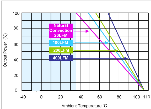
Figure 7: AXA04F18-L Derating Curves (without heatsink) Vin = 24Vdc Load: Io = 0 to 4.5A
