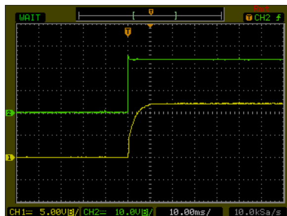
Figure 51: AXA00BB18-L Output Voltage Startup Characteristic by Vin Vin = 24Vdc Load: I_o = \pm 0.835 A Ch1: Vo Ch2: Vin
