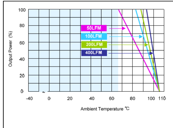
Figure 62: AXA00CC18-L Derating Curves (with heatsink) Vin = 24Vdc Load: Io = 0 to ±0.67 A
