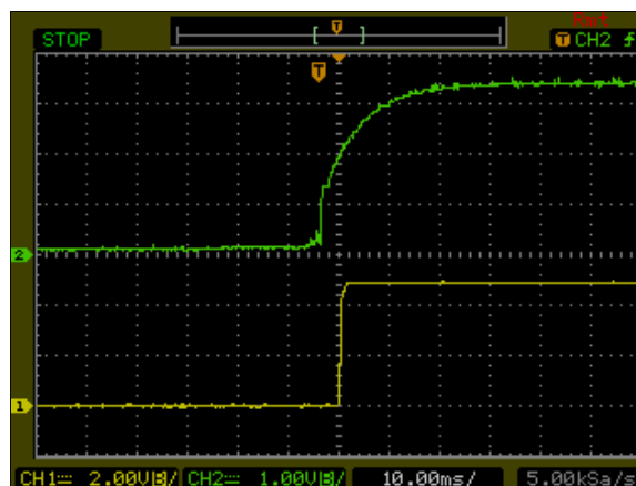
Figure 15: AXA04A18-L Output Voltage Startup Characteristic by Vin Vin = 24Vdc Load: Io = 4A Ch1: Vo Ch2: Vin
