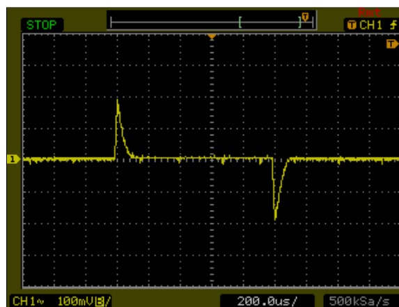
Figure 94: AXA01B36-L Transient Response Vin = 48Vdc Load: Io = 100% to 75% load change Ch 1: Vo
