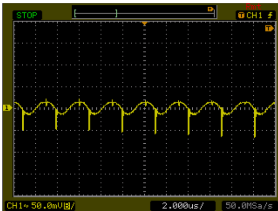
Figure 21: AXA01B18-L Ripple and Noise Measurement Vin = 24Vdc Load: Io = 1.67A Ch 1: Vo
