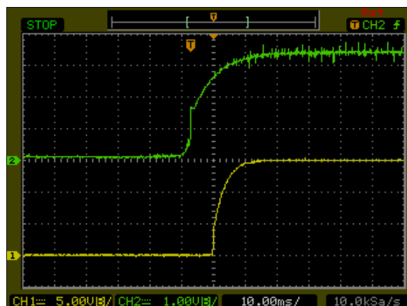
Figure 59: AXA00CC18-L Output Voltage Startup Characteristic by ON/OFF Vin = 24Vdc Load: Io = \pm 0.67 A Ch1: Vo Ch2: Remote On/Off
