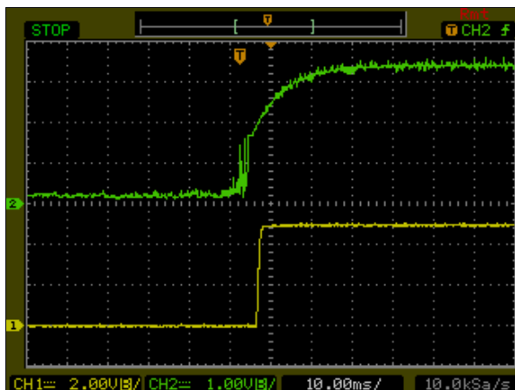
Figure 77: AXA04A36-L Output Voltage Startup Characteristic by ON/OFF Vin = 48Vdc Load: Io = 4A Ch1: Vo Ch2: Remote On/Off
