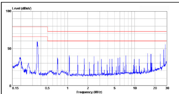
Conduction Emission of EN55022 Class A V_{in} = V_{in, nom} ; Full Load
