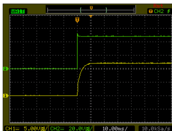
Figure 104: AXA00BB36-L Output Voltage Startup Characteristic by Vin Vin = 48Vdc Load: Io = \pm 0.835 A Ch1: Vo Ch2: Vin
