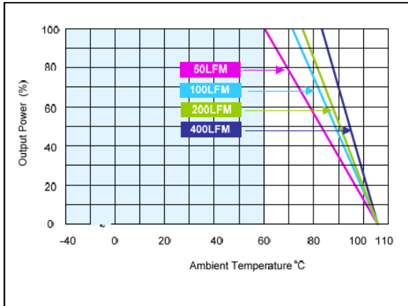
Figure 61: AXA00CC18-L Derating Curves (without heatsink) Vin = 24Vdc Load: Io = 0 to ±0.67 A
