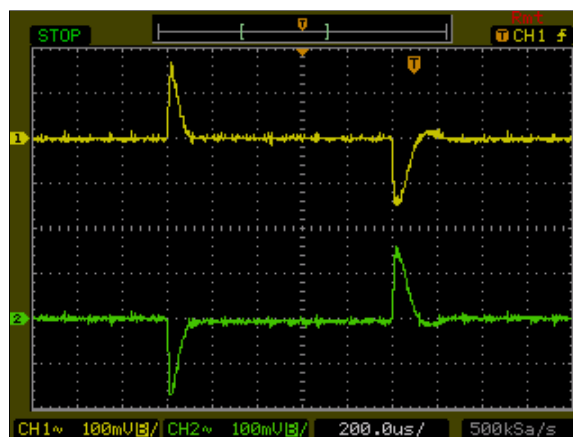
Figure 102: AXA00BB36-L Transient Response Vin = 48Vdc Load: Io = 100% to 75% load change Ch 1: Vo1 Ch2:Vo2
