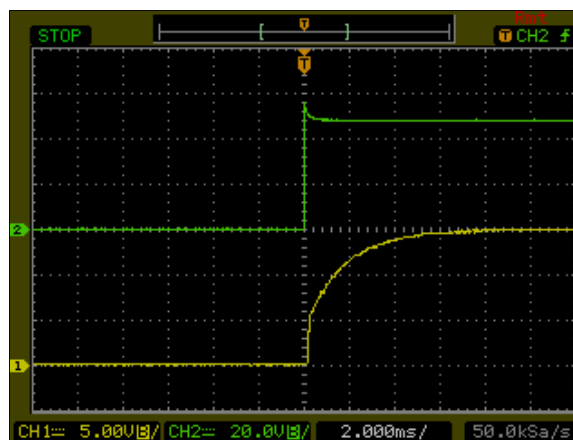
Figure 96: AXA01B36-L Output Voltage Startup Characteristic by Vin Vin = 48Vdc Load: Io = 1.33A Ch1: Vo Ch2: Vin
