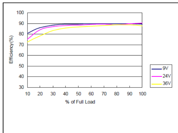
Figure 55: AXA00CC18-L Efficiency Versus Output Current Curve Vin = 9 to 36Vdc Load: Io = 0 to \pm 0.67 A
