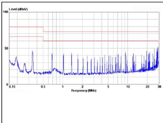
Figure 63: AXA00CC18-L Conduction Emission of EN550122 Class A Vin = 24Vdc Load: Io = ±0.67 A
