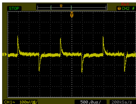
Figure 103: AXA00H36-L Transient Response Vin = 48Vdc Load: Io = 100% to 75% load change Ch 1: Vo
