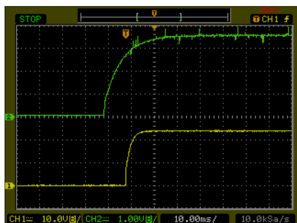
Figure 104: AXA00H36-L Output Voltage Startup Characteristic by ON/OFF Vin = 48Vdc Load: Io = 0.835A Ch1: Vo Ch2: Remote On/Off
