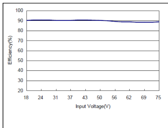
Figure 92: AXA01B36-L Efficiency Versus Input Voltage Curve Vin = 18-75 Vdc Load: Io = 1.33A
