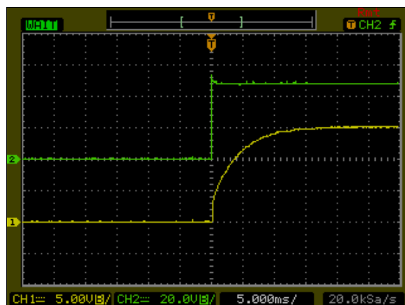
Figure 113: AXA00CC36-L Output Voltage Startup Characteristic by Vin Vin = 48Vdc Load: Io = \pm 0.67 A Ch1: Vo Ch2: Vin
