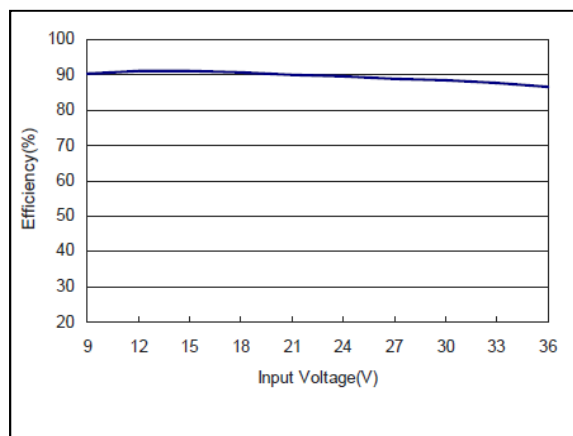
Figure 11: AXA04A18-L Efficiency Versus Input Voltage Curve Vin = 9 to 36Vdc Load: Io = 4A
