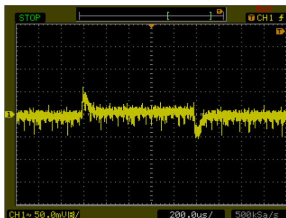
Figure 13: AXA04A18-L Transient Response Vin = 24Vdc Load: Io = 100% to 75% load change Ch 1: Vo
