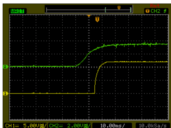
Figure 103: AXA00BB36-L Output Voltage Startup Characteristic by ON/OFF Vin = 48Vdc Load: Io = \pm 0.835 A Ch1: Vo Ch2: Remote On/Off
