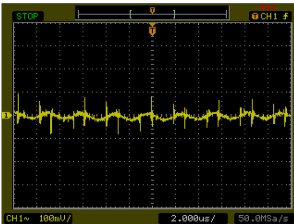
Figure 39: AXA00H18-L Ripple and Noise Measurement Vin = 24Vdc Load: Io = 0.835A Ch 1: Vo
