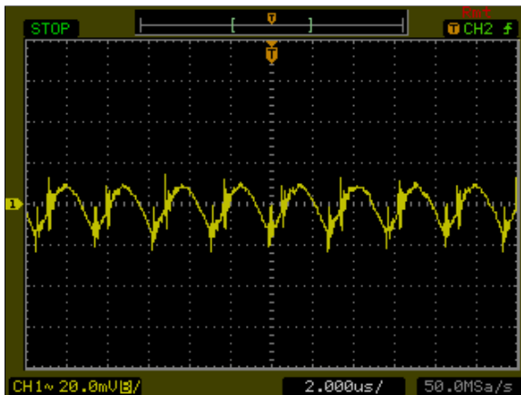
Figure 66: AXA04F36-L Ripple and Noise Measurement Vin = 48Vdc Load: Io = 4.5A Ch 1: Vo
