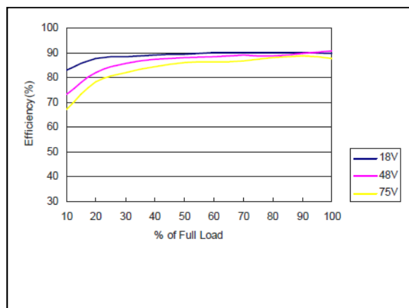
Figure 109: AXA00BB36-L Efficiency Versus Output Current Curve Vin = 18 to 75Vdc Load: Io = 0 to \pm 0.835 A
