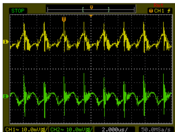
Figure 111 : AXA00BB36-L Ripple and Noise Measurement Vin = 48Vdc Load: Io = \pm 0.835 A Ch 1: Vo1 Ch2:Vo2
