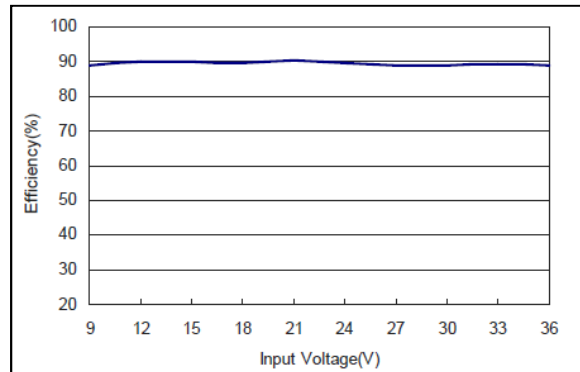
Figure 47: AXA00BB18-L Efficiency Versus Input Voltage Curve Vin = 9 to 36Vdc Load: I_o = \pm 0.835 A
