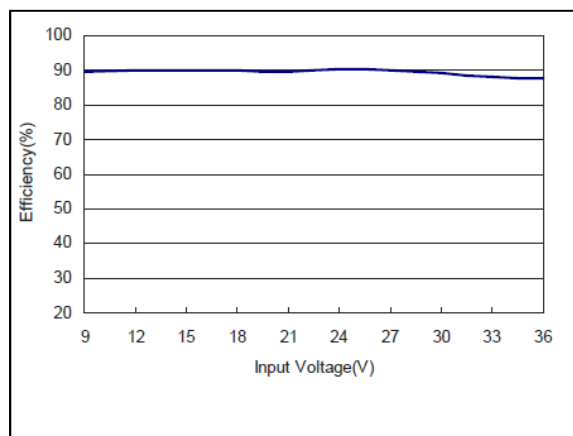
Figure 56: AXA00CC18-L Efficiency Versus Input Voltage Curve Vin = 9 to 36Vdc Load: Io = \pm 0.67 A
