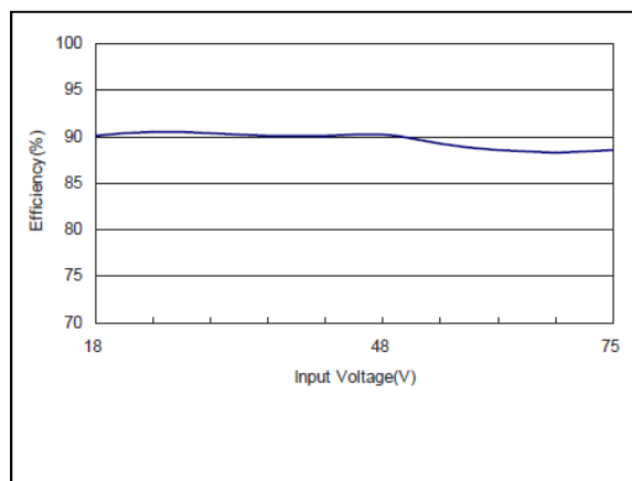
Figure 101: AXA00H36-L Efficiency Versus Input Voltage Curve Vin = 18-75 Vdc Load: Io = 0.835A
