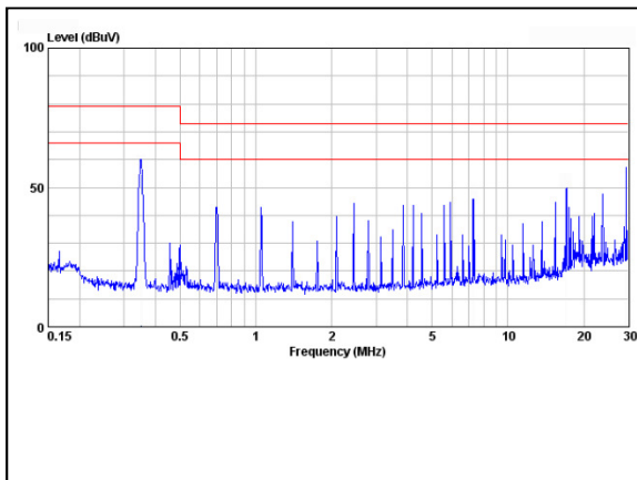
Figure 81: AXA04A36-L Conduction Emission of EN550122 Class A Vin = 48Vdc Load: Io = 4A
