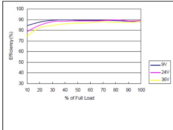
Figure 46: AXA00BB18-L Efficiency Versus Output Current Curve Vin = 9 to 36Vdc Load: I_o = 0 to \pm 0.835 A
