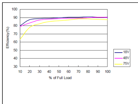
Figure 108: AXA00CC36-L Efficiency Versus Output Current Curve Vin = 18 to 75Vdc Load: Io = 0 to \pm 0.67 A
