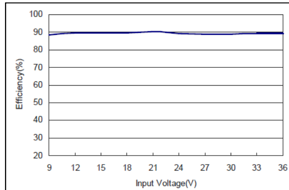
Figure 20: AXA01B18-L Efficiency Versus Input Voltage Curve Vin = 9 to 36Vdc Load: Io = 1.67A
