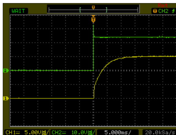
Figure 60: AXA00CC18-L Output Voltage Startup Characteristic by Vin Vin = 24Vdc Load: Io = \pm 0.67 A Ch1: Vo Ch2: Vin
