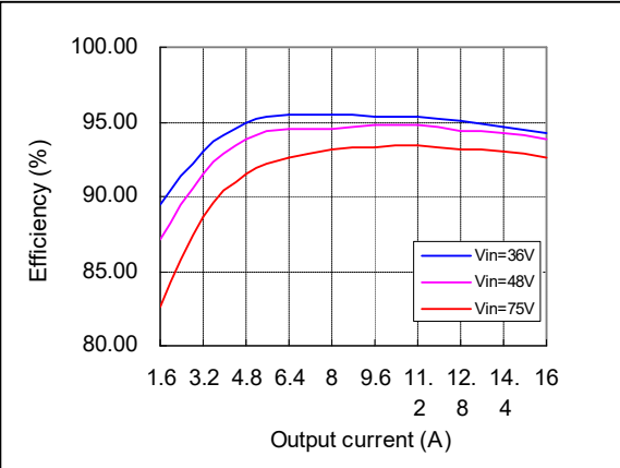
Figure 8: AVE450B-48S28 Efficiency Curves @ 25 °C
