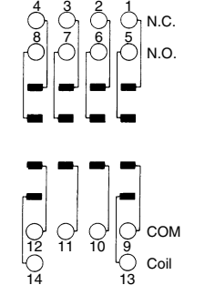
Schematic
