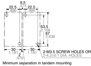
Chassis cutout
