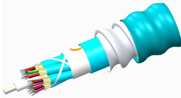
LazrSPEED® Riser Distribution Cable, interlocking aluminum armored with riser jacket, 4 fiber single-unit
